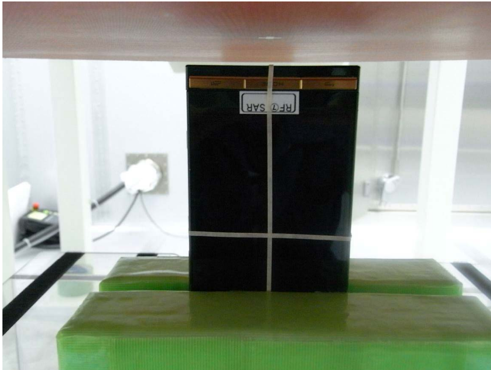
Test setup photo (Bottom)
