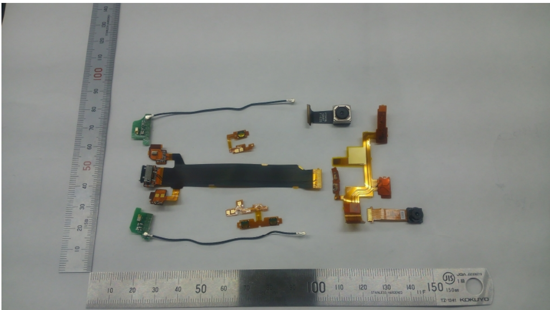
Sub FPC
