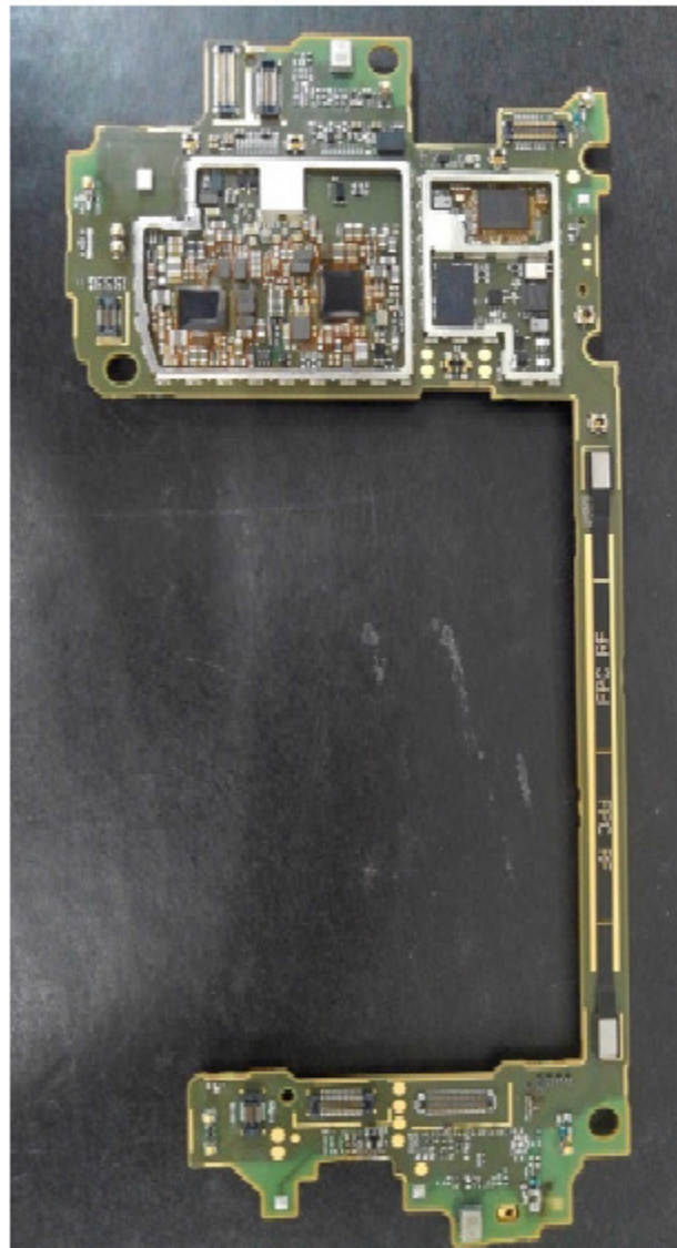
Main PCB rear
