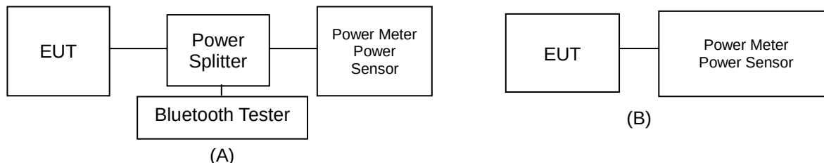
Figure 10.3 Average Power Measurement Setup
