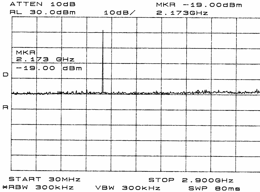
Figure four Spurious Emissions at Antenna Terminal.
