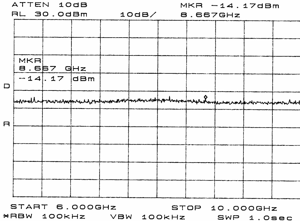
Figure six Spurious Emissions at Antenna Terminal.
