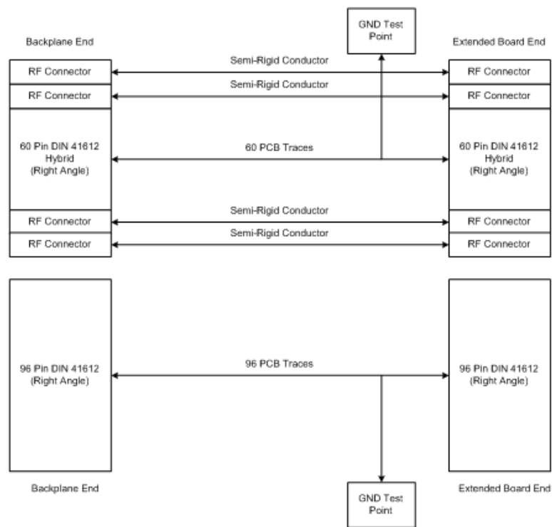
Figure 1-21 Extender Board
