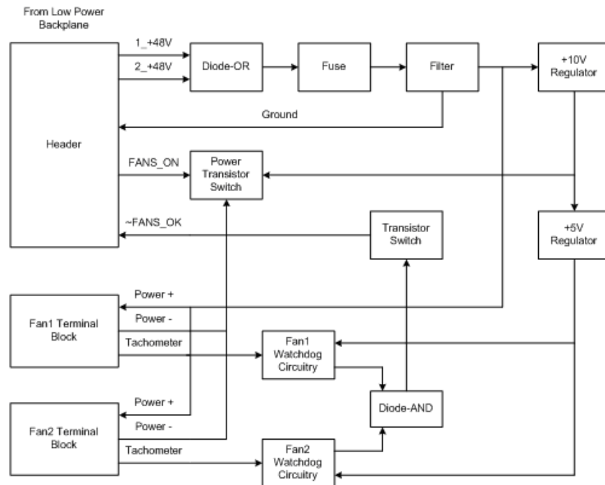
Figure 1-19 Fan Control CCA Block Diagram
