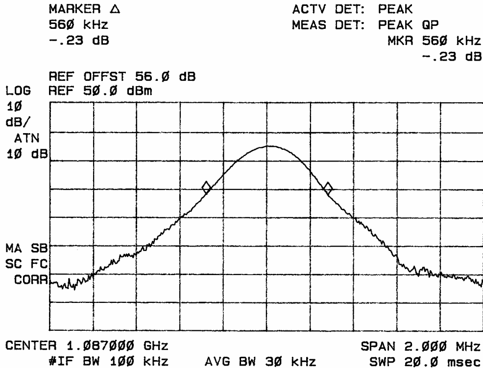
Figure two Occupied Band Width
