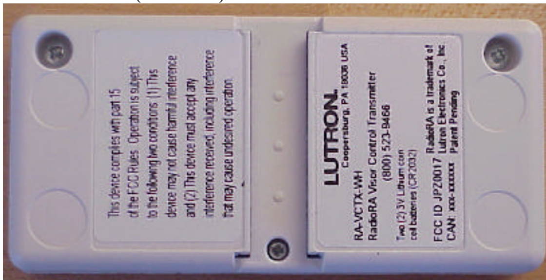
External Transmitter (Bottom Side)
