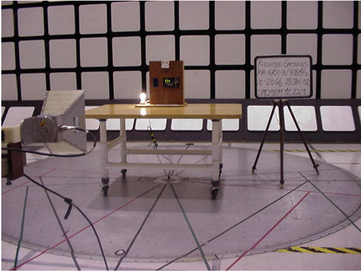
Radiated emissions test 1 - 2GHz set-up
