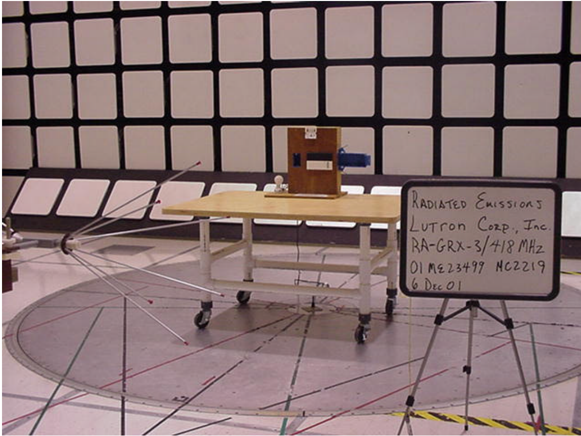
Radiated emissions test 30 - 1000MHz set-up
