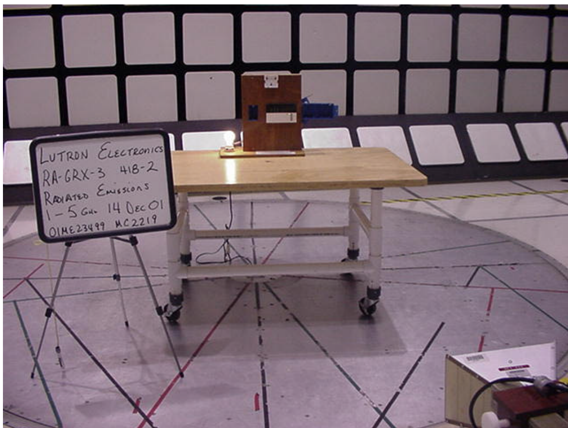
Radiated Emissions test 1 - 5GHz set-up
