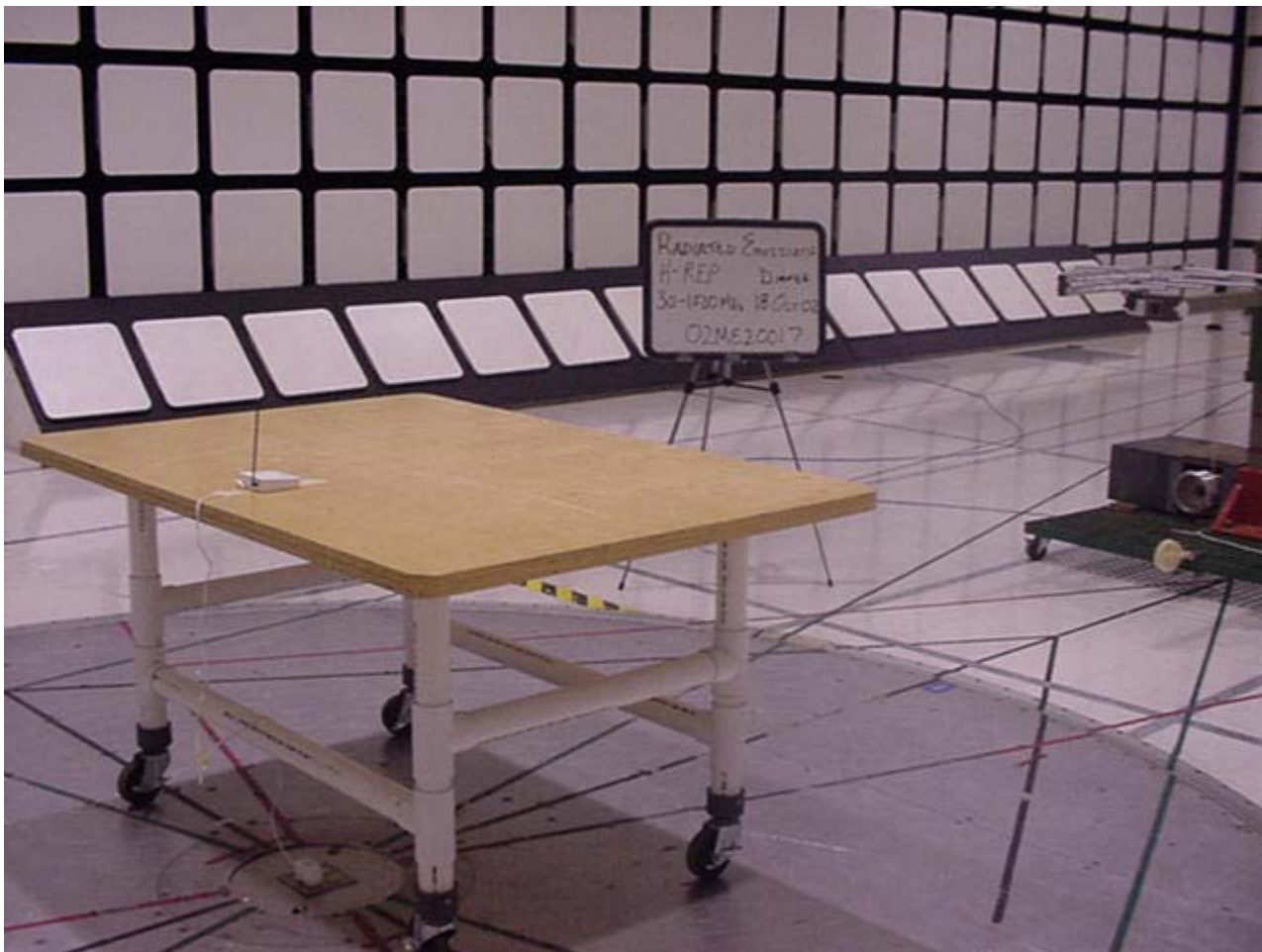
Radiated Emission Test Set-Up 30-1000MHz Rear View
