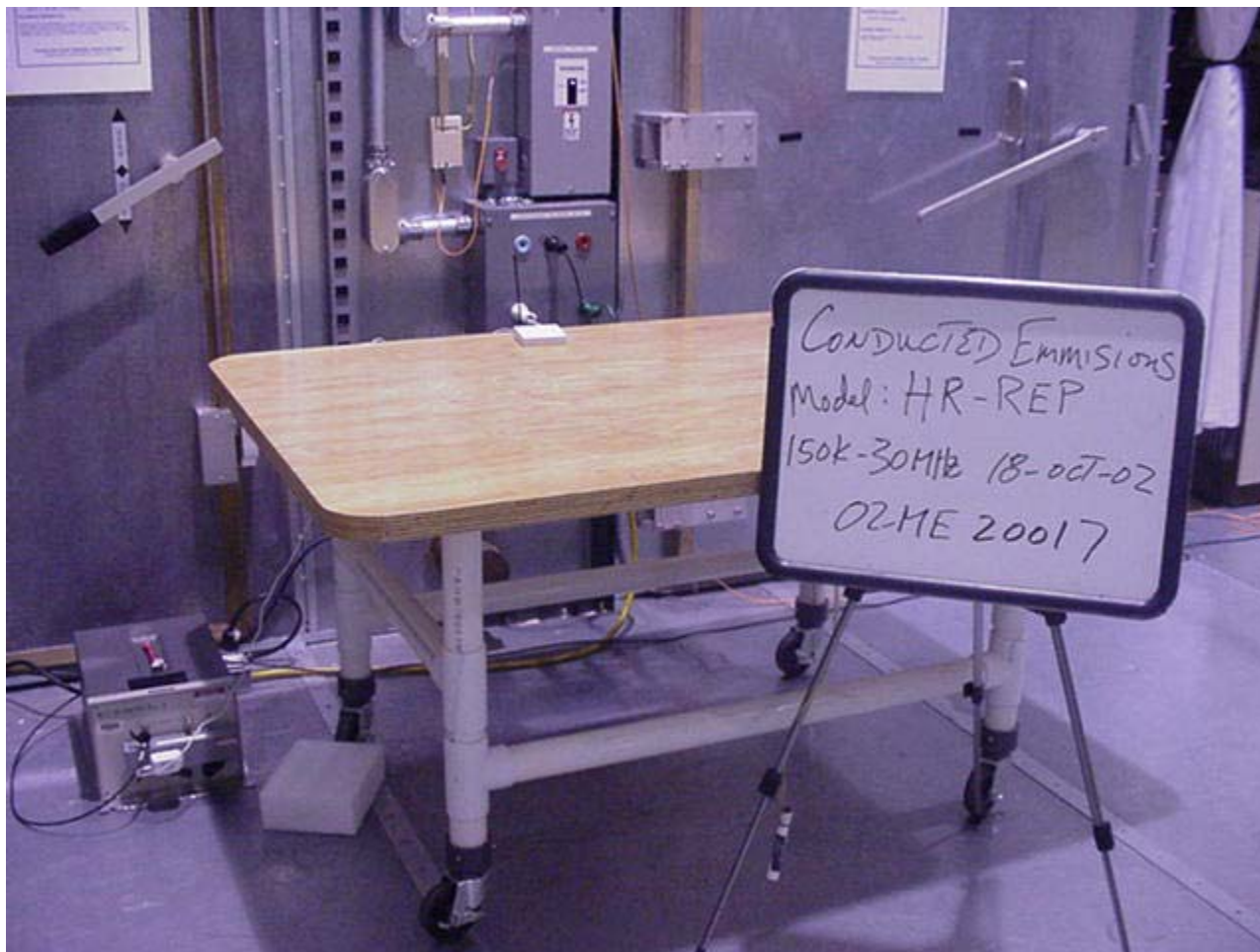
Conducted Emissions Test Set-Up 150k-30MHz
