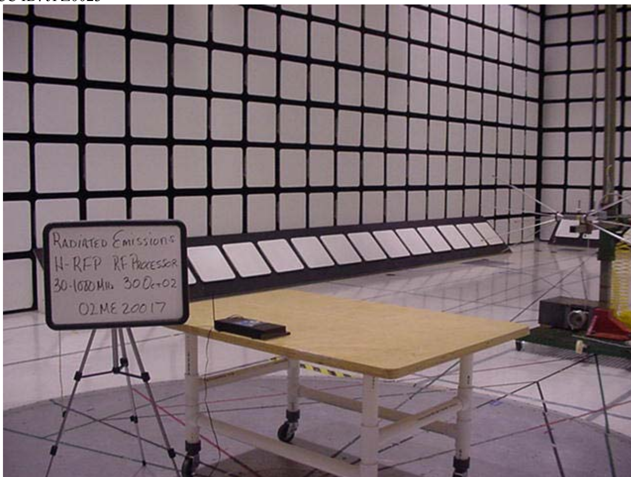
Radiated Emissions Test Set-Up 30-1000MHz Rear View
