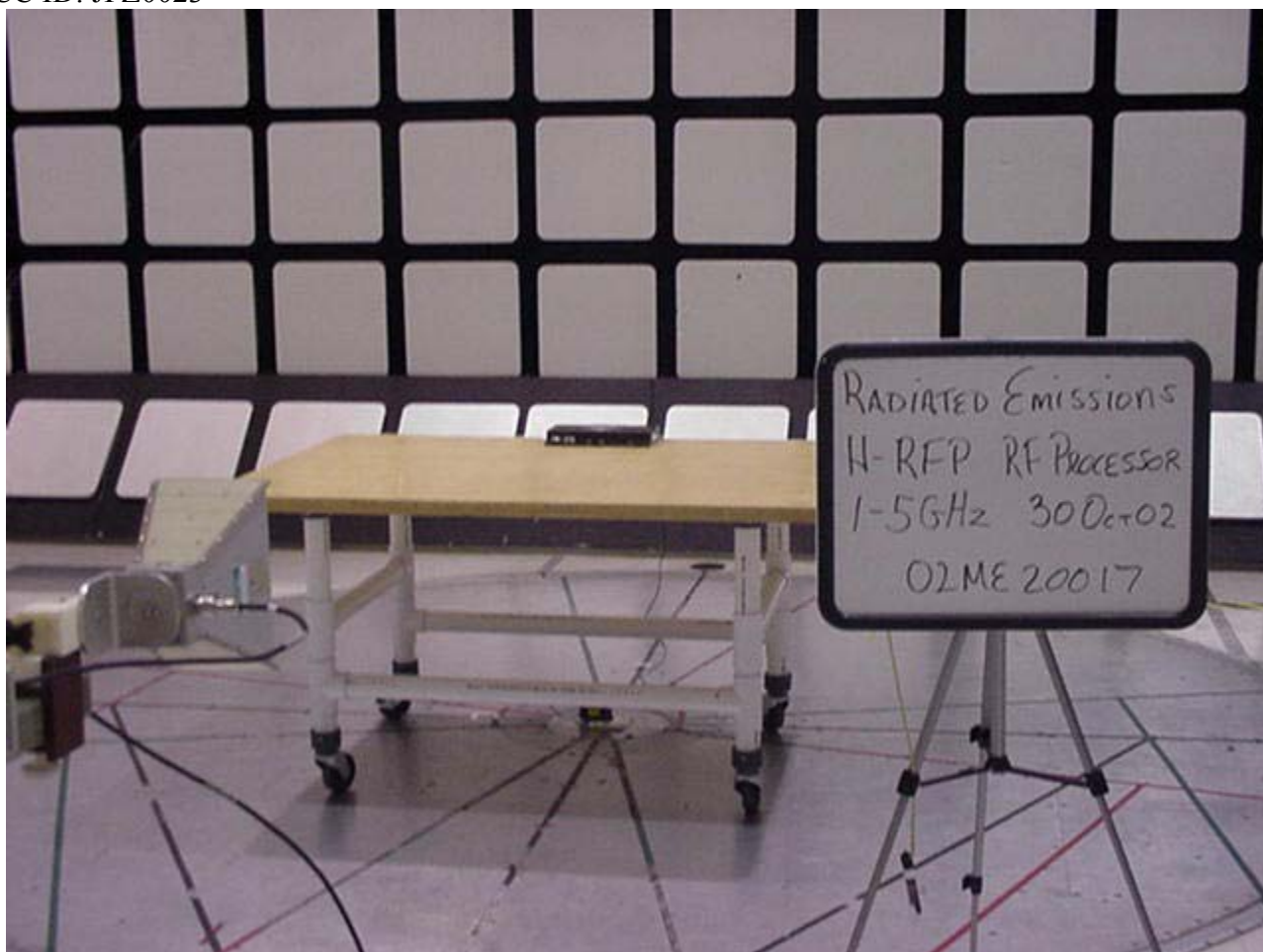
Radiated Emissions Test Set-Up 1-5GHz Front View
