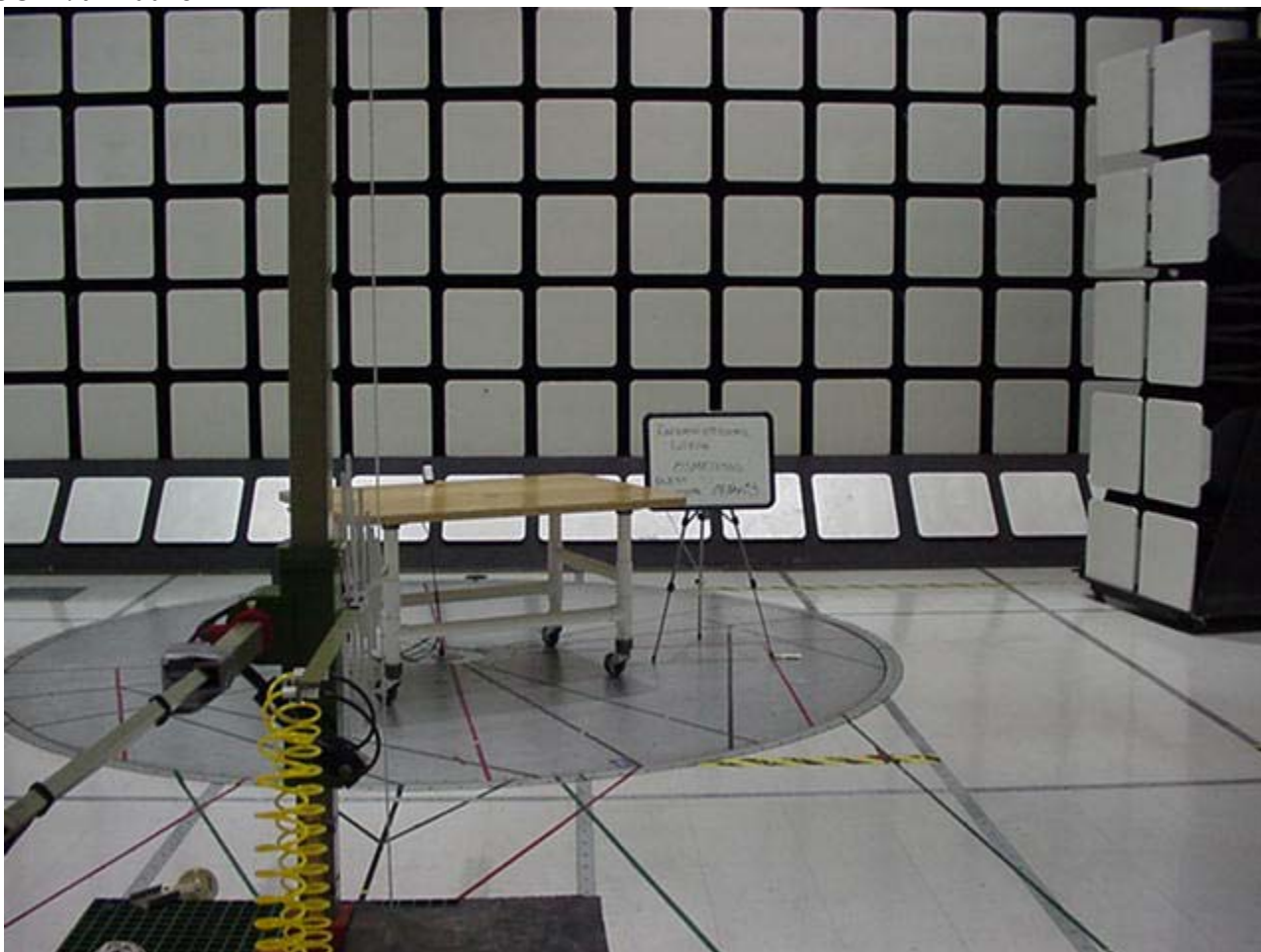
Radiated Emission Test Set-Up 200 to 1000 MHz Front View
