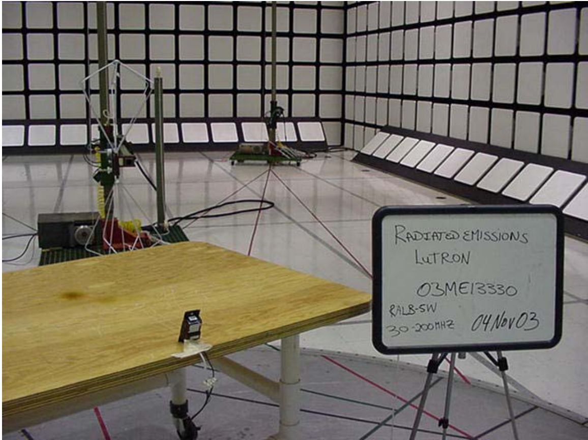
Radiated Emission Test Set-Up 30-200 MHz Rear View
