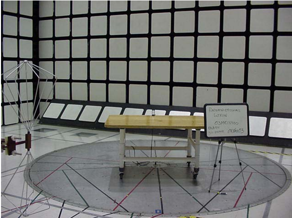
Radiated Emission Test Set-Up 30-200 MHz Front View
