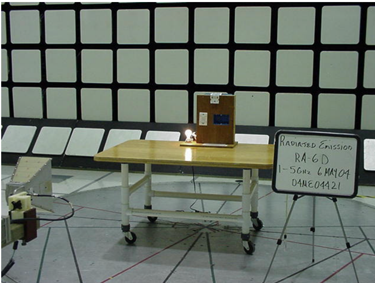
Radiated Emission Test Set-up Front View 1 -5GHz
