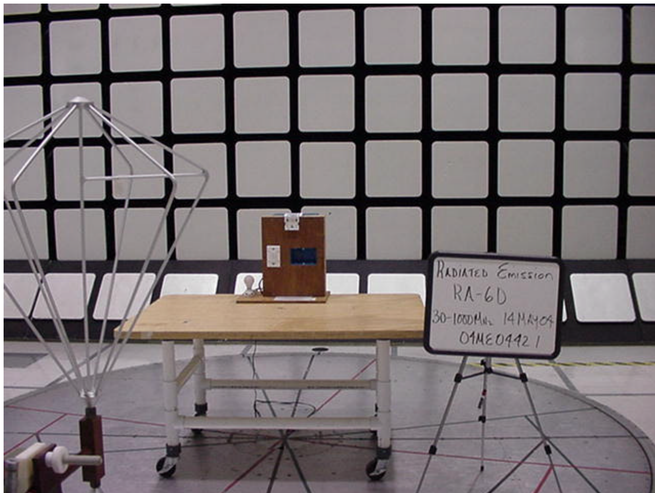
Radiated Emission Test Set-up Front View 30 –1000MHz
