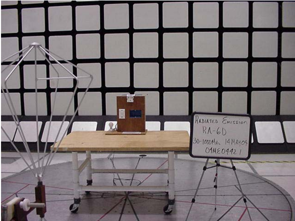
Radiated Emission Test Set-up Front View 30 –1000MHz
