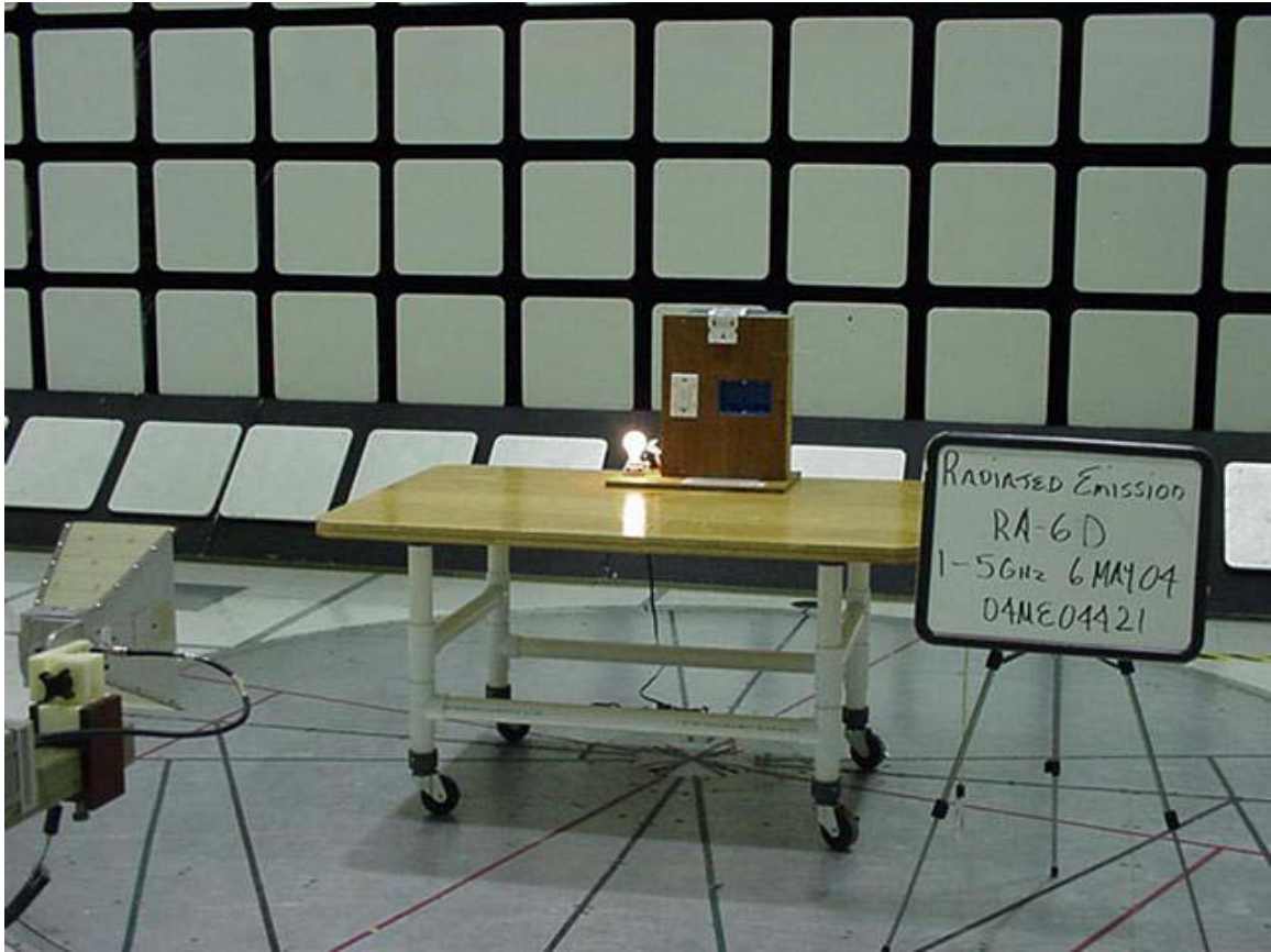
Radiated Emission Test Set-up Front View 1 -5GHz
