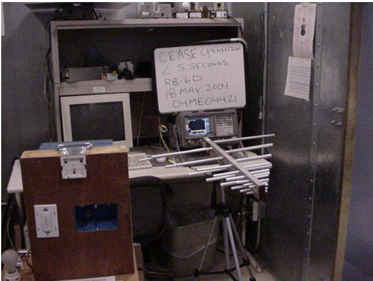
Cease Operation Test Set-Up
