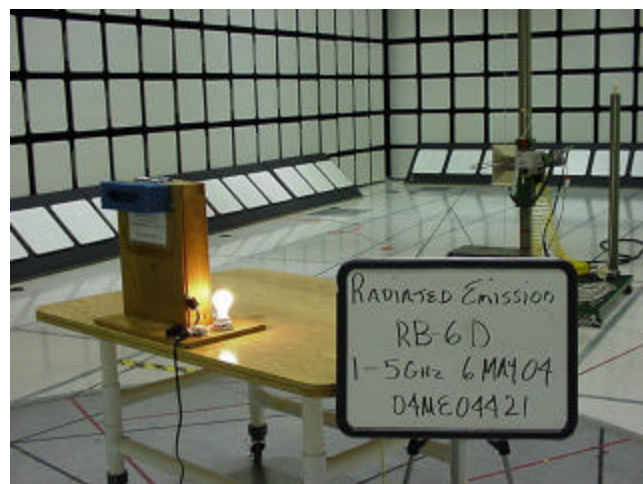
Rear – 1-5GHz
