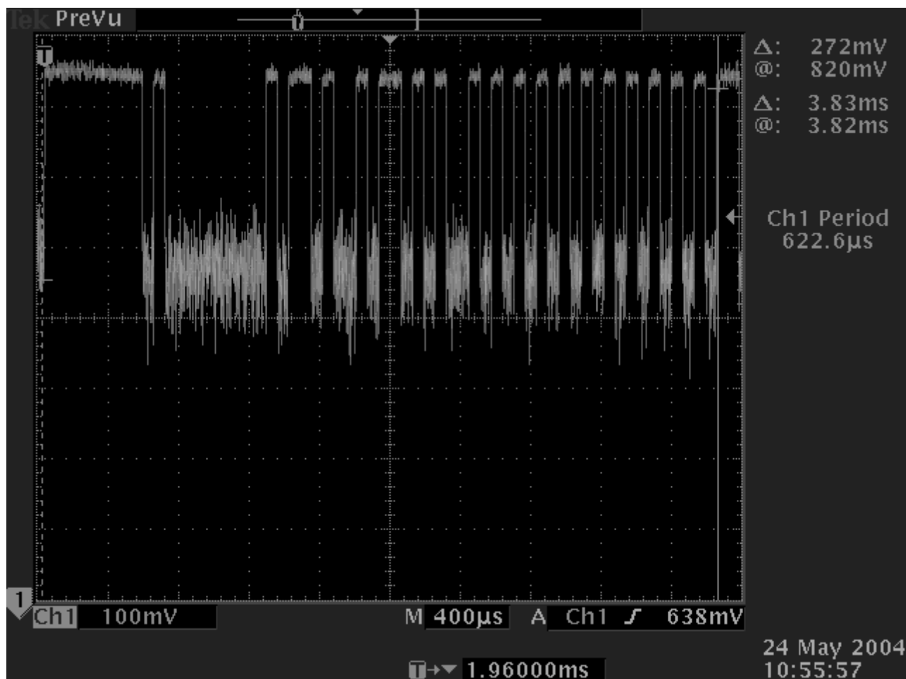
Pulse Train T0 – T1
