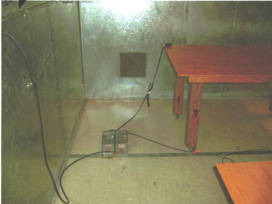
EUT 80cm From LISN
