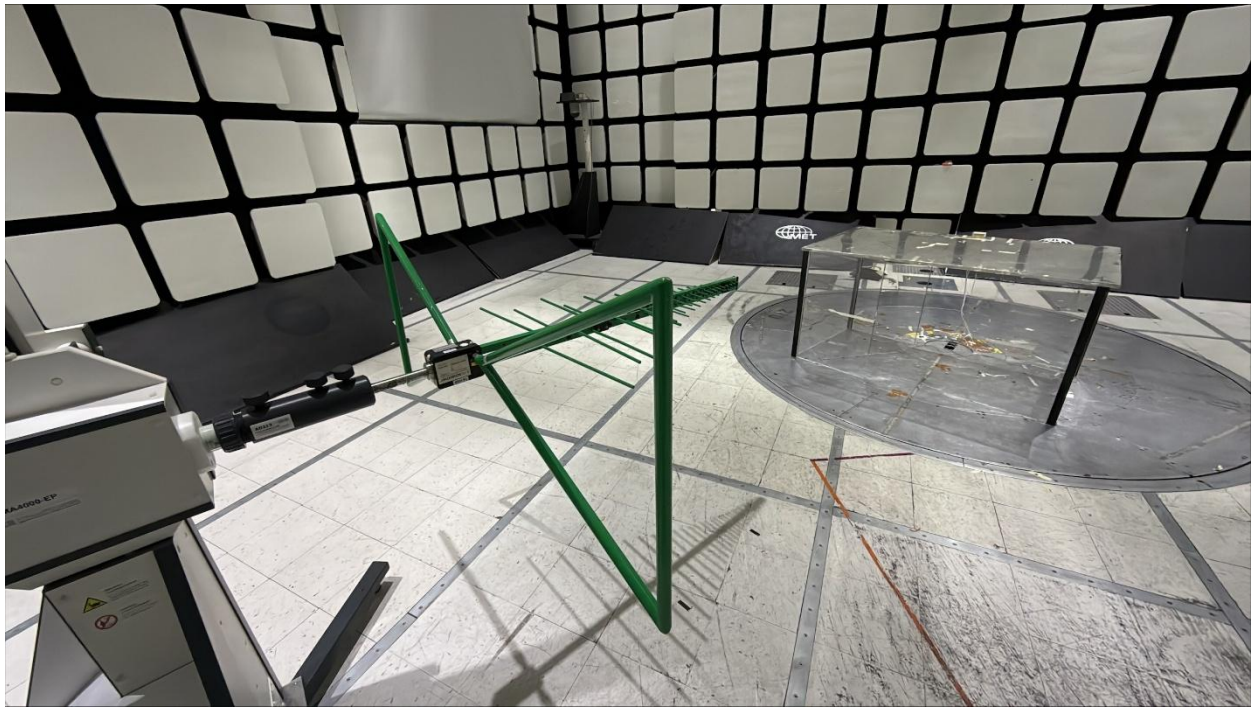
Radiated Emissions 30MHz – 1GHz (Antenna View)
