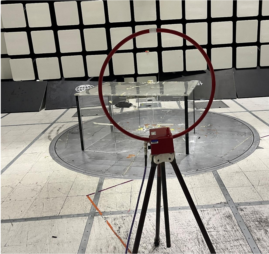
Radiated Emissions Below 30MHz (Antenna View)
