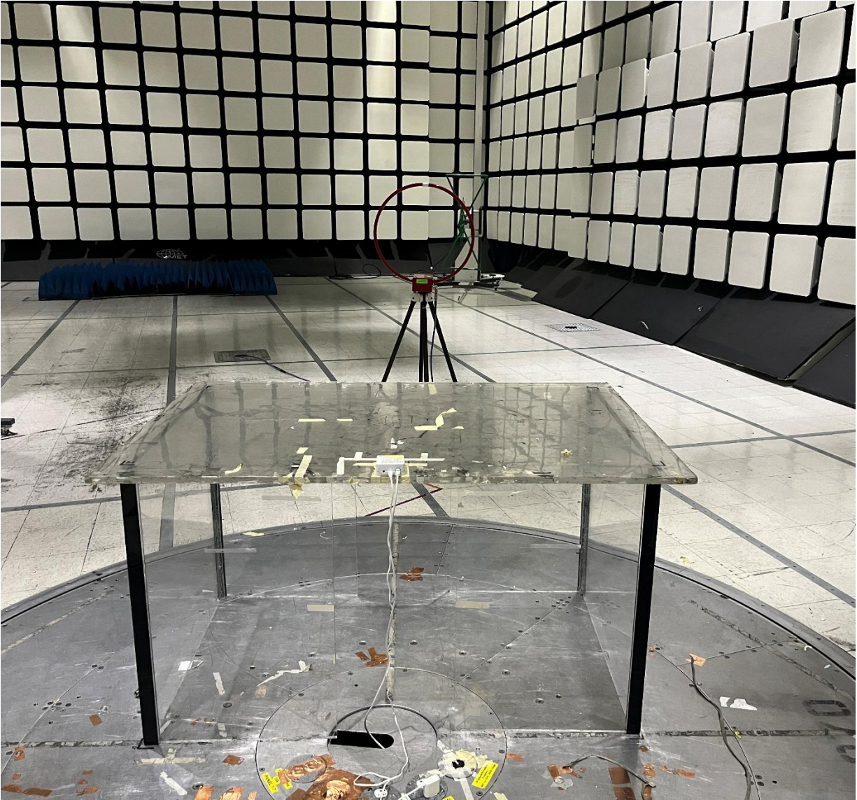
Radiated Emissions Below 30MHz (Back Side)
