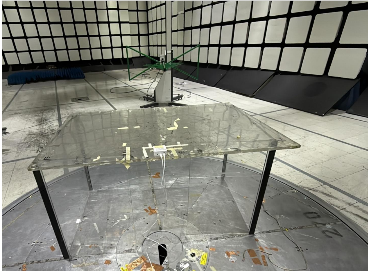
Radiated Emissions 30MHz – 1GHz (Back Side)
