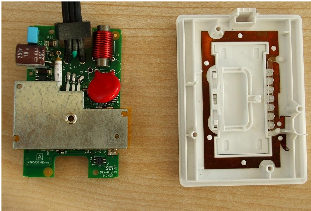
PD-APS PWB removed to show antenna
