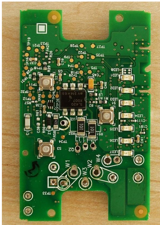
PD-APS PWB Front
