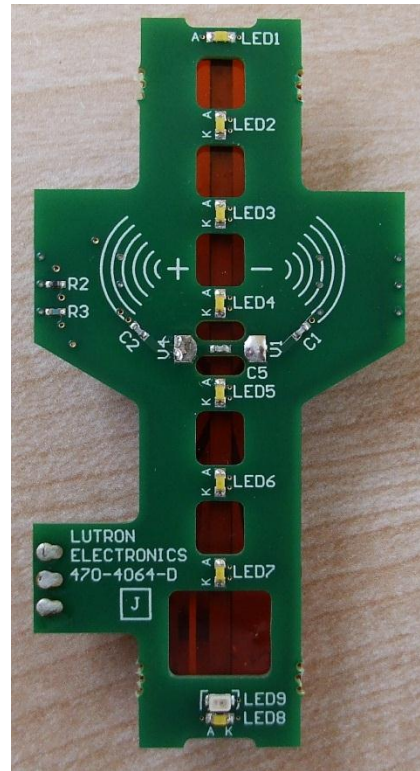
GT-RF Front Board (front)
