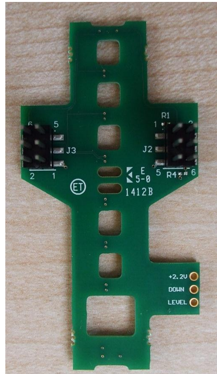
GT-RF Front Board with Flex potentiometer removed
