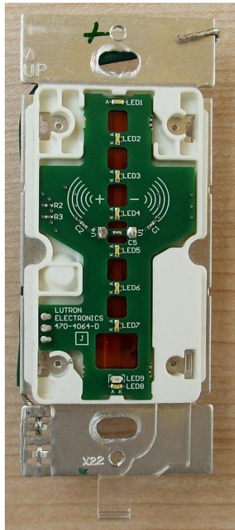
GT-RF with Antenna removed
