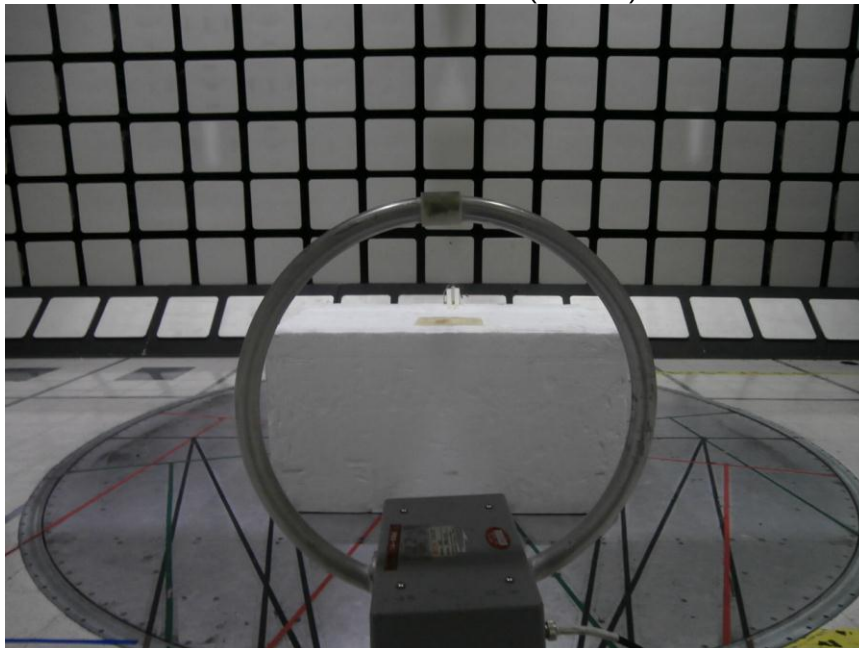
RADIATED EMISSIONS BELOW 1000MHz (FRONT)
