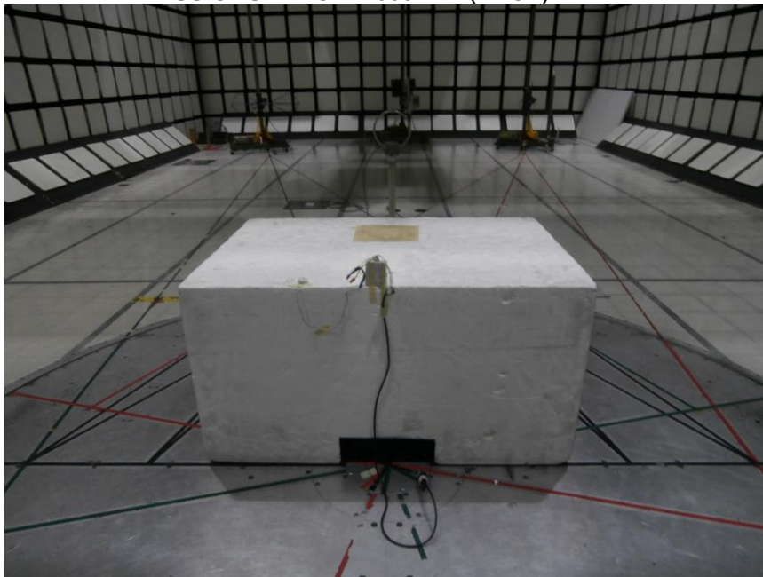
RADIATED EMISSIONS BELOW 1000MHz (BACK)
