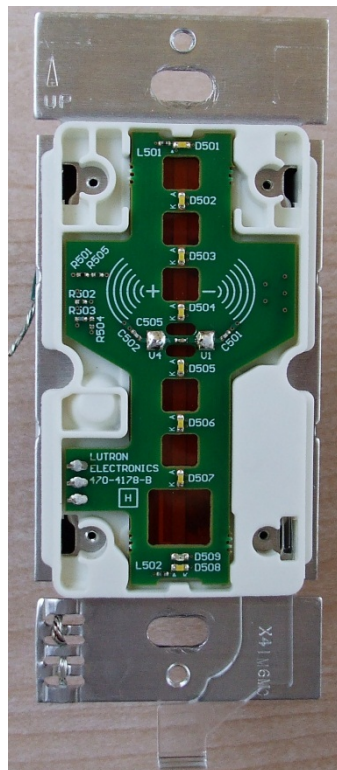
GT-RF2 Antenna Removed
