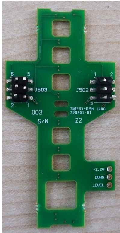
GT-RF2 Back of Front Board
