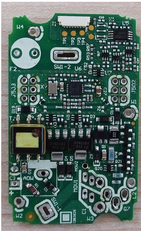
GT-RF2 Back of Power board
