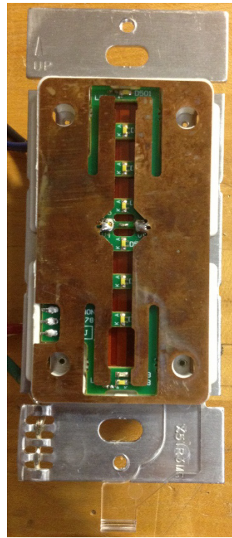
GT-RF2 Bezel Removed
