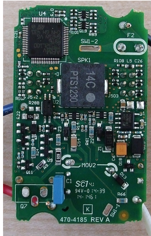
GT-RF2 Front of Power Board
