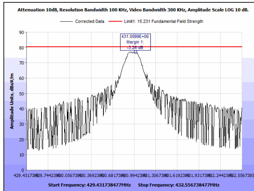
Plot 2. Fundamental Field Strength, 430 MHz with DCCF (77.44dBuV/m)
