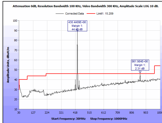
Plot 4. Spurious Emissions, 430 MHz, 30 MHz – 1 GHz
