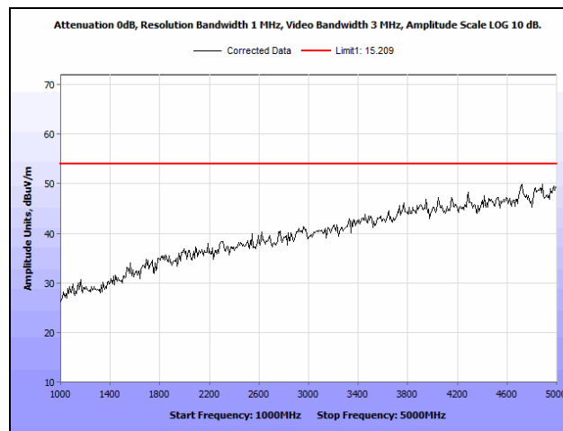
Plot 5. Spurious Emissions, 430 MHz, 1 GHz – 5 GHz
