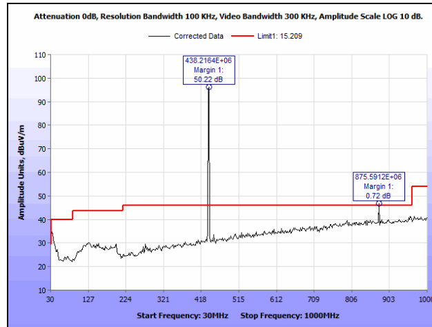
Plot 7. Spurious Emissions, 437 MHz, 30 MHz – 1 GHz
