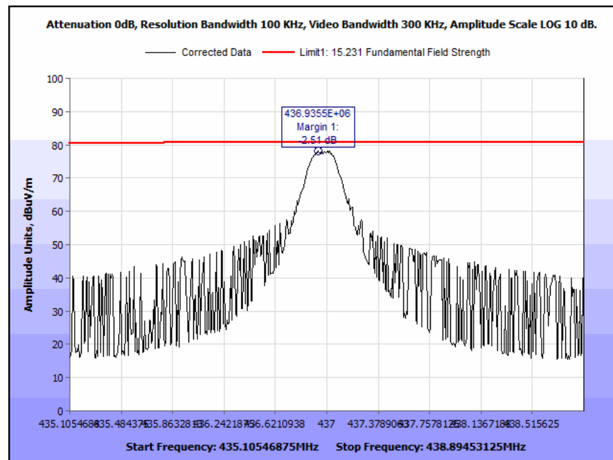
Plot 3. Fundamental Field Strength, 437 MHz with DCCF (78.39dBuV/m)
