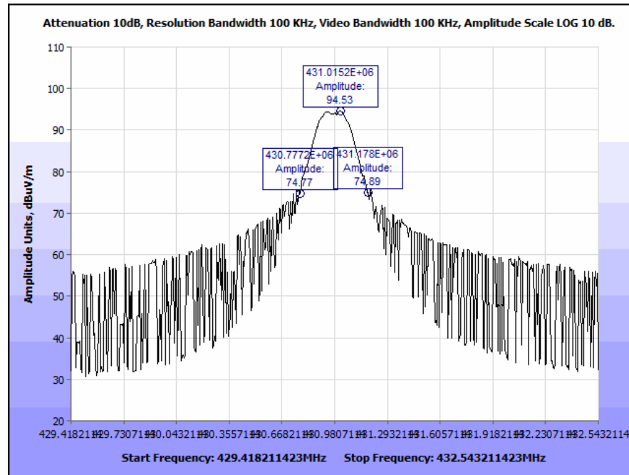
Plot 8. Occupied Bandwidth, 431 MHz
