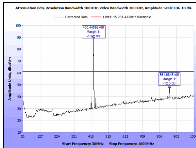
Plot 6. Spurious Emissions, 430 MHz, 30 MHz – 1 GHz, Harmonic
