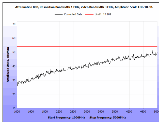
Plot 8. Spurious Emissions, 437 MHz, 1 GHz – 5 GHz
