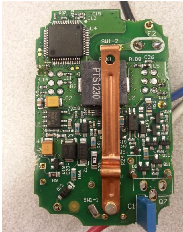
Back Board and Side of Unit, Identical for all Devices
