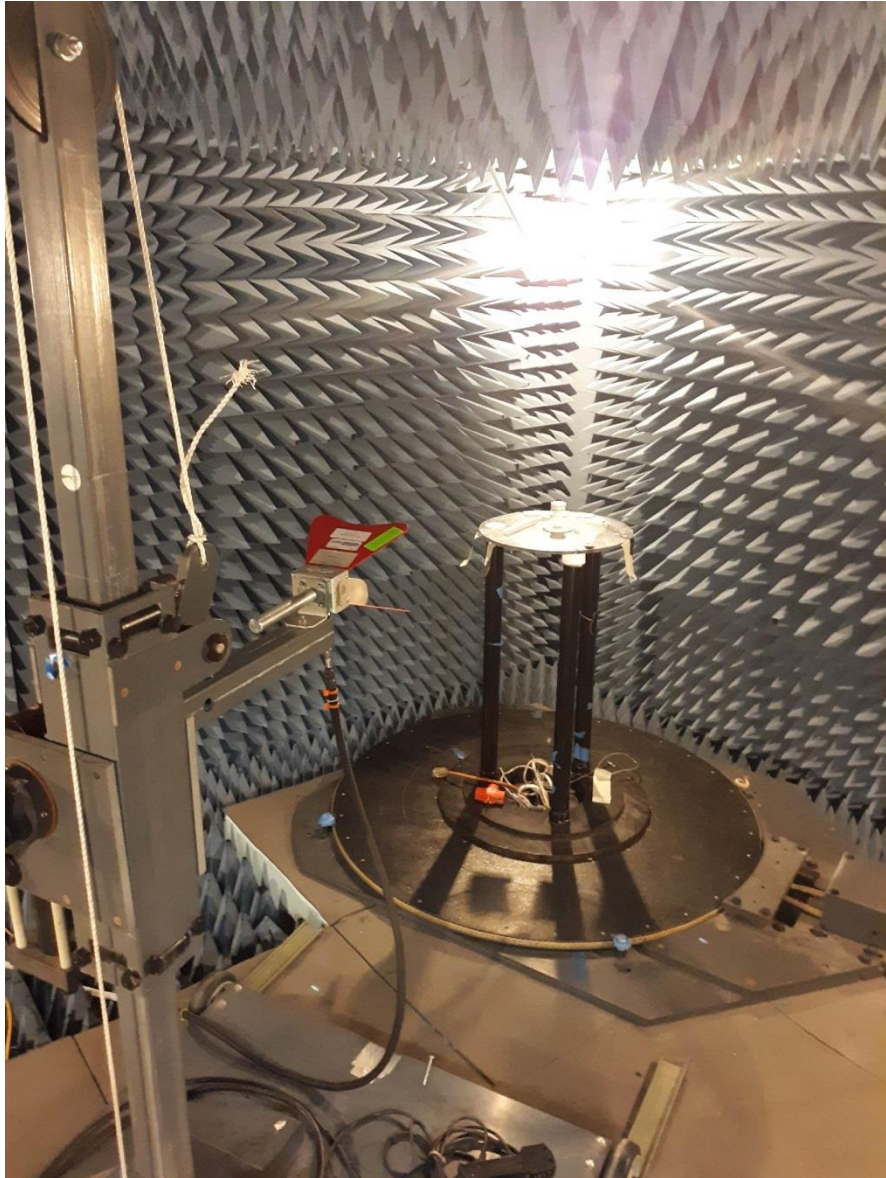
Photograph 1. Radiated Emissions, Spurious Above 1 GHz
