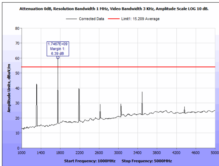
Plot 15. Radiated Spurious Emissions, Average, Ch. 436.6 MHz, 1-5 GHz
