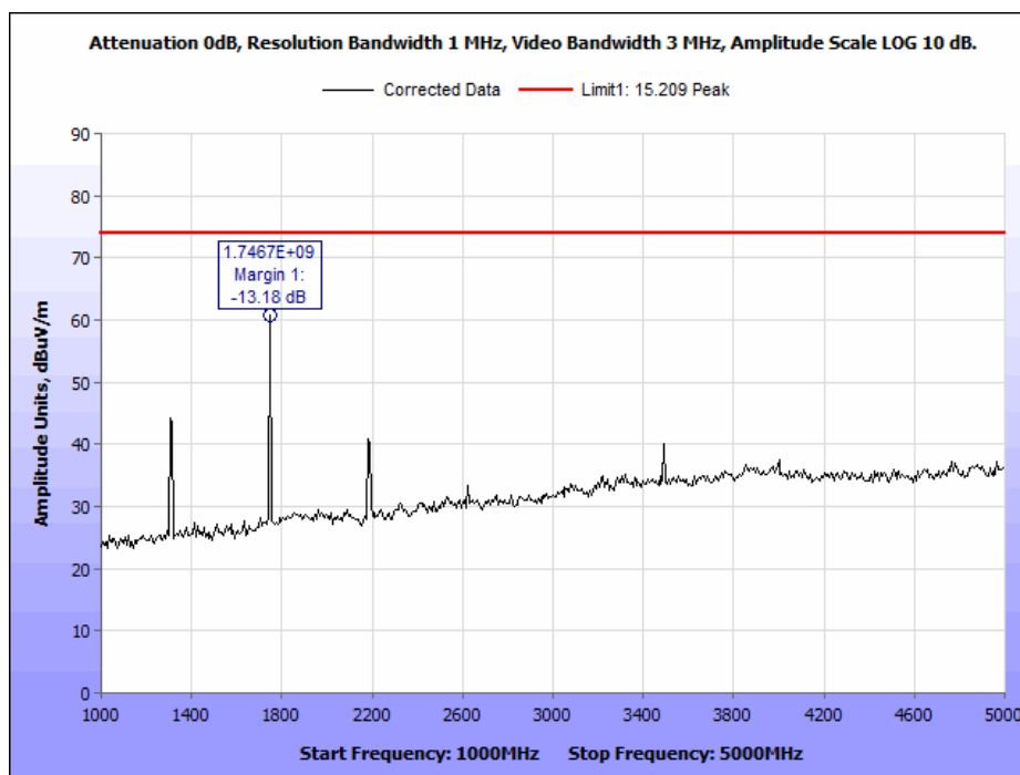
Plot 18. Radiated Spurious Emissions, Peak, Ch. 436.6 MHz, 1-5 GHz
