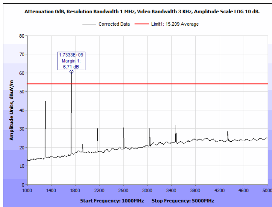
Plot 17. Radiated Spurious Emissions, Average, Ch. 433.6 MHz, 1-5 GHz
