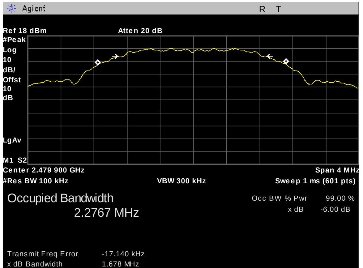
Figure 17: 6 dB Bandwidth, High Channel, 2480 MHz
