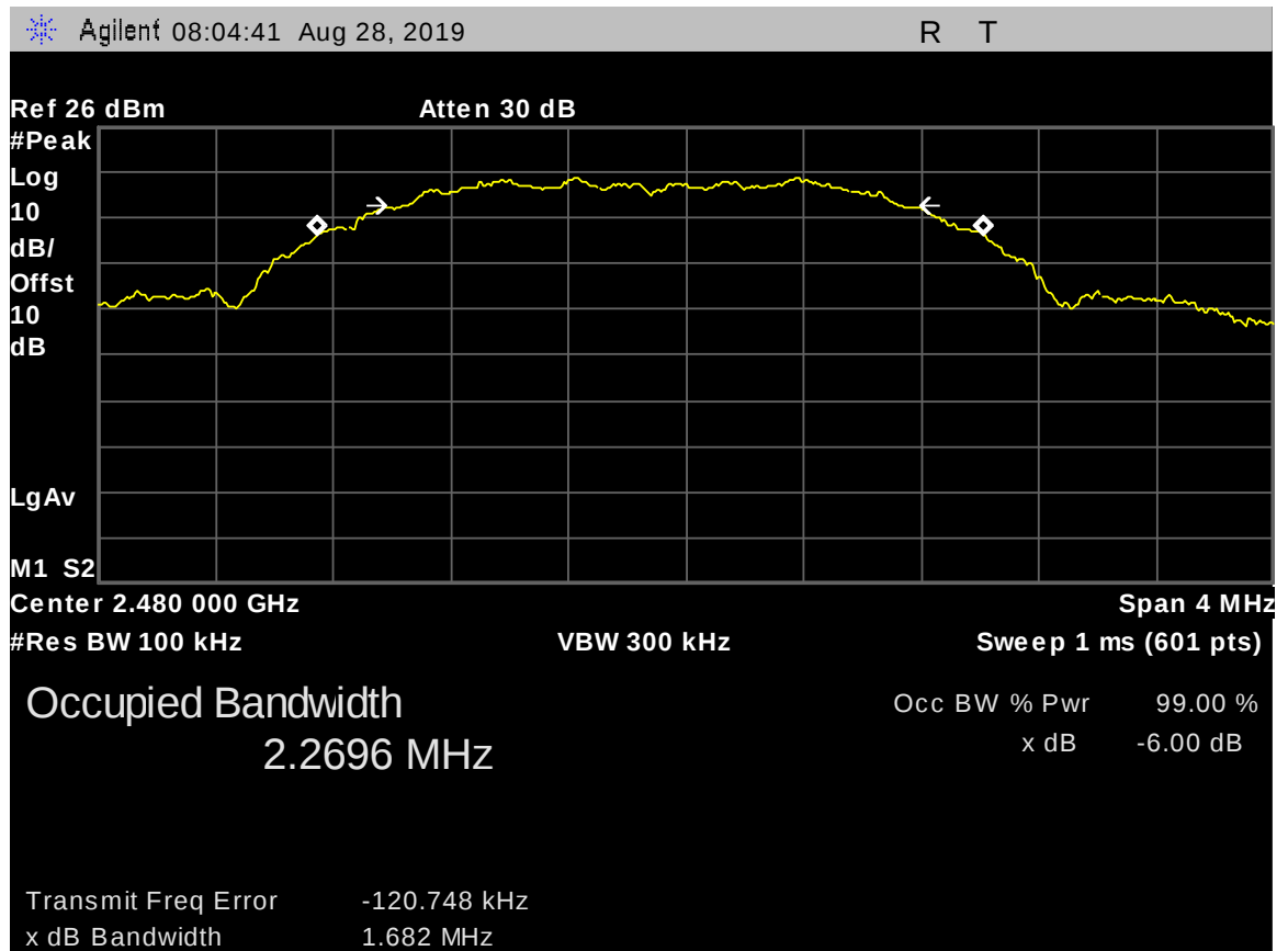
Figure 17: 6dB Bandwidth, ANT2, 2480 MHz
