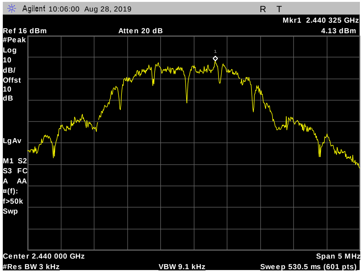
Figure 48: Peak Power Spectral Density, ANT2, 2440 MHz
