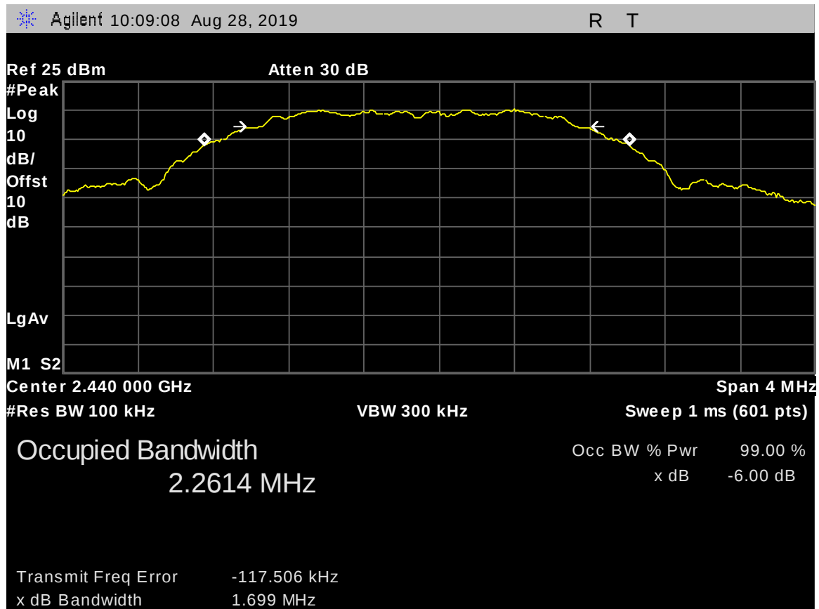
Figure 16: 6dB Bandwidth, ANT2, 2440 MHz
