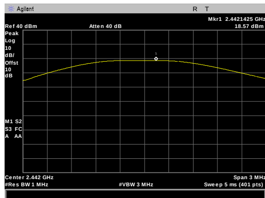
Figure 9: Power Output, BLE Mid Channel, Peak Conducted Power
