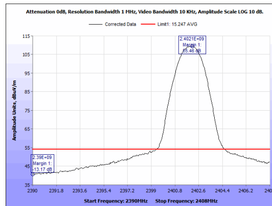
Figure 51: Radiated Emissions, BLE Low Channel, Band Edge, Average, Antenna 2
