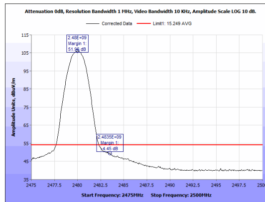
Figure 53: Radiated Emissions, BLE High Channel, Band Edge, Average, Antenna 1
