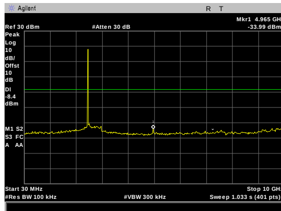
Figure 63: Conducted Spurious Emissions, BLE High Channel, 30 MHz - 10 GHz
