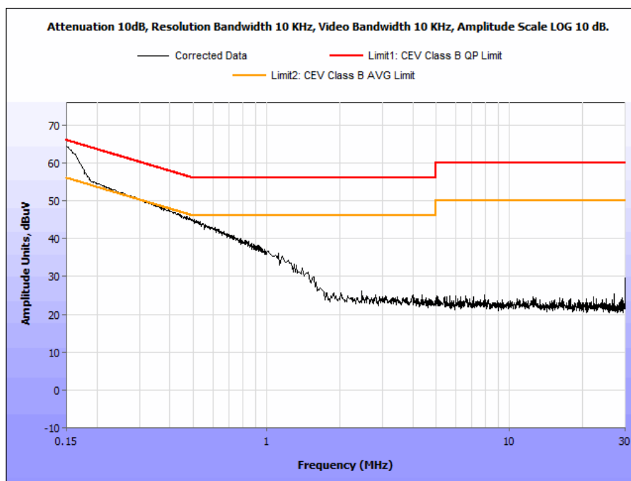
Figure 2: Conducted Emissions, Plot, Phase BLE
