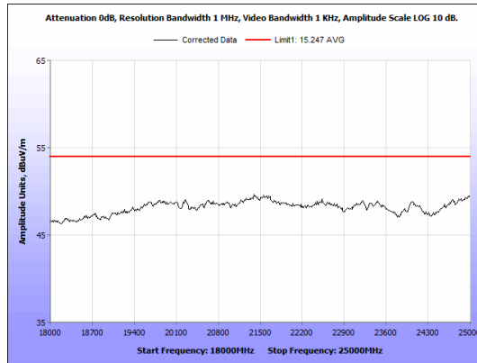
Figure 14: Radiated Emissions, BLE Low Channel, 18GHz - 25GHz, Average, Antenna 1
