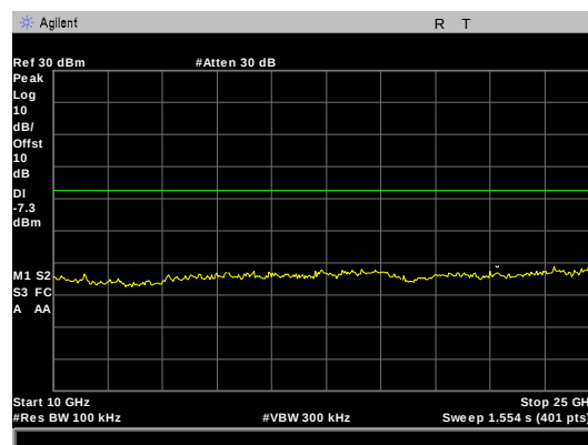
Figure 59: Conducted Spurious Emissions, BLE Low Channel 10 GHz - 25 GHz
