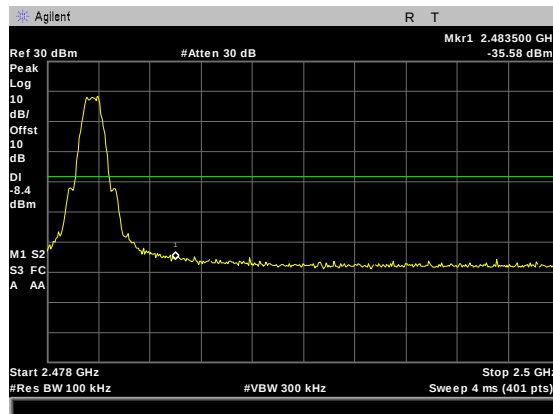
Figure 67: Conducted Spurious Emissions, BLE High Channel, band edge
