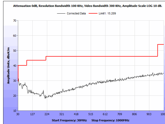
Figure 11: Radiated Emissions, BLE Low Channel, 30 MHz - 1 GHz, Antenna 1
