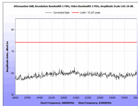
Figure 16: Radiated Emissions, BLE Low Channel, 18GHz - 25GHz, Peak, Antenna 1
