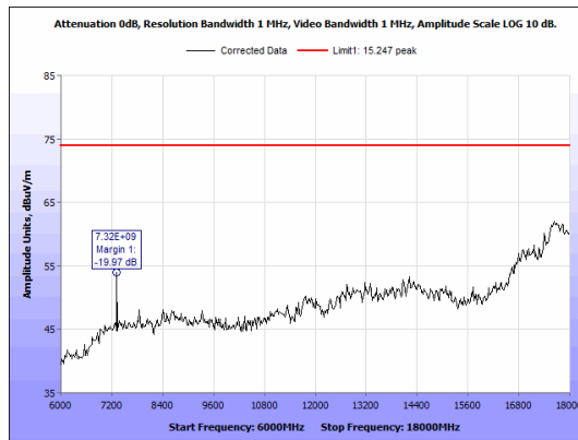
Figure 40: Radiated Emissions, BLE Mid Channel, 6GHz - 18GHz, Peak, Antenna 2
