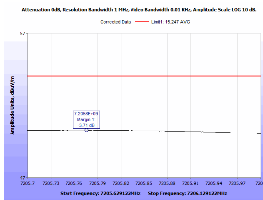
Figure 29: Radiated Emissions, BLE Low Channel, Average, 7.2 GHz, emission, Antenna 2
