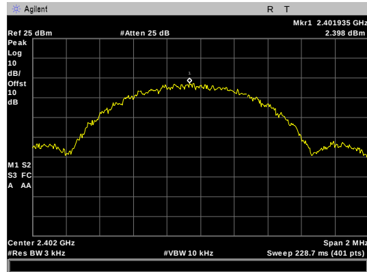
Figure 68: Power Spectral Density, BLE Low Channel
