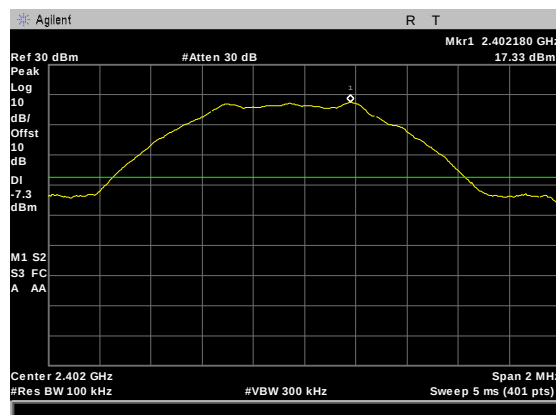
Figure 58: Conducted Spurious Emissions, BLE Low Channel reference level measurement
