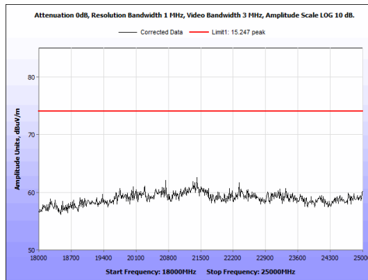
Figure 34: Radiated Emissions, BLE Low Channel 18GHz - 25GHz, Peak, Antenna 2
