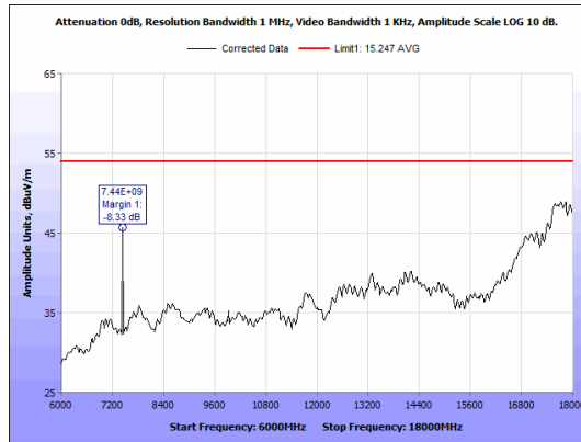
Figure 44: Radiated Emissions, BLE High Channel, 6GHz - 18GHz, Average, Antenna 2
