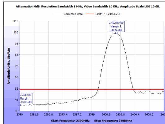
Figure 49: Radiated Emissions, BLE Low Channel, Band Edge, Average, Antenna 1
