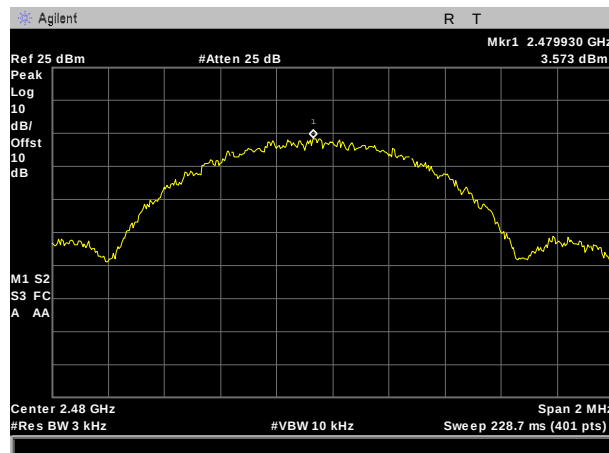
Figure 70: Power Spectral Density, BLE High Channel
