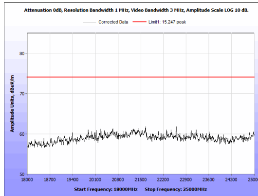
Figure 48: Radiated Emissions, BLE High Channel, 18GHz - 25GHz, Peak, Antenna 2
