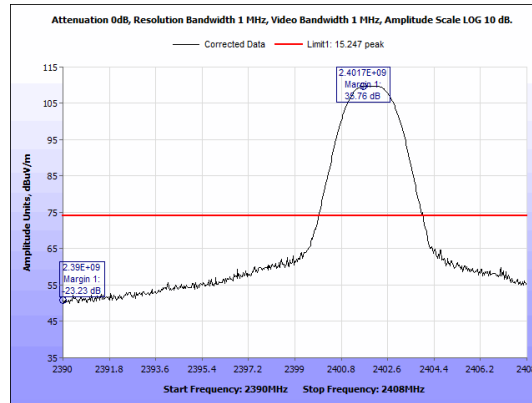
Figure 52: Radiated Emissions, BLE Low Channel, Band Edge, Peak, Antenna 2
