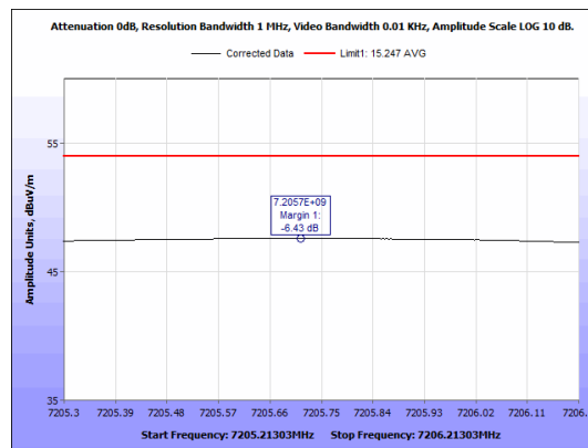
Figure 12: Radiated Emissions, BLE Low Channel, Average, 7.2 GHz emission, Antenna 1
