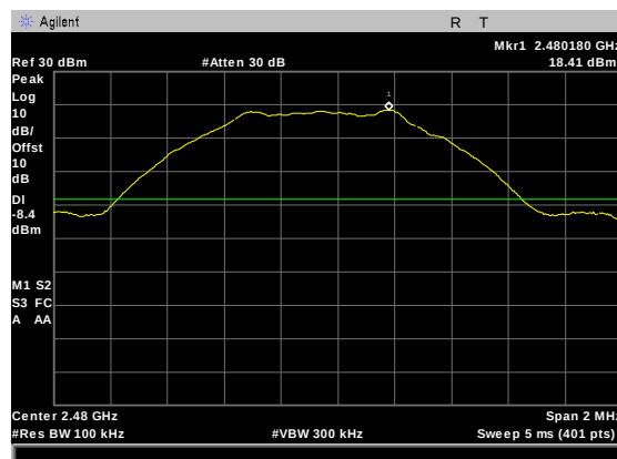
Figure 65: Conducted Spurious Emissions, BLE High Channel, reference level measurement
