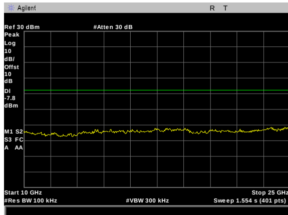
Figure 61: Conducted Spurious Emissions, BLE Mid Channel, 10 GHz - 25 GHz
