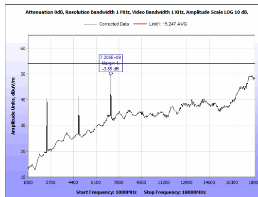
Figure 13: Radiated Emissions, BLE Low Channel, 1GHz - 18GHz, Average, Antenna 1
