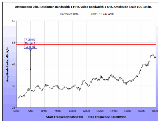
Figure 30: Radiated Emissions, BLE Low Channel 6GHz - 18GHz, Average, Antenna 2
