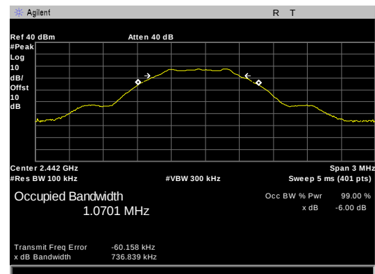
Figure 6: 6 dB Occupied Bandwidth, 6 dB DTS Bandwidth, BLE Mid Channel
