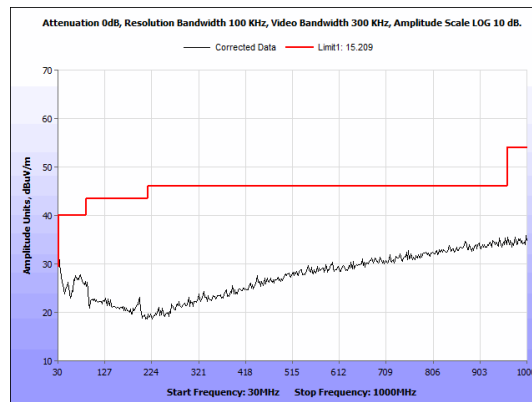
Figure 22: Radiated Emissions, BLE High Channel, 30 MHz - 1 GHz Antenna 1
