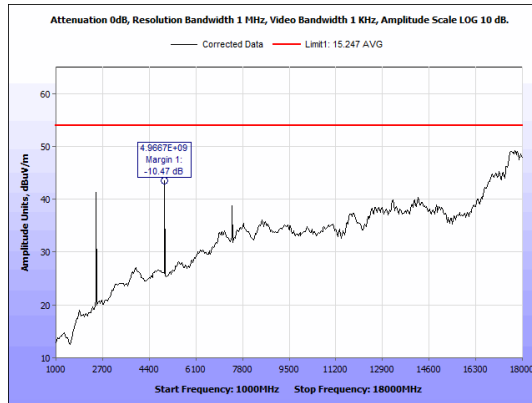
Figure 23: Radiated Emissions, BLE High Channel, 1GHz - 18GHz, Average, Antenna 1
