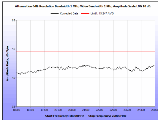
Figure 24: Radiated Emissions, BLE High Channel, 18GHz - 25GHz, Average, Antenna 1
