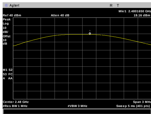
Figure 10: Power Output, BLE High Channel, Peak Conducted Power
