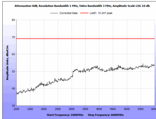
Figure 32: Radiated Emissions, BLE Low Channel 1GHz - 6 GHz, Peak, Antenna 2
