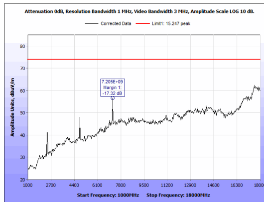
Figure 15: Radiated Emissions, BLE Low Channel, 1GHz - 18GHz, Peak, Antenna 1
