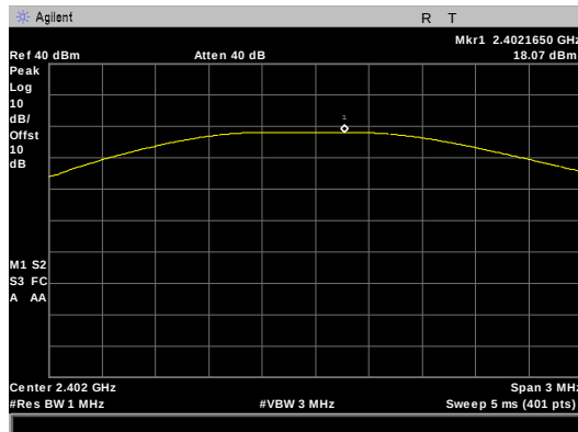
Figure 8: Power Output, BLE Low Channel, Peak Conducted Power
