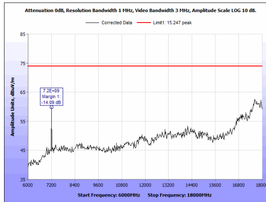
Figure 33: Radiated Emissions, BLE Low Channel 6GHz - 18GHz, Peak, Antenna 2
