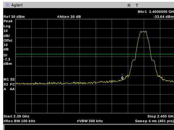
Figure 66: Conducted Spurious Emissions, BLE Low Channel band edge
