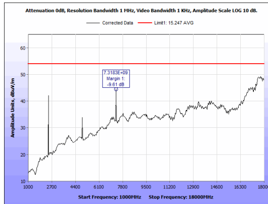
Figure 18: Radiated Emissions, BLE Mid Channel, 1GHz - 18GHz, Average, Antenna 1
