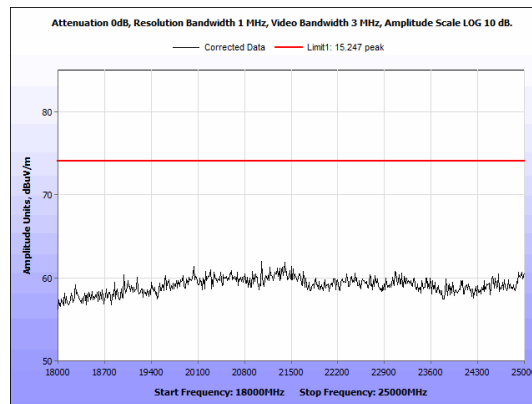
Figure 21: Radiated Emissions, BLE Mid Channel, 18GHz - 25GHz, Peak, Antenna 1
