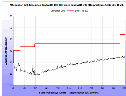
Figure 42: Radiated Emissions, BLE High Channel, 30 MHz - 1 GHz Antenna 2
