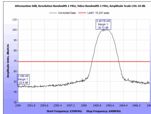
Figure 50: Radiated Emissions, BLE Low Channel, Band Edge, Peak, Antenna 1
