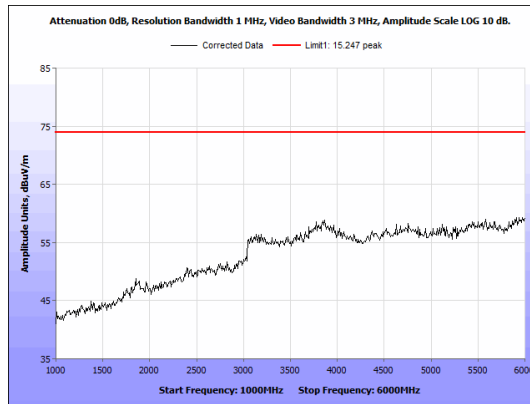
Figure 39: Radiated Emissions, BLE Mid Channel, 1GHz - 6 GHz, Peak, Antenna 2
