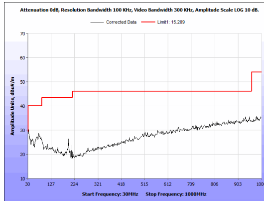
Figure 35: Radiated Emissions, BLE Mid Channel, 30 MHz - 1 GHz Antenna 2
