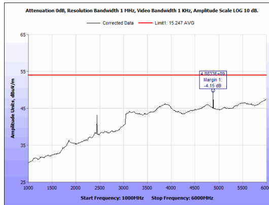
Figure 36: Radiated Emissions, BLE Mid Channel, 1GHz - 6 GHz, Average, Antenna 2
