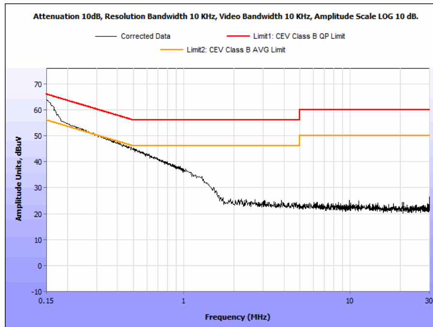
Figure 3: Conducted Emissions, Plot, Neutral BLE
