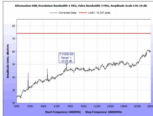
Figure 20: Radiated Emissions, BLE Mid Channel, 1GHz - 18GHz, Peak, Antenna 1
