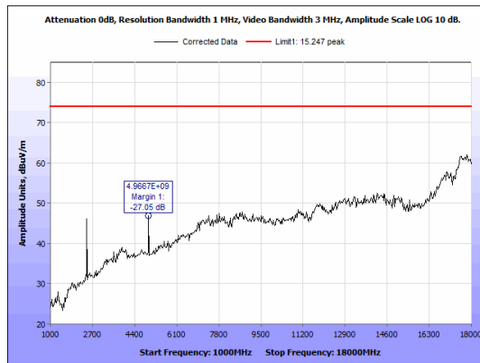
Figure 25: Radiated Emissions, BLE High Channel, 1GHz - 18GHz, Peak, Antenna 1
