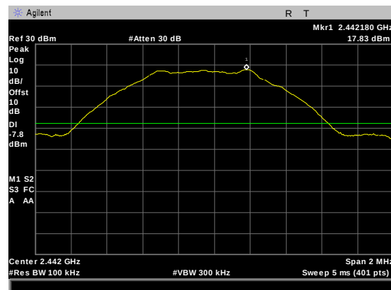
Figure 62: Conducted Spurious Emissions, BLE Mid Channel, reference level measurement
