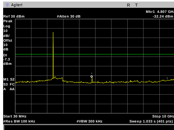
Figure 57: Conducted Spurious Emissions, BLE Low Channel 30 MHz - 10 GHz
