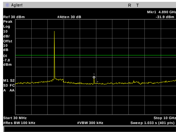
Figure 60: Conducted Spurious Emissions, BLE Mid Channel, 30 MHz - 10 GHz
