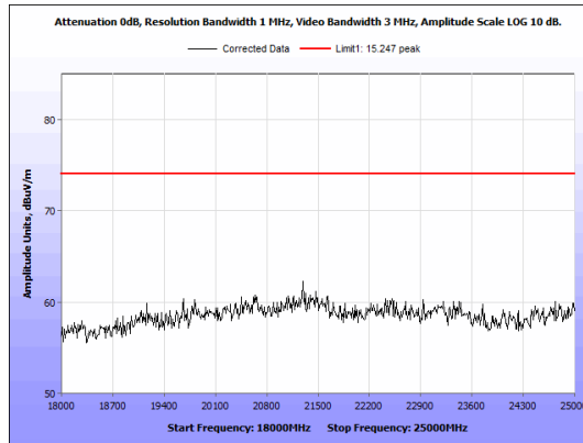
Figure 41: Radiated Emissions, BLE Mid Channel, 18GHz - 25GHz, Peak, Antenna 2
