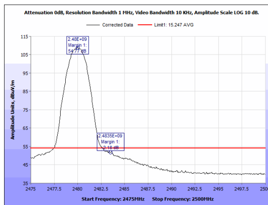
Figure 56: Radiated Emissions, BLE High Channel, Band Edge, Average, Antenna 2
