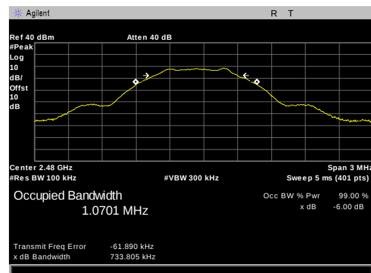
Figure 7: 6 dB Occupied Bandwidth, BLE High Channel
