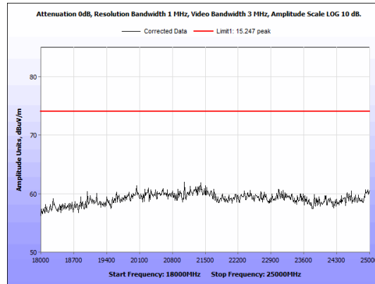
Figure 26: Radiated Emissions, BLE High Channel, 18GHz - 25GHz, Peak, Antenna 1
