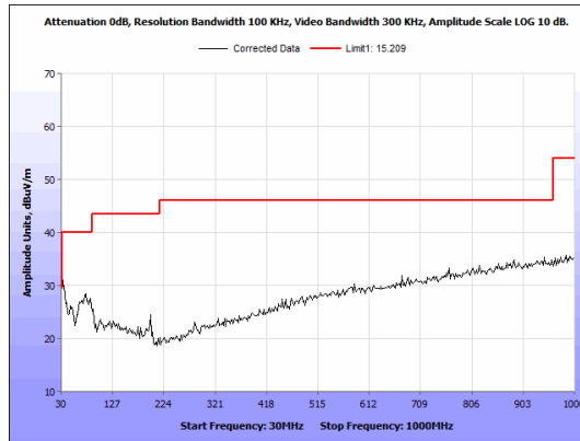
Figure 17: Radiated Emissions, BLE Mid Channel, 30 MHz - 1 GHz Antenna 1
