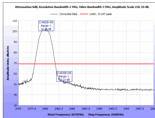
Figure 54: Radiated Emissions, BLE High Channel, Band Edge, Peak, Antenna 1
