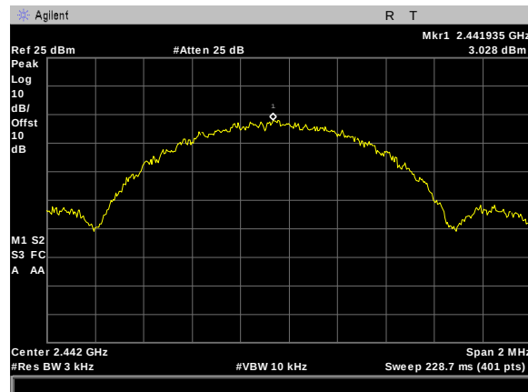
Figure 69: Power Spectral Density, BLE Mid Channel
