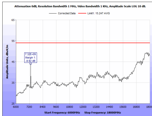
Figure 37: Radiated Emissions, BLE Mid Channel, 6GHz - 18GHz, Average, Antenna 2
