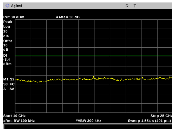
Figure 64: Conducted Spurious Emissions, BLE High Channel, 10 GHz - 25 GHz
