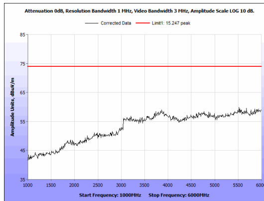
Figure 46: Radiated Emissions, BLE High Channel, 1GHz - 6 GHz, Peak, Antenna 2
