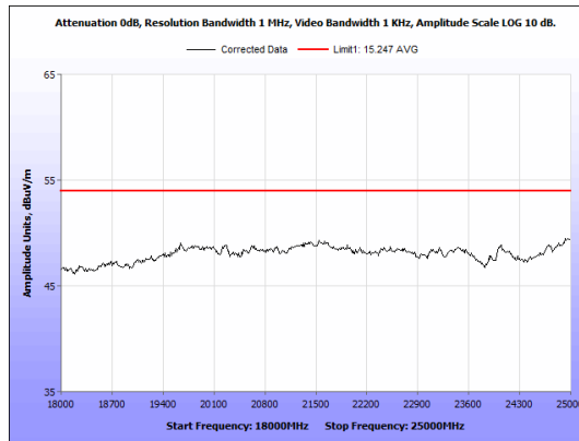
Figure 45: Radiated Emissions, BLE High Channel, 18GHz - 25GHz, Average, Antenna 2
