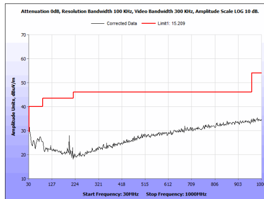
Figure 27: Radiated Emissions, BLE Low Channel, 30 MHz - 1 GHz, Antenna 2
