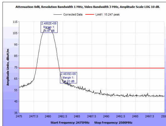
Figure 55: Radiated Emissions, BLE High Channel, Band Edge, Peak, Antenna 2
