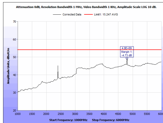
Figure 28: Radiated Emissions, BLE Low Channel, 1GHz - 6 GHz, Average, Antenna 2
