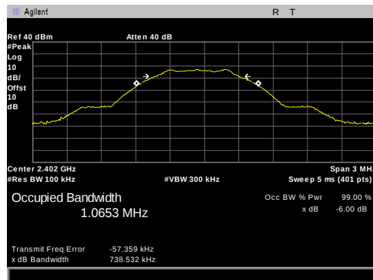
Figure 5: 6 dB Occupied Bandwidth, BLE Low Channel
