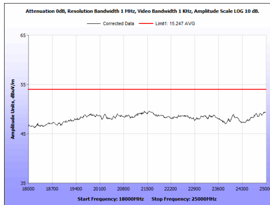
Figure 19: Radiated Emissions, BLE Mid Channel, 18GHz - 25GHz, Average, Antenna 1
