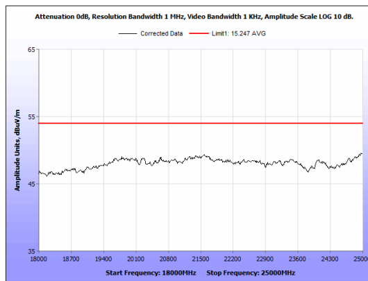
Figure 31: Radiated Emissions, BLE Low Channel 18GHz - 25GHz, Average, Antenna 2
