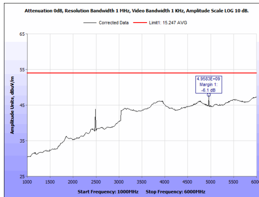
Figure 43: Radiated Emissions, BLE High Channel, 1GHz - 6 GHz, Average, Antenna 2
