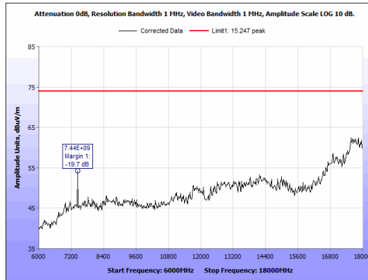
Figure 47: Radiated Emissions, BLE High Channel, 6GHz - 18GHz, Peak, Antenna 2
