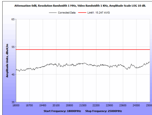
Figure 38: Radiated Emissions, BLE Mid Channel, 18GHz - 25GHz, Average, Antenna 2
