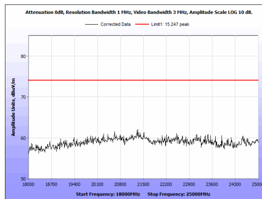
Figure 31: Radiated Emissions, ZigBee, 18GHz - 25GHz Peak, Low Channel, Antenna 2
