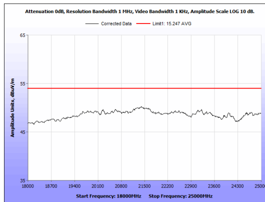
Figure 15: Radiated Emissions, ZigBee, 18GHz - 25GHz, Average, Low Channel, Antenna 1
