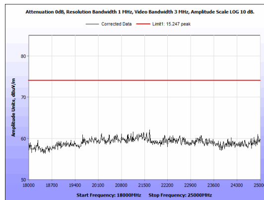
Figure 25: Radiated Emissions, ZigBee, 18GHz - 25GHz Peak, High channel, Antenna 1
