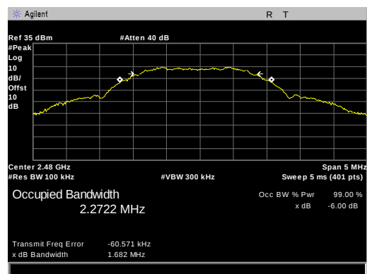
Figure 7: 6 dB Occupied Bandwidth, ZigBee High channel
