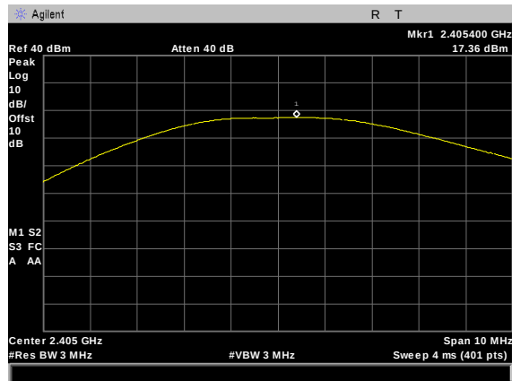
Figure 8: Conducted Power, ZigBee Low channel Peak
