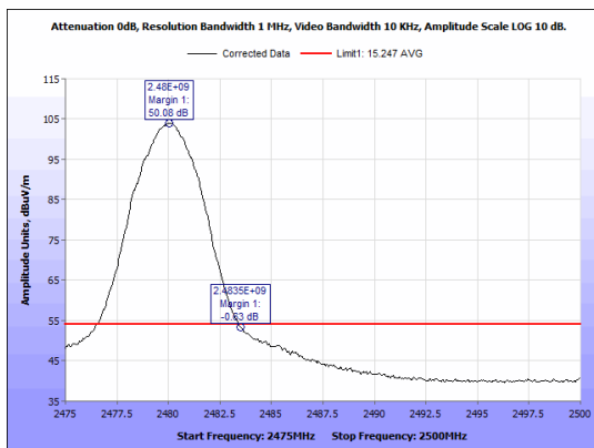
Figure 48: Radiated Emissions, ZigBee High Channel Band Edge, Average, Antenna 1
