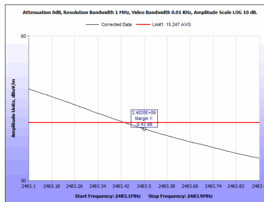
Figure 52: Radiated Emissions, ZigBee High Channel Band Edge, Average, 10Hz Antenna 2
