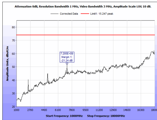
Figure 14: Radiated Emissions, ZigBee, 1GHz - 18GHz Peak, Low Channel, Antenna 1
