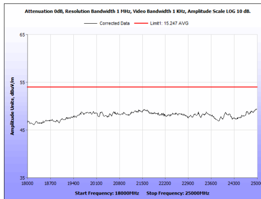
Figure 40: Radiated Emissions, ZigBee, 18GHz - 25GHz, Average, High channel, Antenna 2
