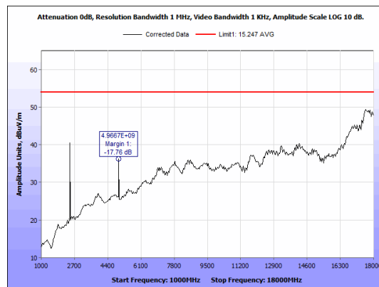
Figure 22: Radiated Emissions, ZigBee, 1GHz - 18GHz, Average, High channel, Antenna 1
