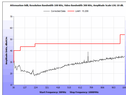
Figure 21: Radiated Emissions, ZigBee, 30 MHz - 1 GHz, High channel, Antenna 1
