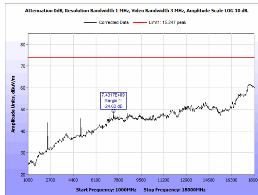
Figure 23: Radiated Emissions, ZigBee, 1GHz - 18GHz Peak, High channel, Antenna 1
