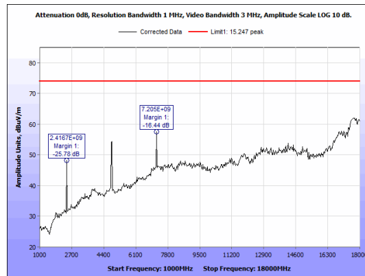
Figure 29: Radiated Emissions, ZigBee, 1GHz - 18GHz Peak, Low Channel, Antenna 2
