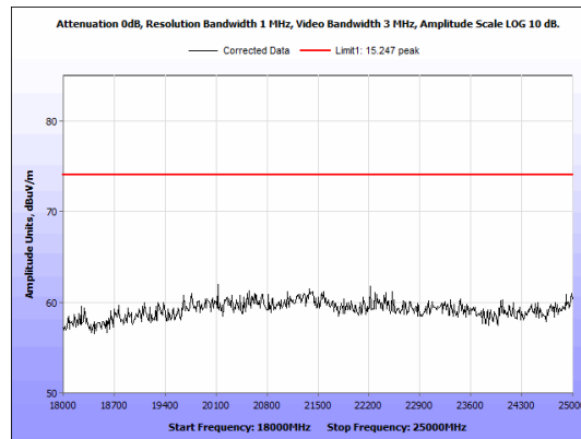
Figure 20: Radiated Emissions, ZigBee, 18GHz - 25GHz Peak, Mid Channel, Antenna 1
