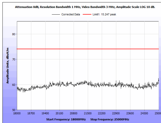
Figure 16: Radiated Emissions, ZigBee, 18GHz - 25GHz Peak, Low Channel, Antenna 1
