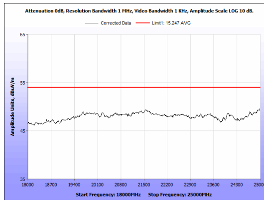
Figure 35: Radiated Emissions, ZigBee, 18GHz - 25GHz, Average, Mid Channel, Antenna 2
