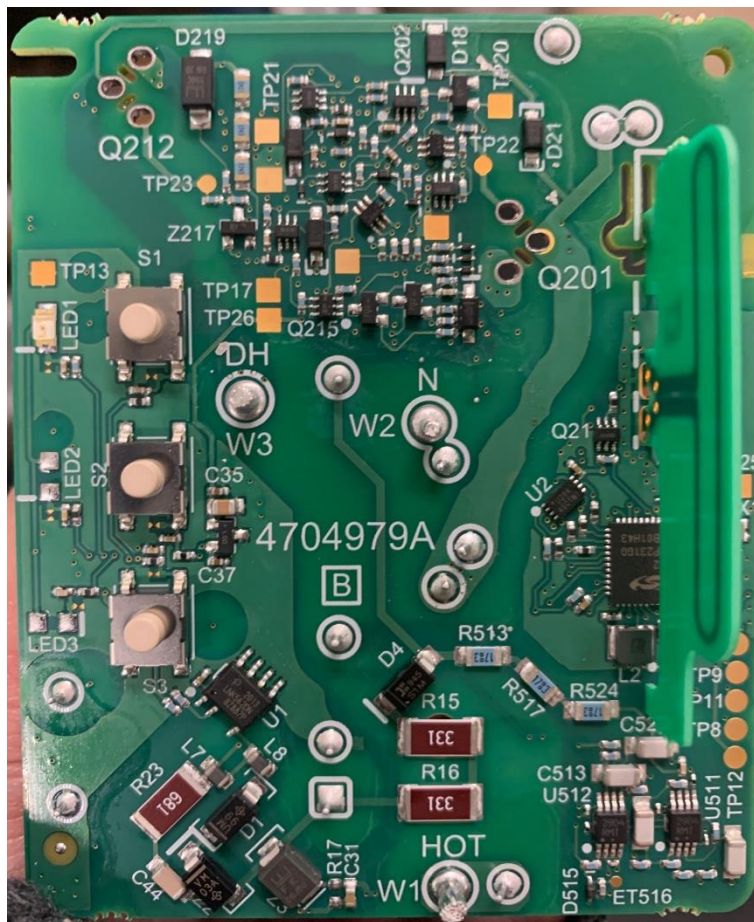
TOP OF PCB
