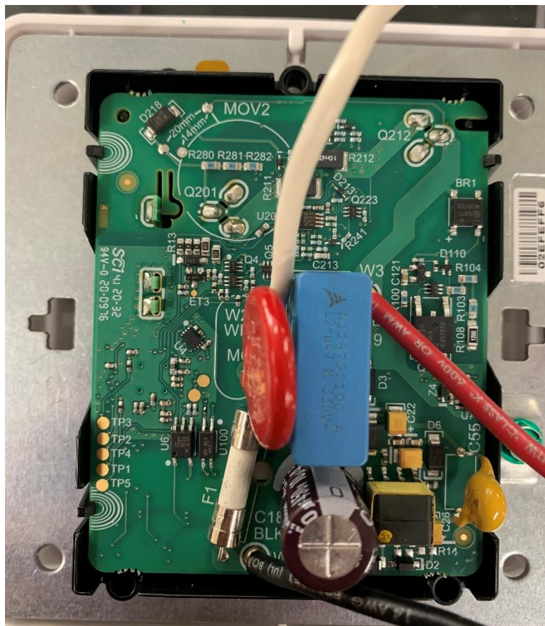
BOTTOM OF PCB WITH MOV LIFTED
