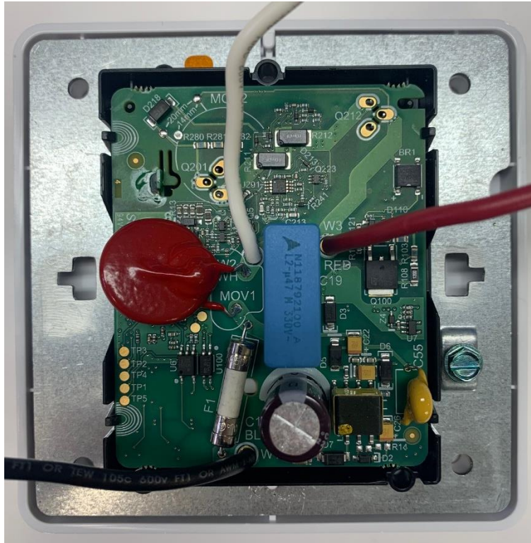
BOTTOM OF PCB
