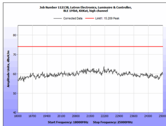
Figure 51: Cabinet Radiated Emissions, BLE 1Mbit High Channel 18GHz-25GHz Peak.
