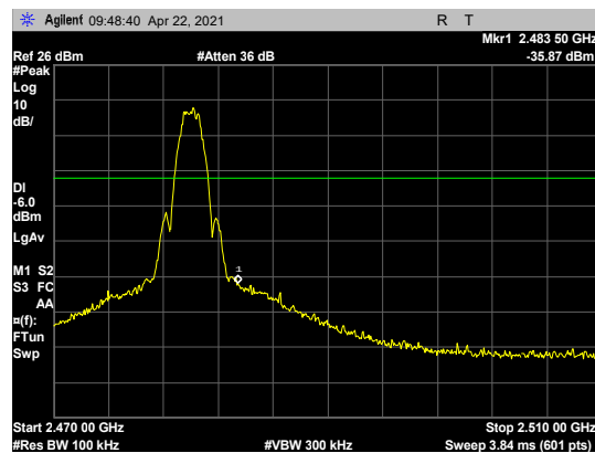
Figure 87: Conducted Spurious Emissions, BLE 2Mbit high channel band edge
