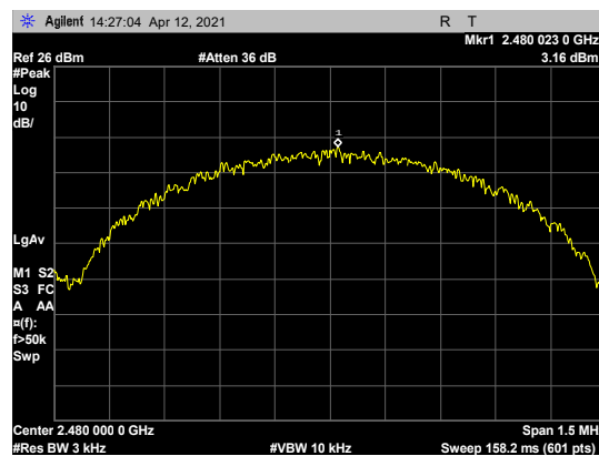
Figure 91: Power Spectral Density, BLE 1Mbit high channel Peak
