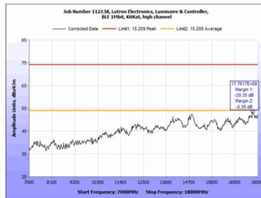
Figure 49: Cabinet Radiated Emissions, BLE 1Mbit High Channel 7GHz-18GHz PK and AVG.
