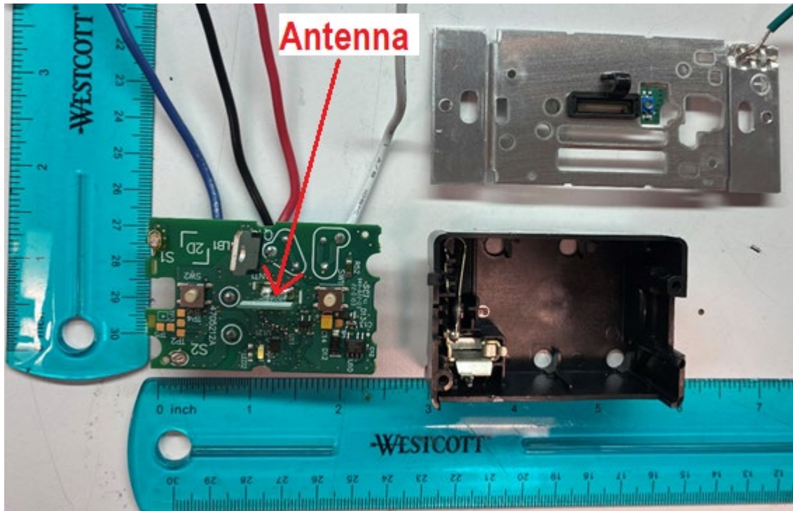
Top Side View (with Enclosure)
