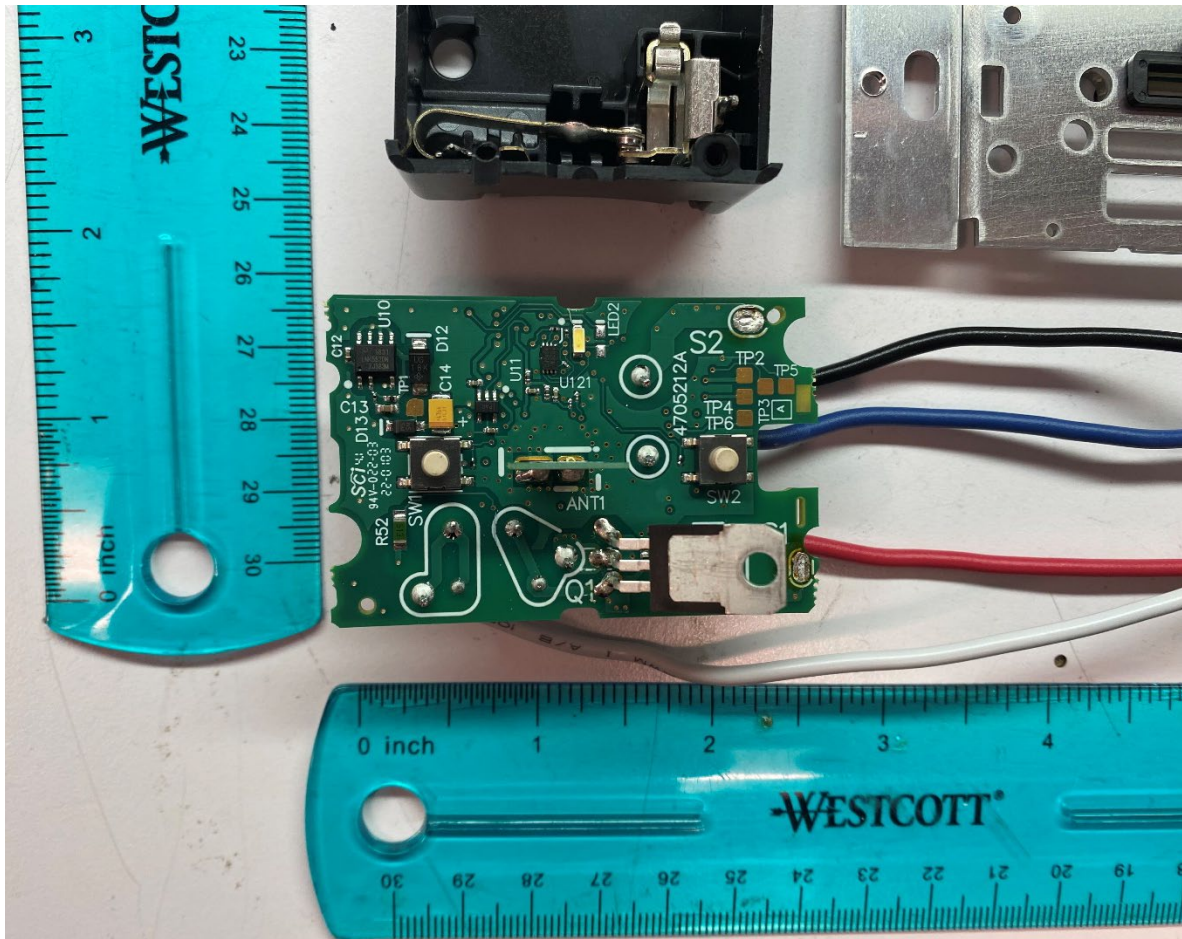
Top Side PCB View
