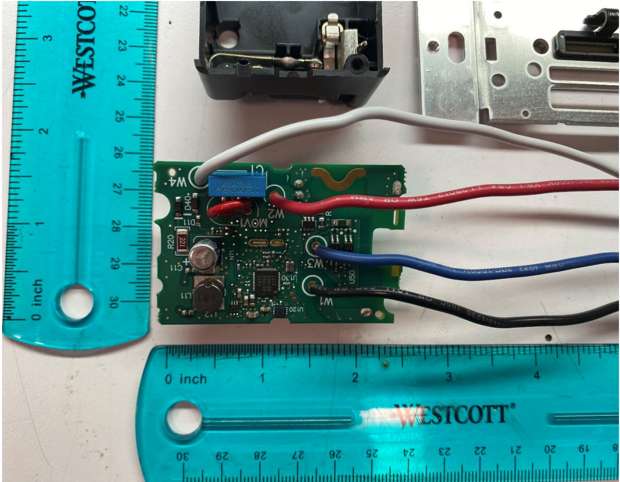
Bottom Side PCB View
