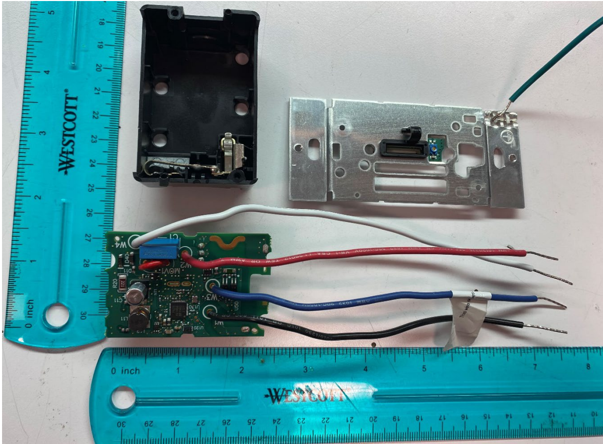
Bottom Side PCB View (with Enclosure)
