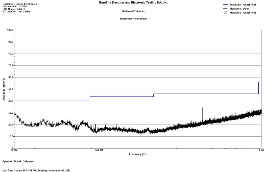
Figure 5. Radiated Spurious Emissions - Low Channel, 30-1000 MHz Horizontal Polarization
