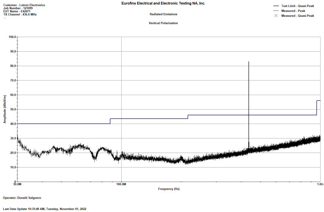
Figure 10. Radiated Spurious Emissions - High Channel, 30-1000 MHz Vertical Polarization
