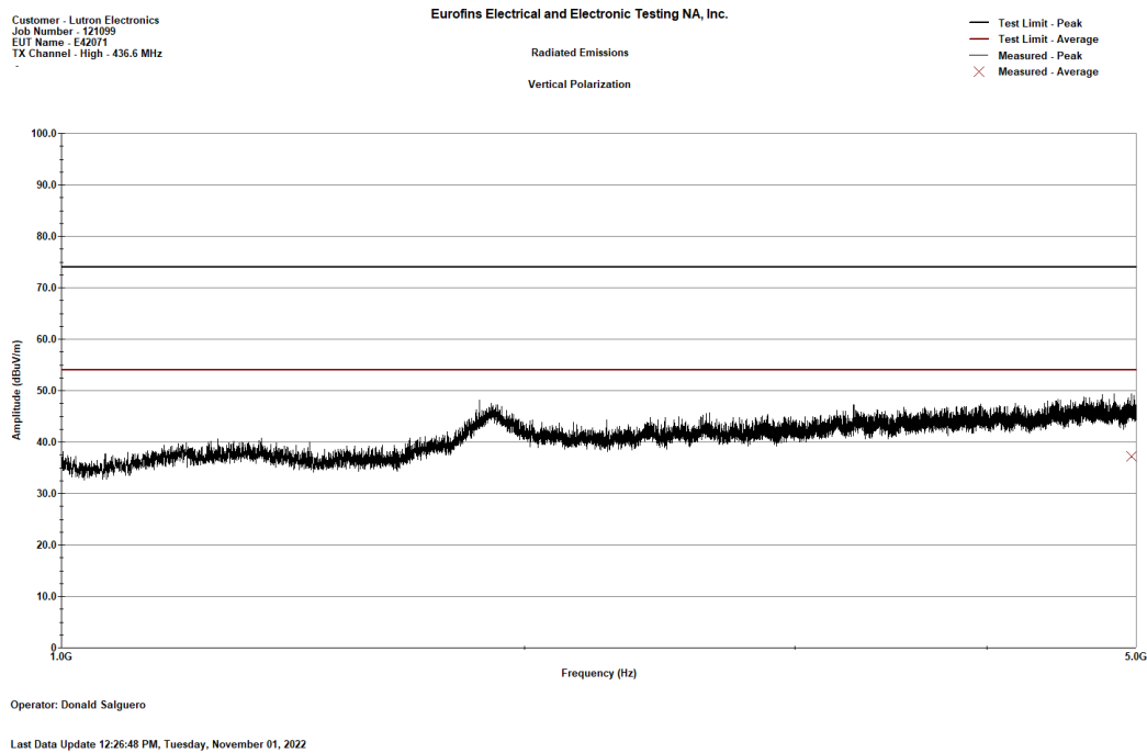
Figure 12. Radiated Spurious Emissions - High Channel, 1-5 GHz Vertical Polarization
