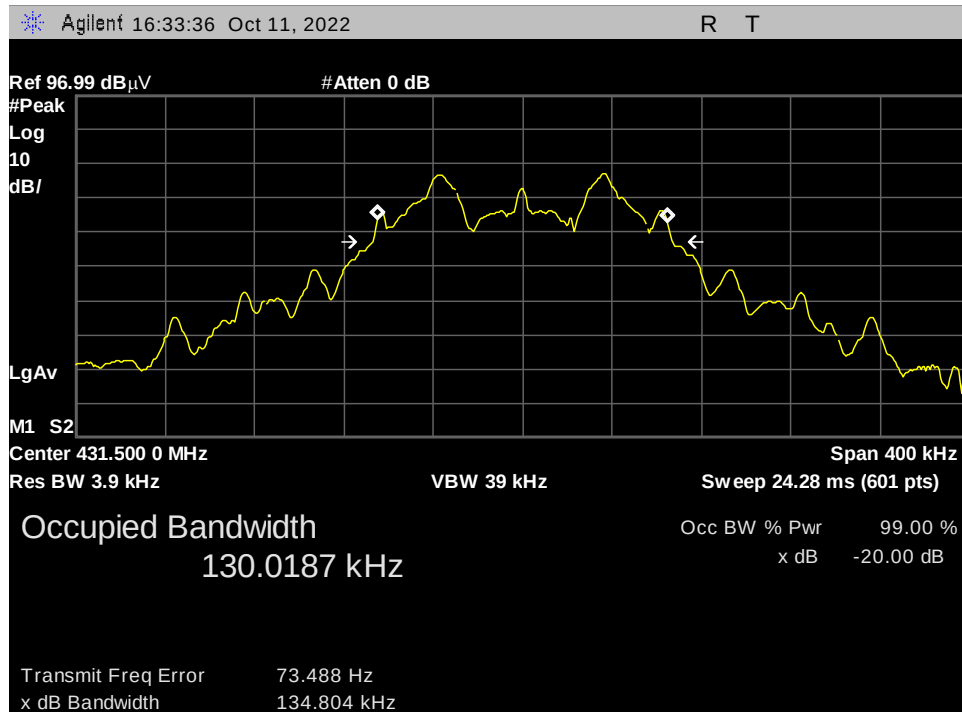
Figure 17. OBW Low Channel
