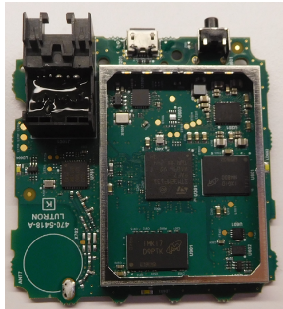
PWB top w/ shield removed
