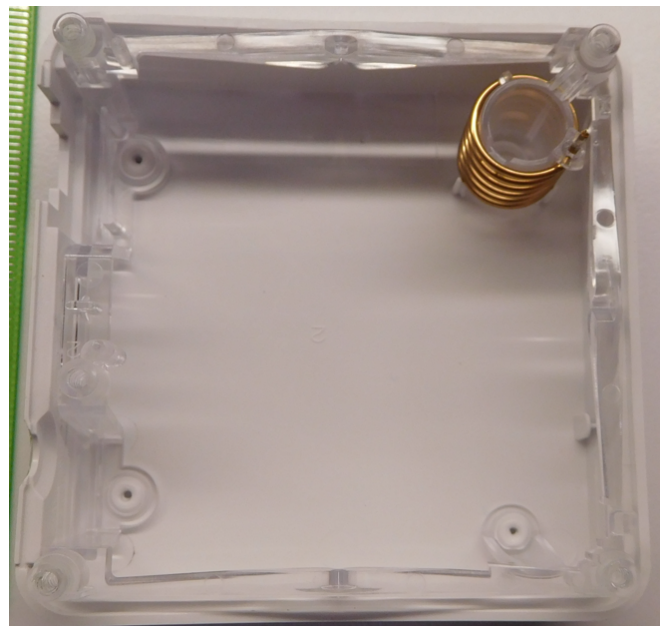
DUT inside top w/ antenna
