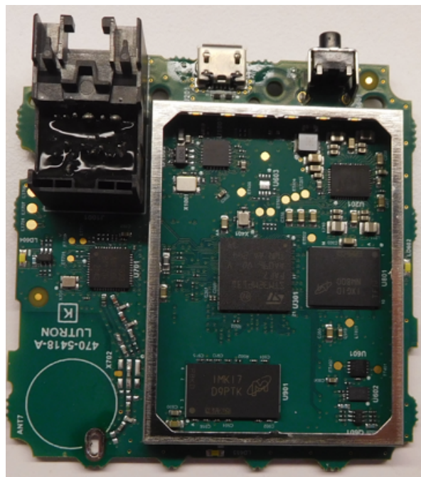
PWB top w/ shield removed
