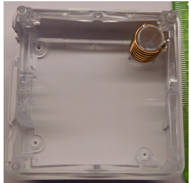
DUT inside top w/ antenna
