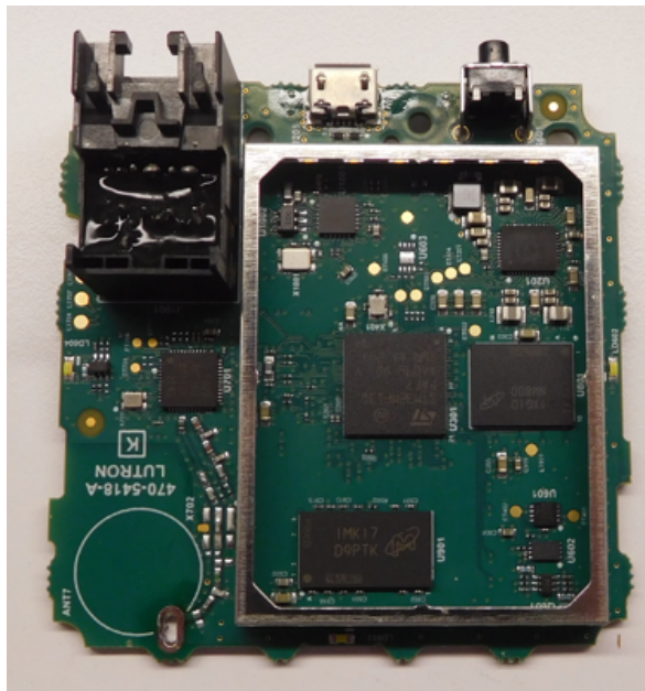
PWB top w/ shield removed
