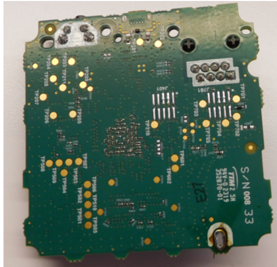
DUT with back cover removed
