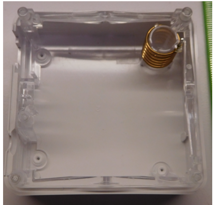
DUT inside top w/ antenna
