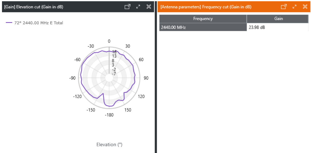
Figure 2: Peak Gain
