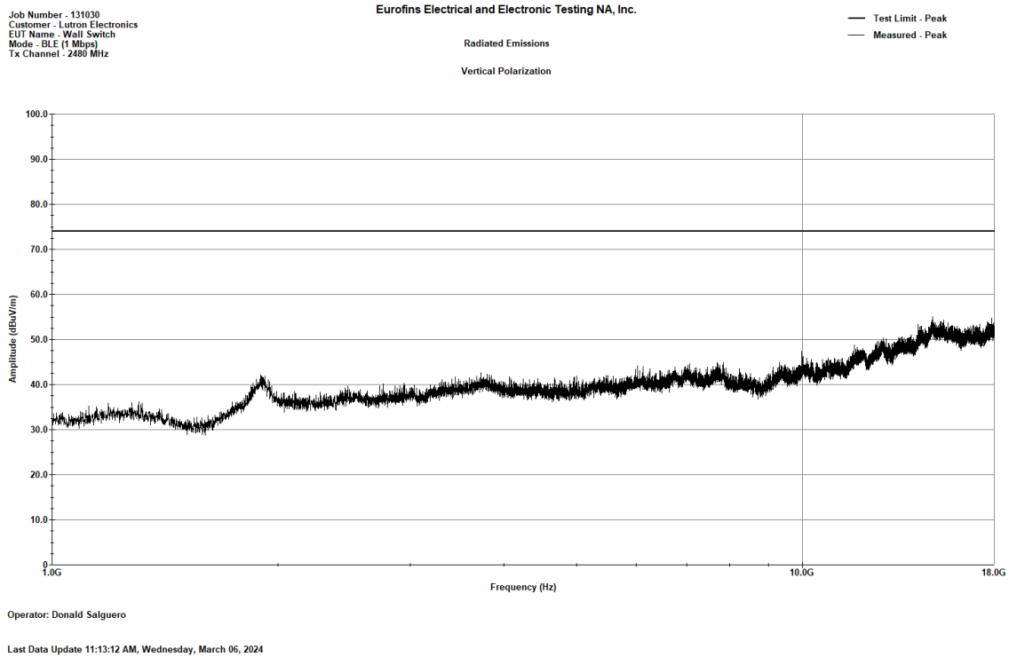
Figure 60. BLE (1 Mbps)_2480MHz_Radiated Emissions, Peak, 1 - 18 GHz-_V
