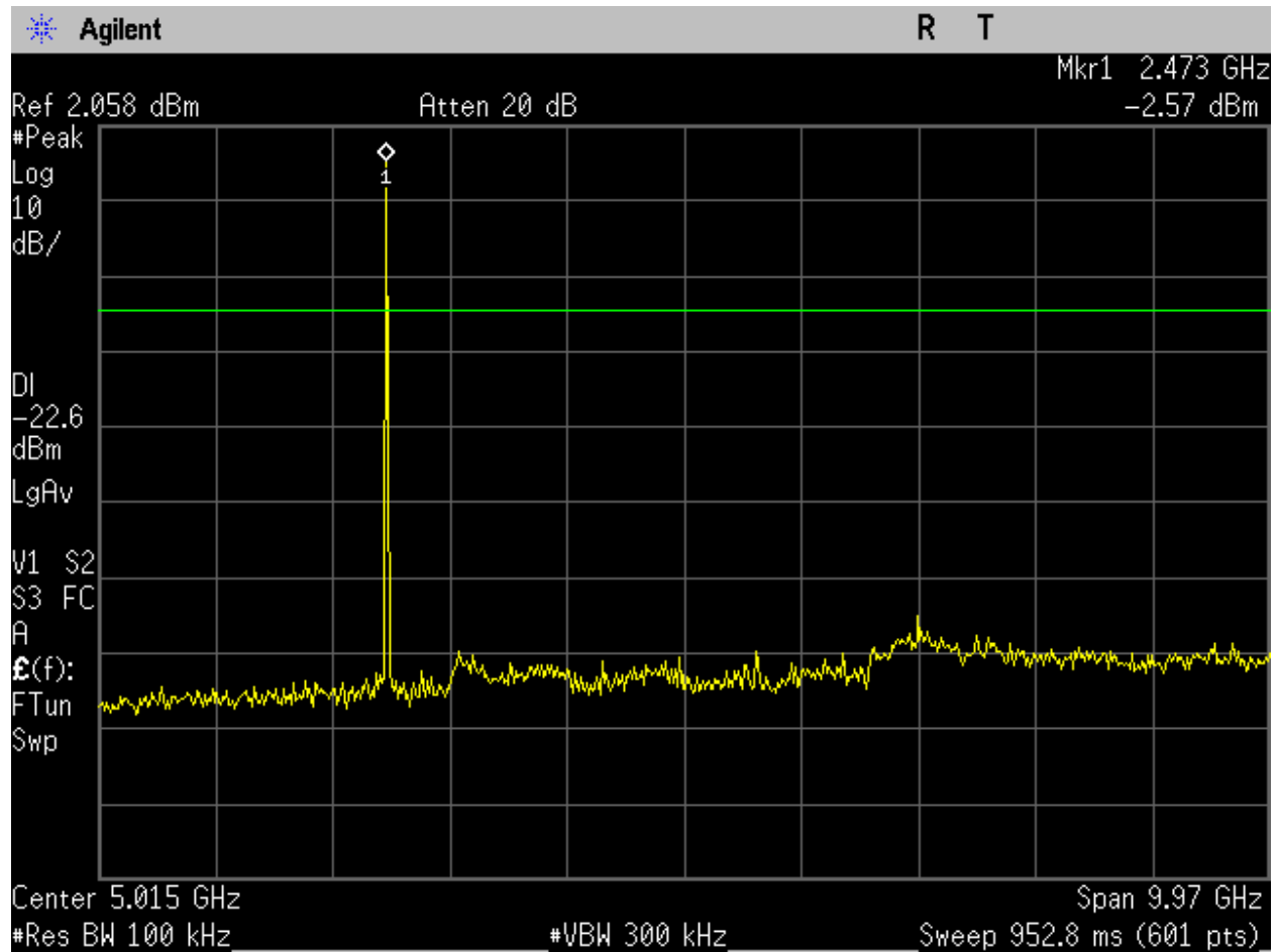
Figure 90. BLE_High Ch_2480MHz_1MBit_-20dBc_30MHz-10GHz_Port 1.
