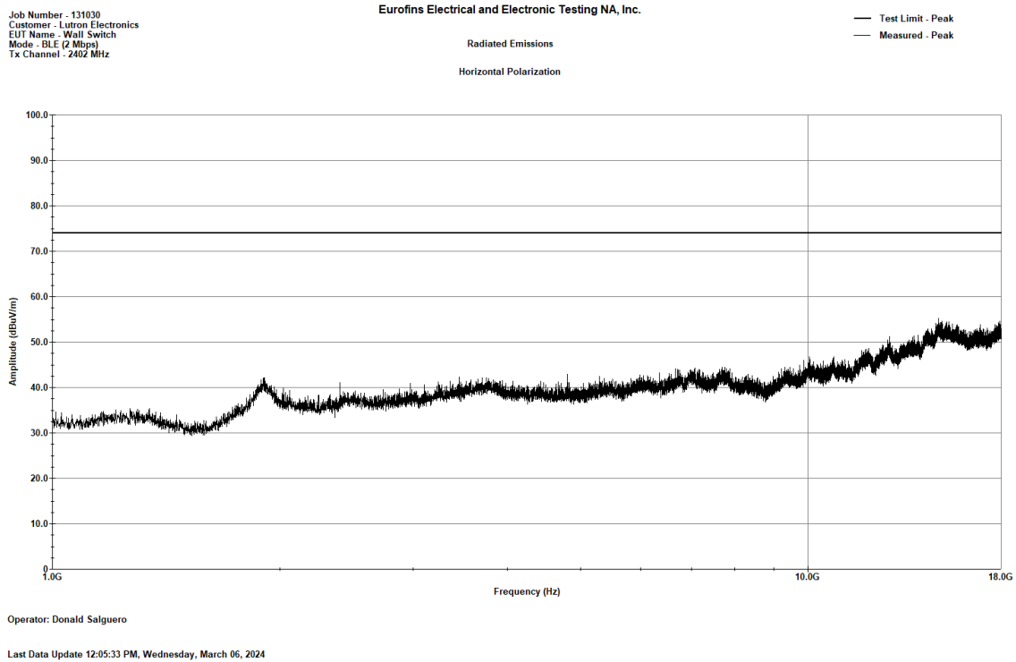
Figure 69. BLE (2 Mbps)_2402MHz_Radiated Emissions, Peak, 1 - 18 GHz-_H
