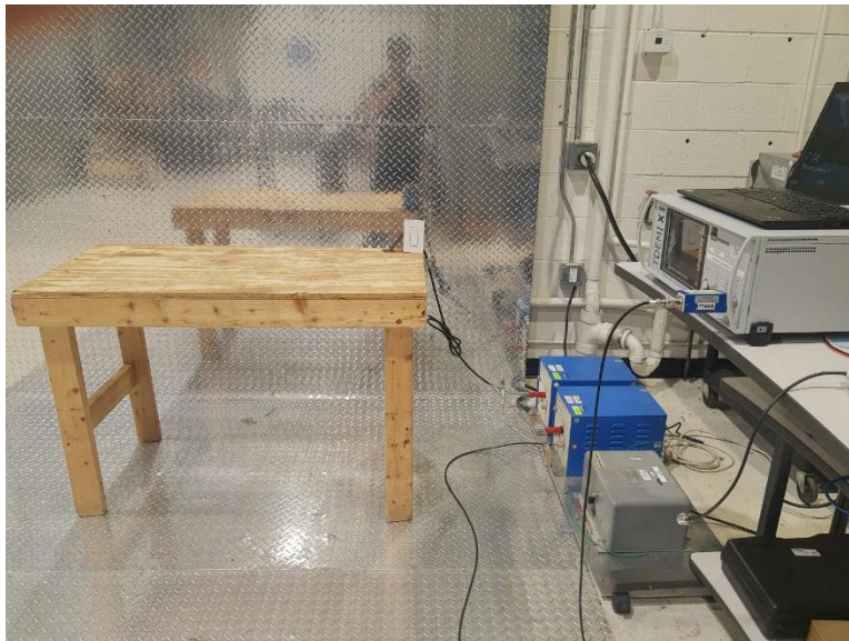
Photograph 2. CE Setup
