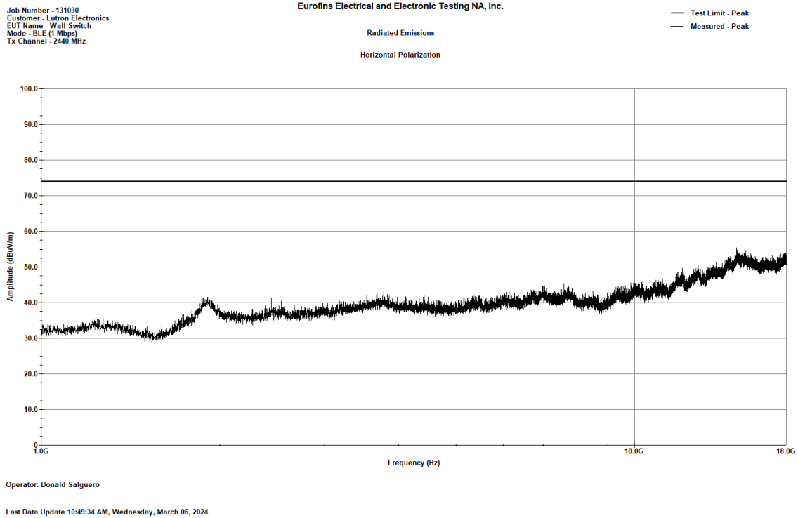
Figure 53. BLE (1 Mbps)_2440MHz_Radiated Emissions, Peak, 1 - 18 GHz-_H
