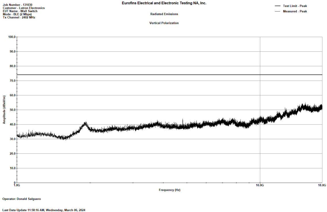
Figure 70. BLE (2 Mbps)_2402MHz_Radiated Emissions, Peak, 1 - 18 GHz-_V
