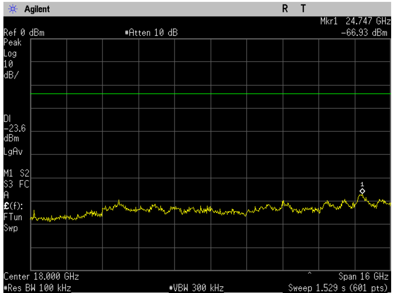
Figure 95. BLE_Low Ch_2402MHz_1MBit_-20dBc_10-26GHz_Port 1.
