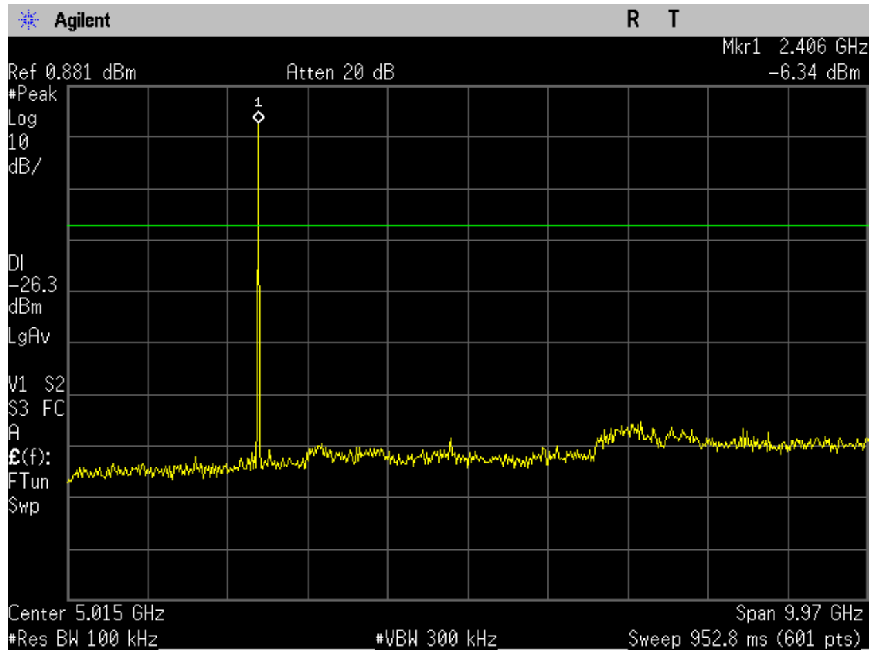
Figure 99. BLE_Low Ch_2402MHz_2MBit_-20dBc_30MHz-10GHz_Port 1.
