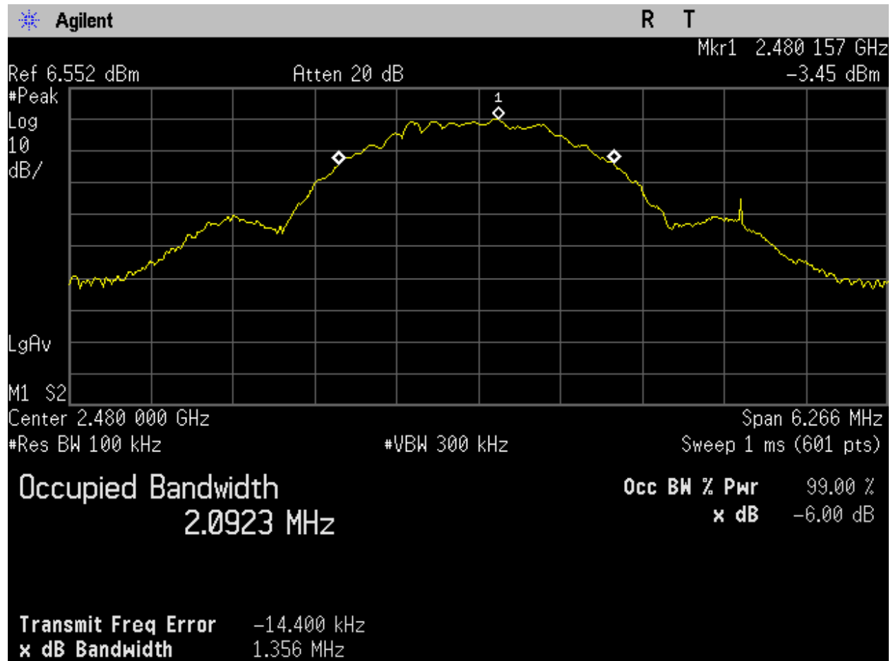
Figure 8. BLE_High Ch_2480MHz_2MBit_Occupied Bandwidth_-6dB_Port 1.
