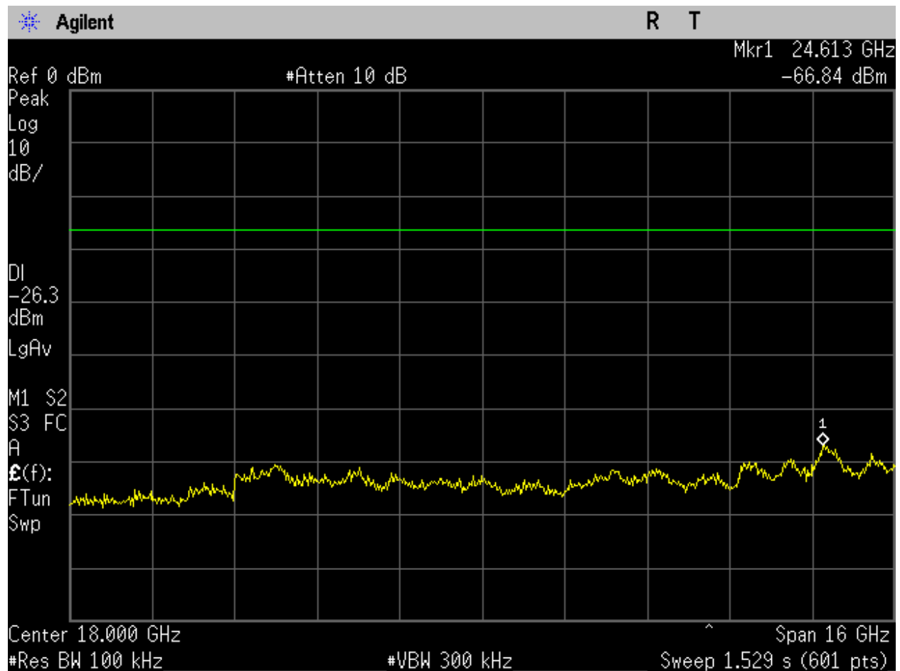
Figure 98. BLE_Low Ch_2402MHz_2MBit_-20dBc_10-26GHz_Port 1.
