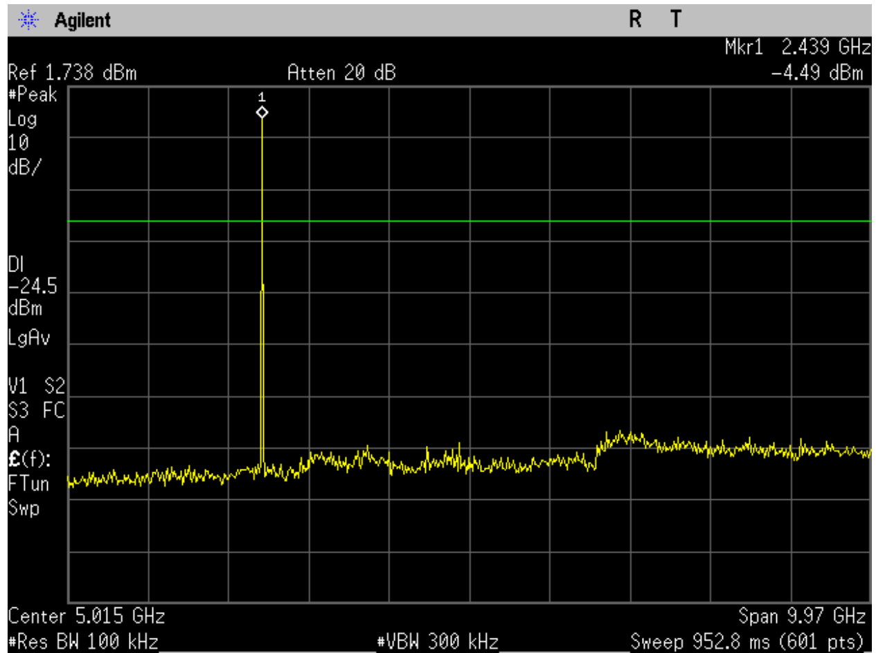
Figure 104. BLE_Mid Ch_2440MHz_2MBit_-20dBc_30MHz-10GHz_Port 1.
