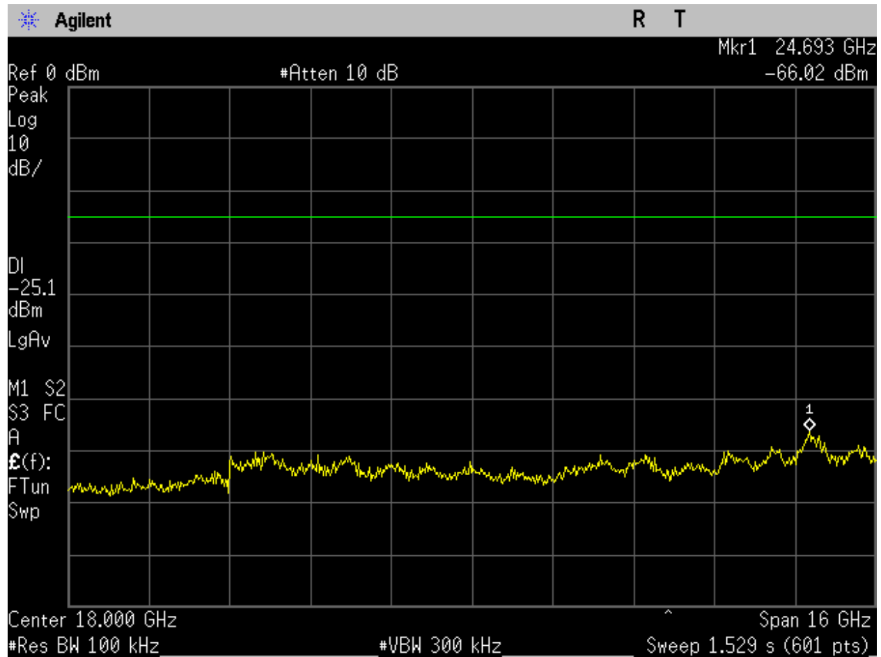
Figure 92. BLE_High Ch_2480MHz_2MBit_-20dBc_10-26GHz_Port 1.
