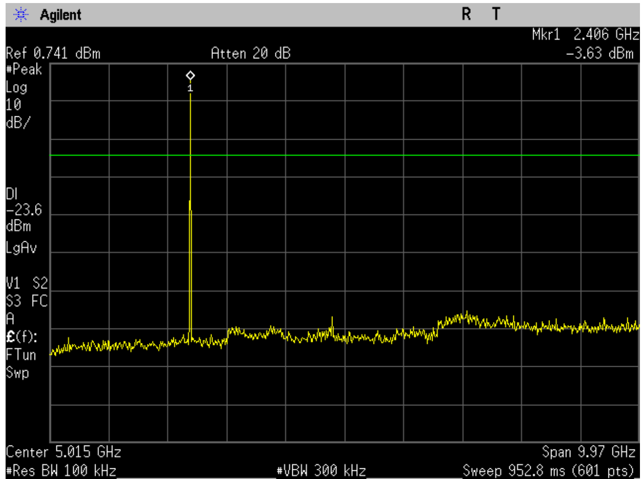
Figure 96. BLE_Low Ch_2402MHz_1MBit_-20dBc_30MHz-10GHz_Port 1.
