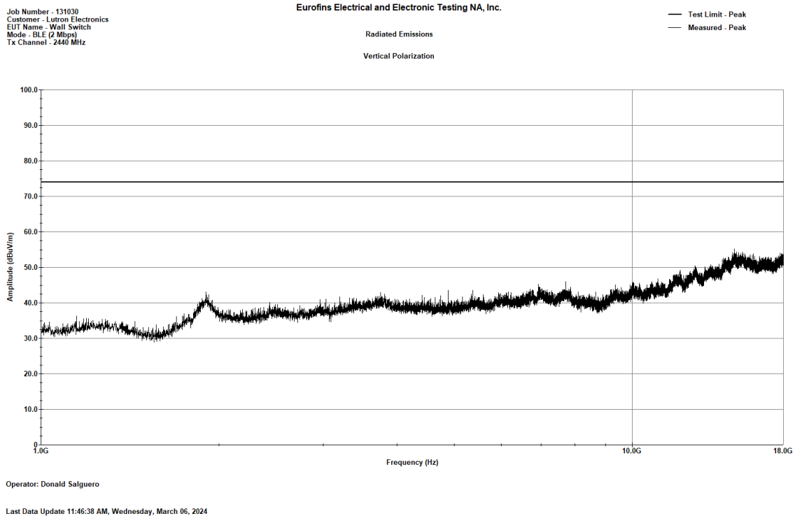
Figure 76. BLE (2 Mbps)_2440MHz_Radiated Emissions, Peak, 1 - 18 GHz-_V
