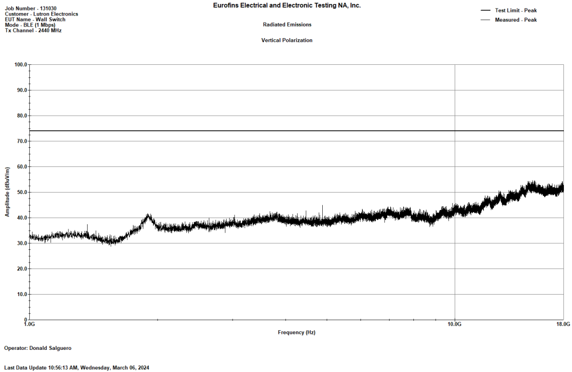
Figure 54. BLE (1 Mbps)_2440MHz_Radiated Emissions, Peak, 1 - 18 GHz-_V
