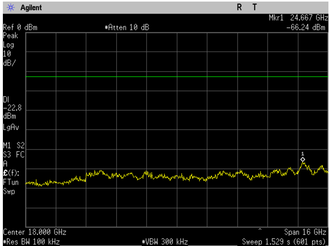
Figure 101. BLE_Mid Ch_2440MHz_1MBit_-20dBc_10-26GHz_Port 1.
