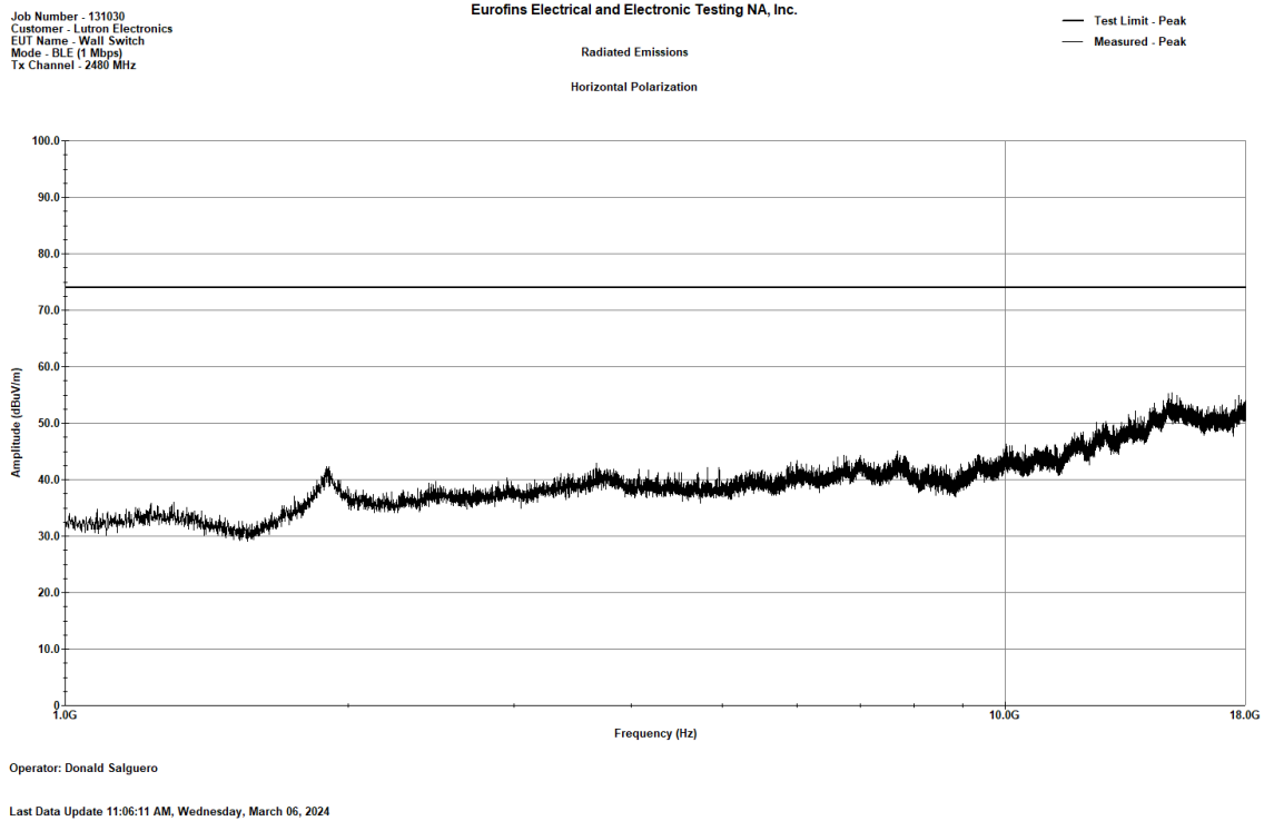
Figure 59. BLE (1 Mbps)_2480MHz_Radiated Emissions, Peak, 1 - 18 GHz-_H
