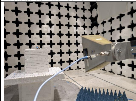
Radiated Spurious Emission- Above 1GHz - BVBRLC-LP-AT
