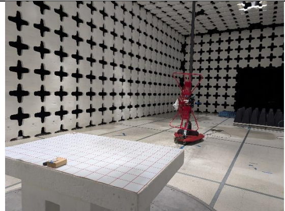
Radiated Spurious Emission-Below 1GHz-Back- BVBRLC-LP-AT
