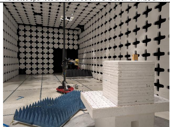
Radiated Spurious Emission- Above 1GHz-Back- BVBRLC-LP-AT
