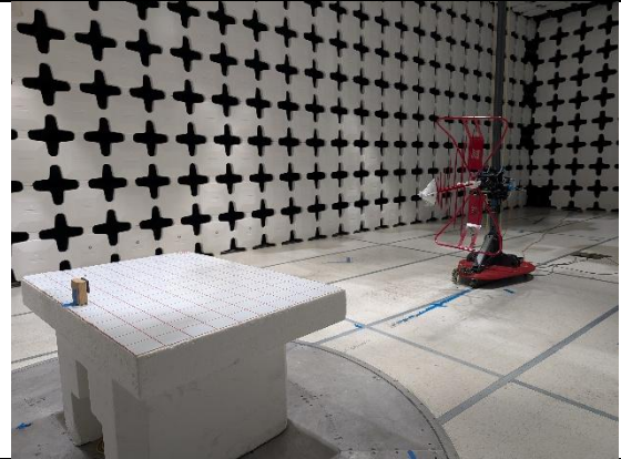
Radiated Spurious Emission-Below 1GHz-Back- BVBRLC-DB
