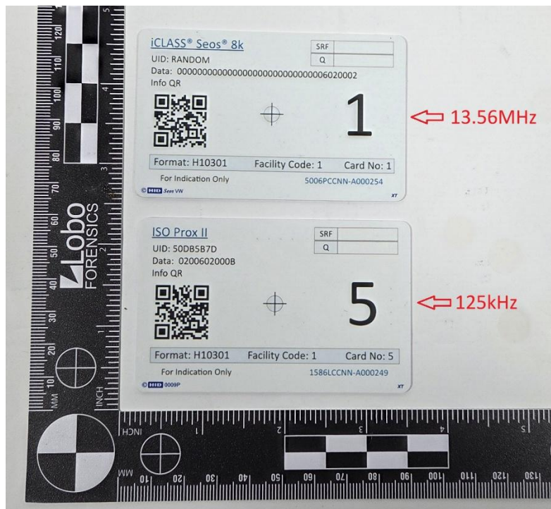
Tags/Credentials_Bottom_125kHz and 13.56MHz (used with OMNIKEY Readers)
