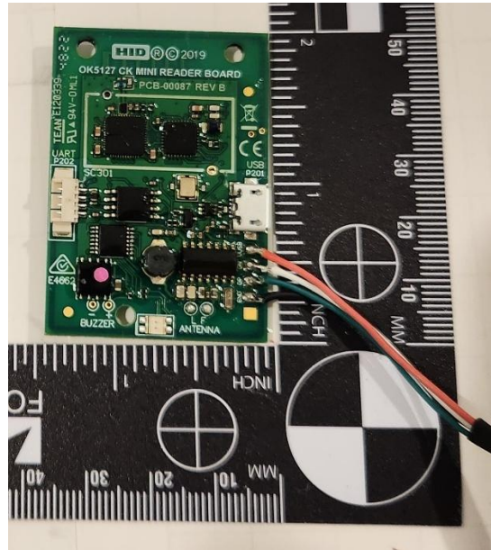
OMNIKEY 5127CK MINI_RF Shield Removed_Top Side
