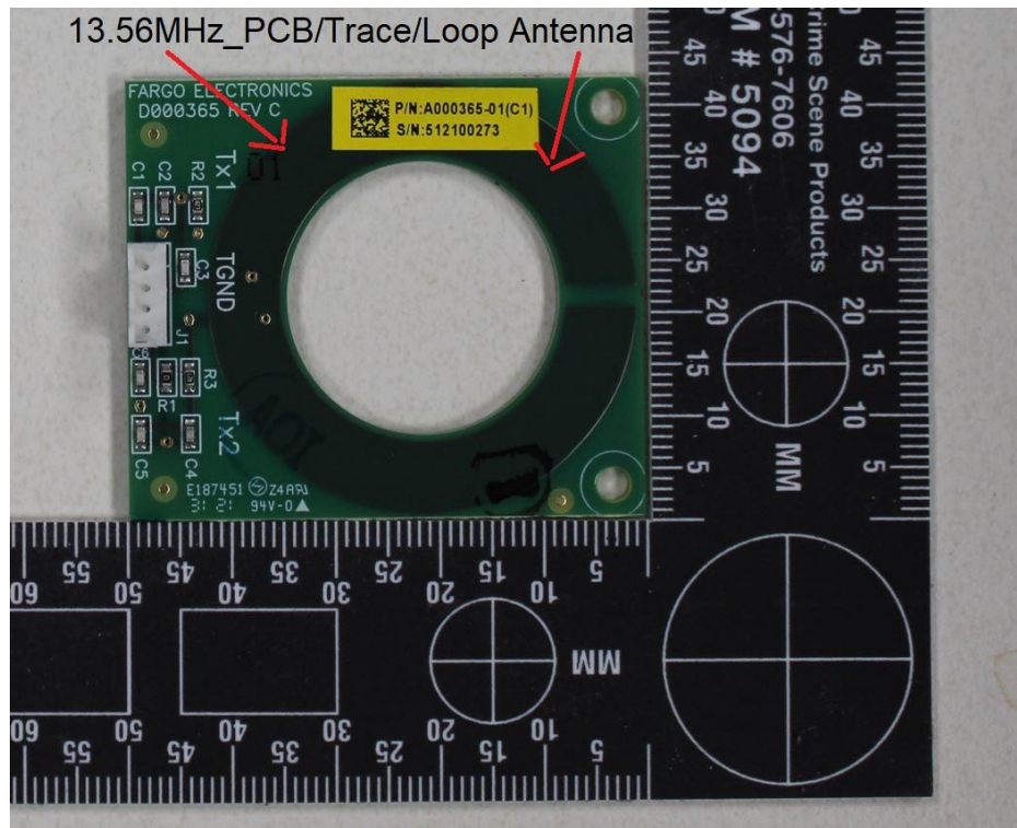
Ribbon RFID_PCB Antenna_Top Side
