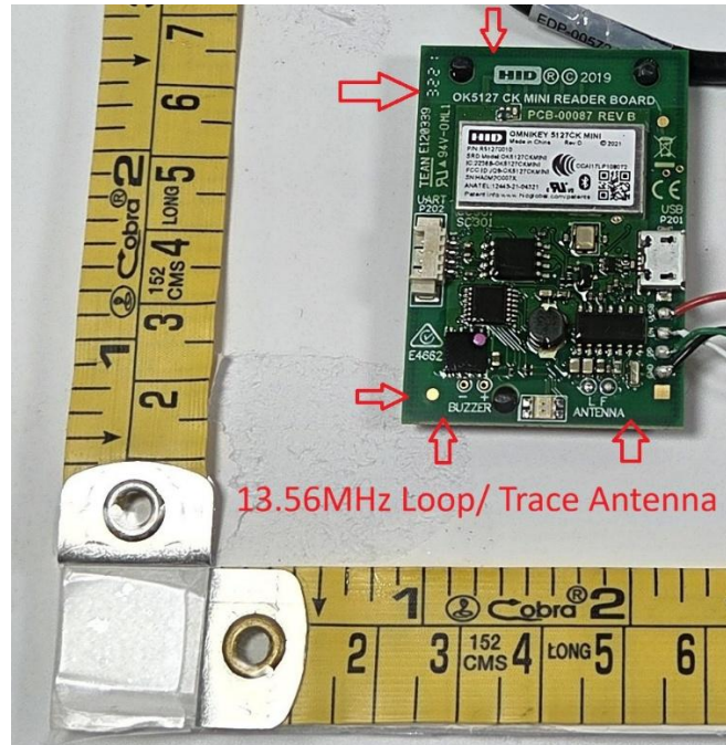
OMNIKEY 5127CK MINI Encoder_HF Antenna Location_Top Side
