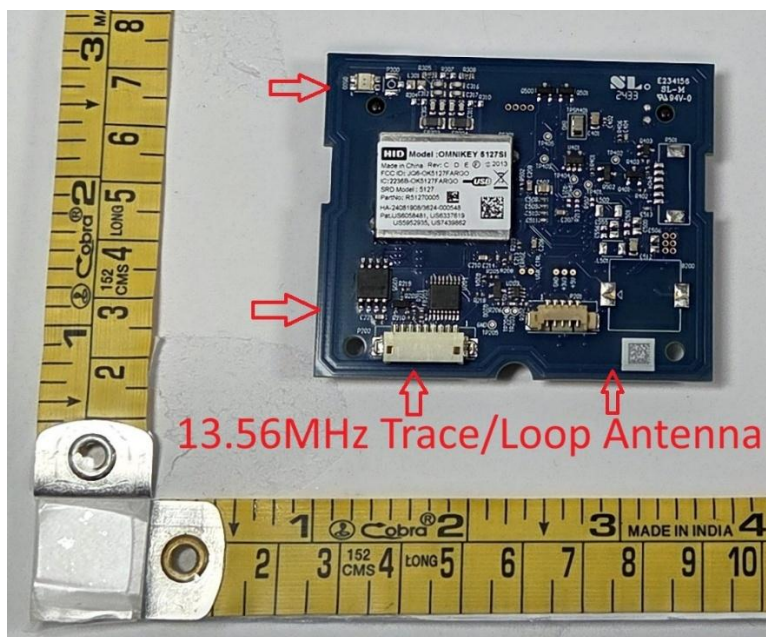
OMNIKEY 5127SI Encoder_HF Antenna Location_Top Side
