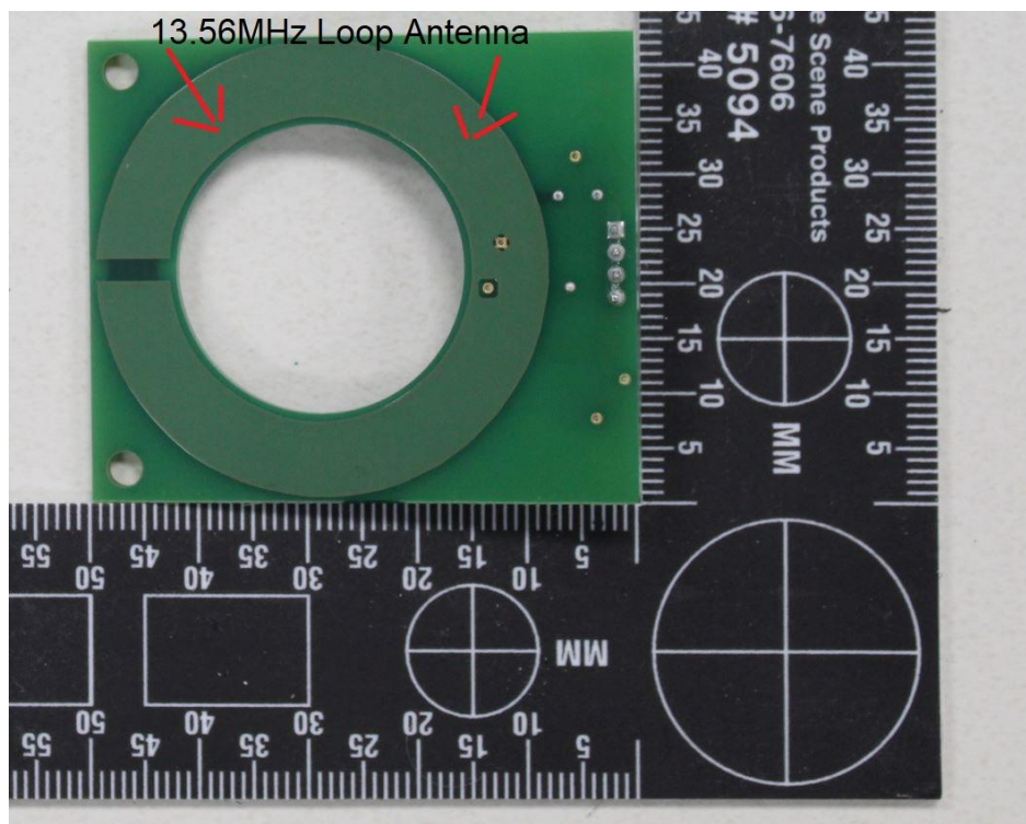
Ribbon RFID_PCB Antenna_Bottom Side
