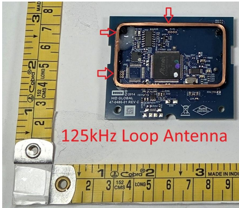
OMNIKEY 5127SI Encoder_LF Antenna Location_Bottom Side
