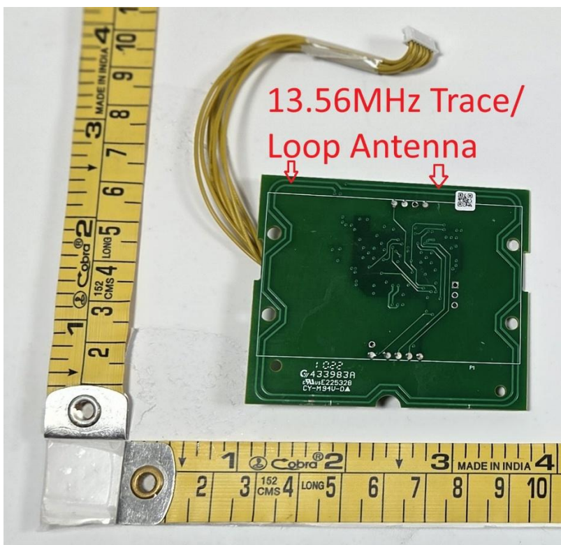
OMNIKEY 5122 Encoder_HF Antenna Location_Bottom Side
