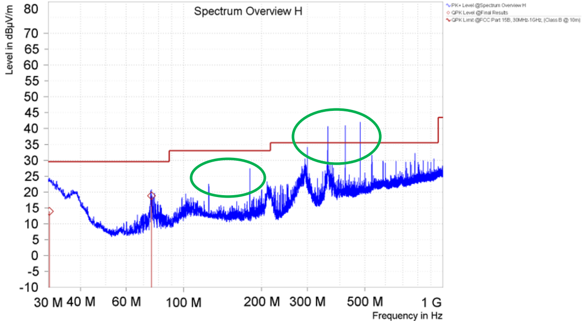
Figure 9. Spurious Emissions 30MHz – 1GHz, Horizontal (5127SI) 3
