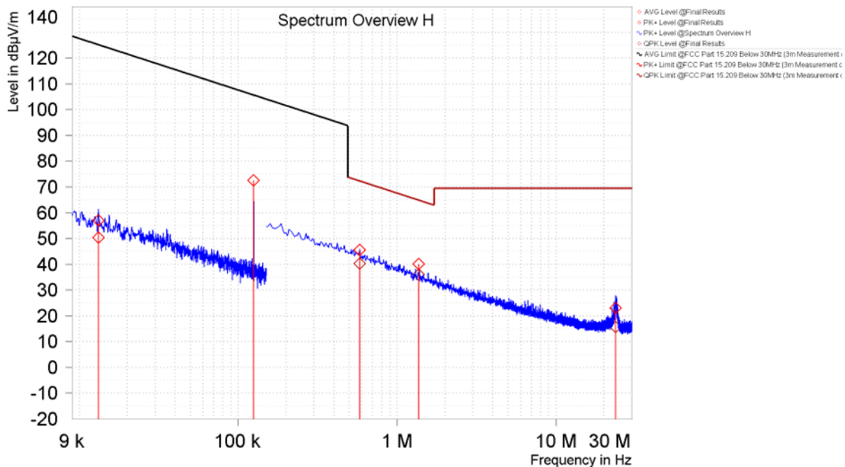
Figure 15. Spurious Emissions Below 30MHz, Coaxial Loop (CK MINI)
