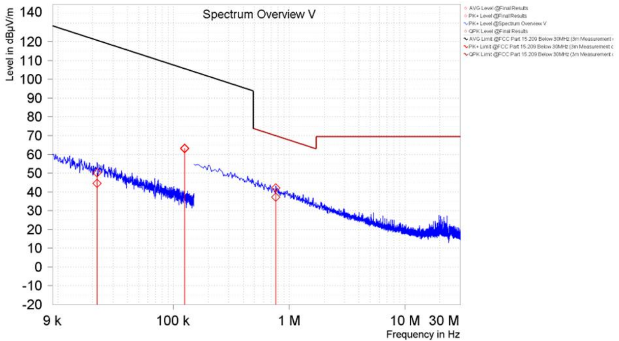
Figure 6. Spurious Emissions Below 30MHz, Coplanar Loop, (5127SI)
