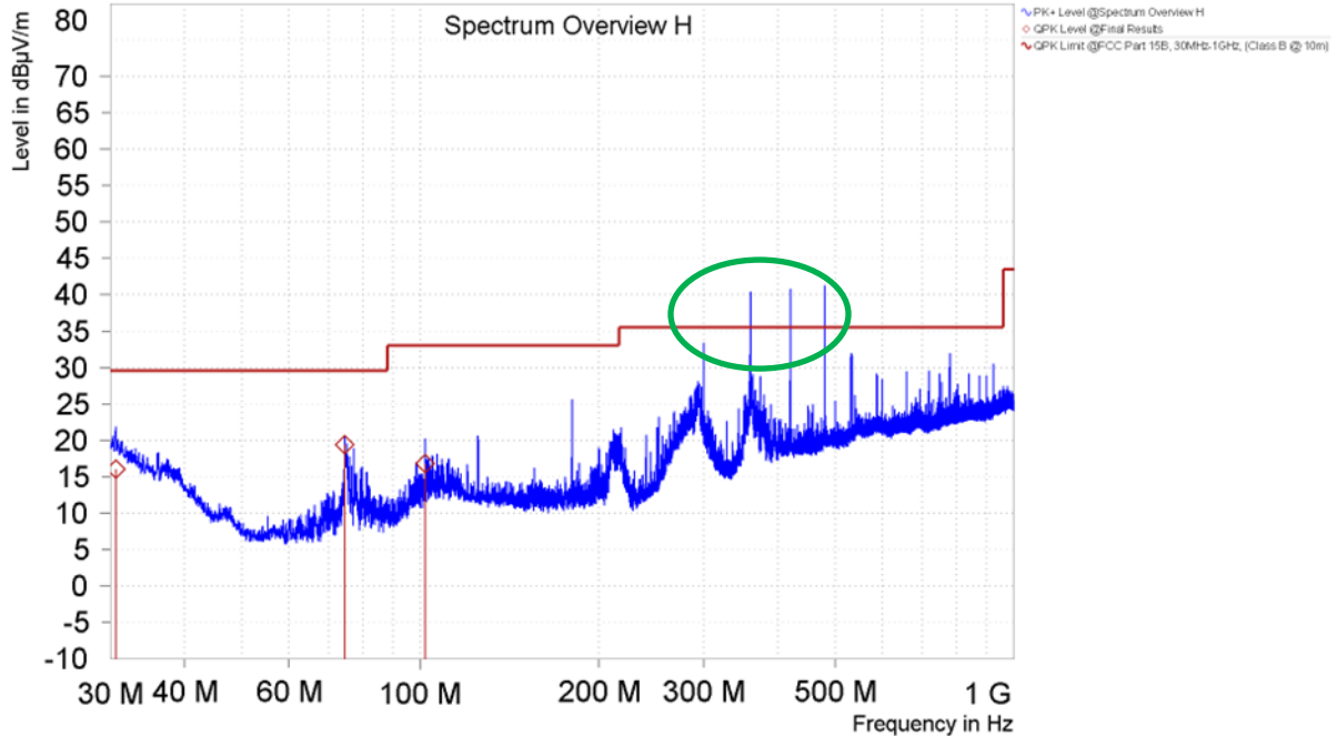
Figure 13. Spurious Emissions 30MHz – 1GHz, Horizontal (5127SI, Without Credential) 6
