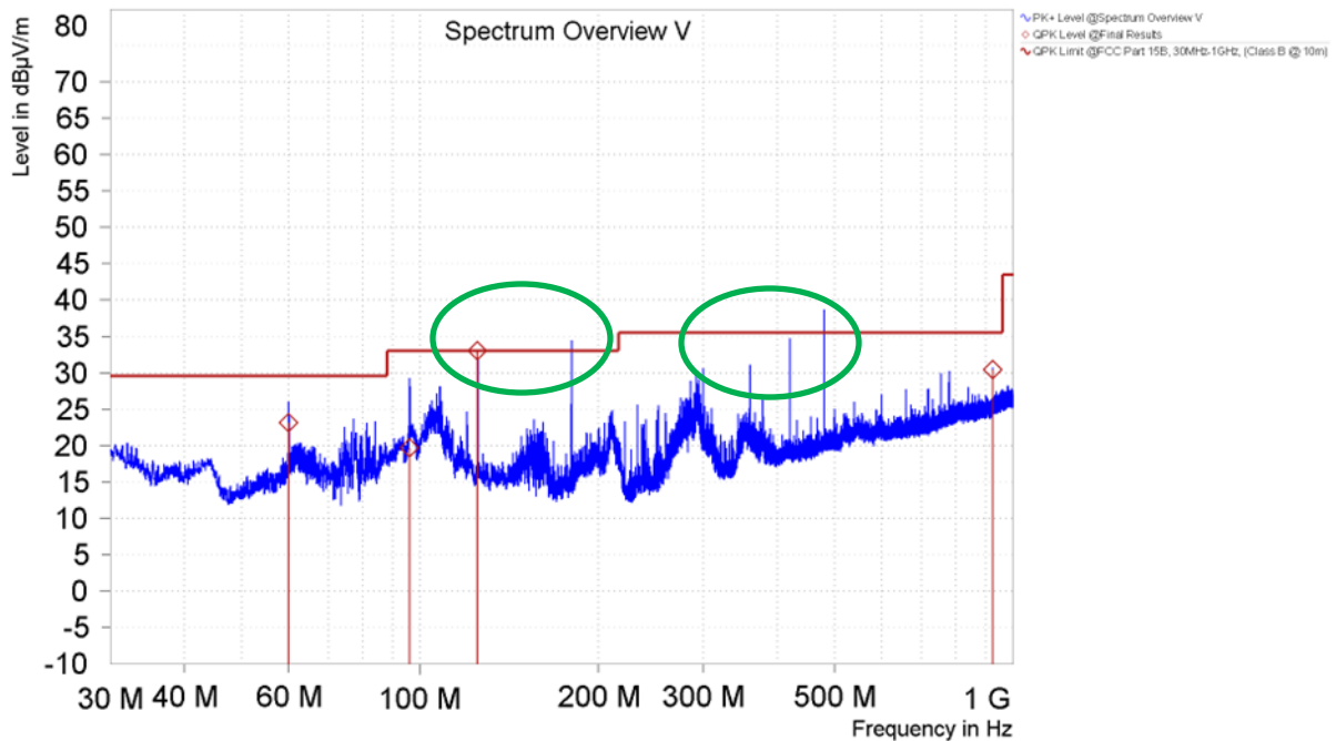
Figure 20. Spurious Emissions 30MHz – 1GHz, Vertical (CK MINI, Without Credential) 12
