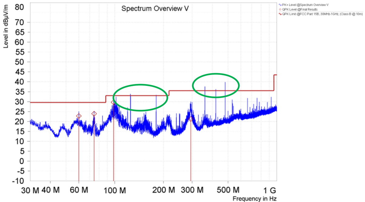
Figure 12. Spurious Emissions 30MHz – 1GHz, Vertical (5127SI, Without Credential) 6
