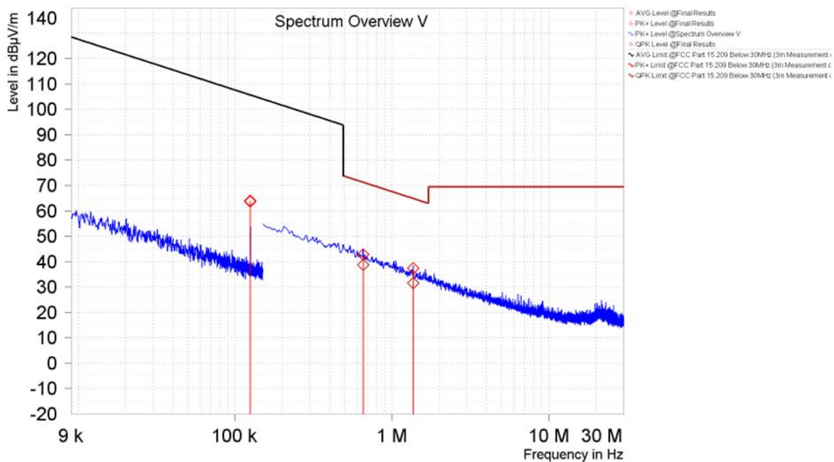
Figure 14. Spurious Emissions Below 30MHz, Coplanar Loop, (CK MINI)
