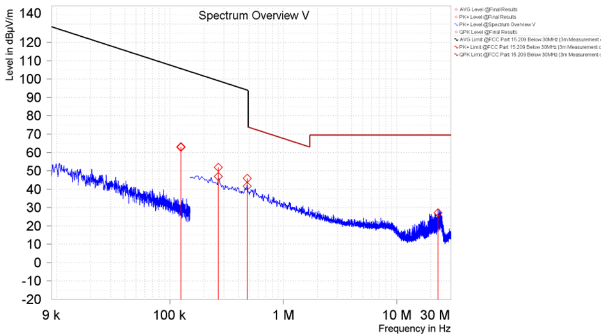
Figure 10. Spurious Emissions Below 30MHz, Coplanar Loop, (5127SI, Without Credential)
