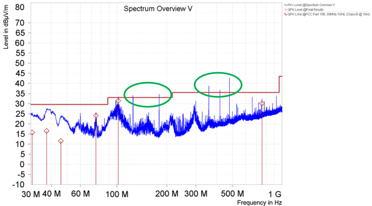
Figure 8. Spurious Emissions 30MHz – 1GHz, Vertical (5127SI) 3
