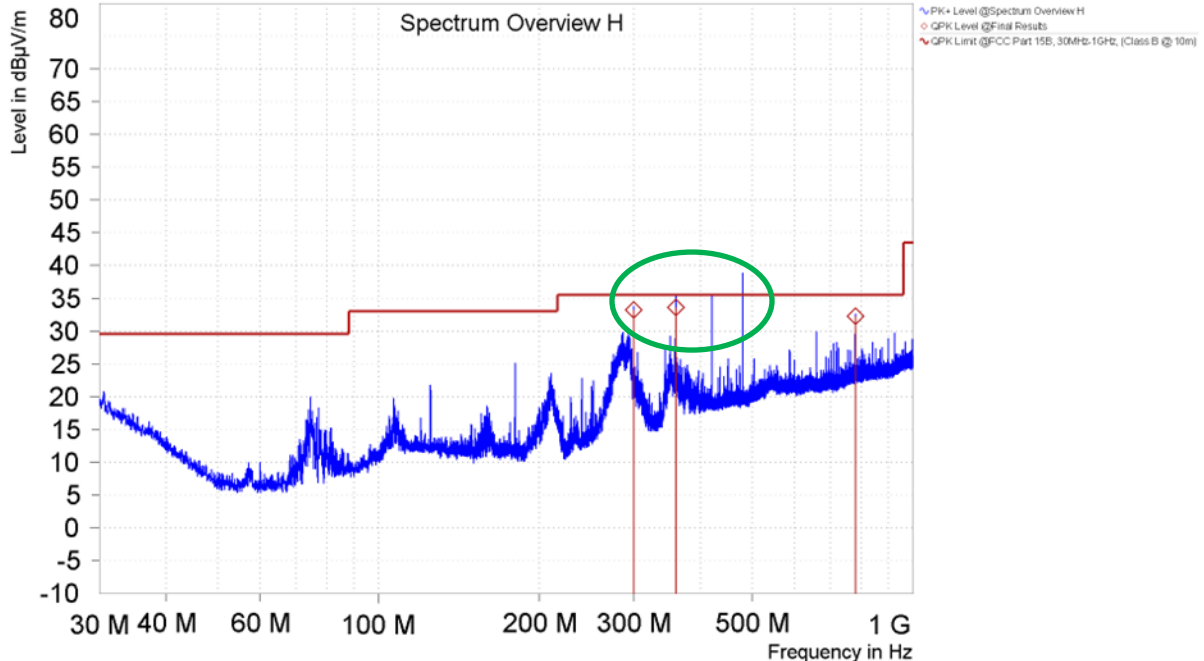
Figure 17. Spurious Emissions 30MHz – 1GHz, Horizontal (CK MINI) 9
