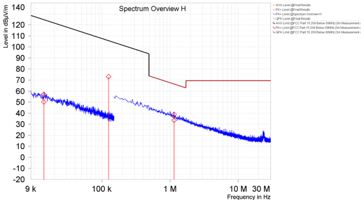
Figure 7. Spurious Emissions Below 30MHz, Coaxial Loop (5127SI)
