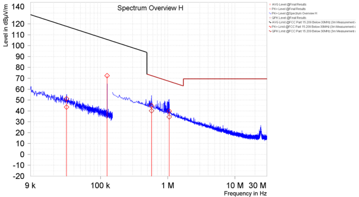
Figure 19. Spurious Emissions Below 30MHz, Coaxial Loop (CK MINI, Without Credential)
