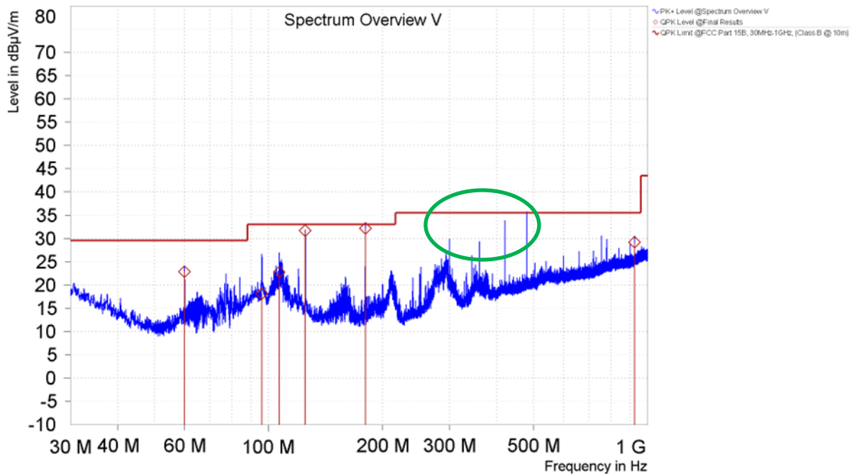
Figure 16. Spurious Emissions 30MHz – 1GHz, Vertical (CK MINI) 9
