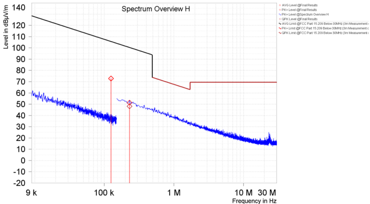
Figure 11. Spurious Emissions Below 30MHz, Coaxial Loop (5127SI, Without Credential)
