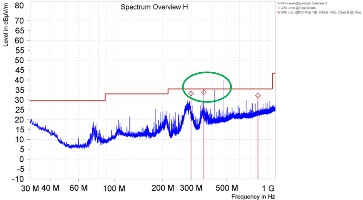
Figure 21. Spurious Emissions 30MHz – 1GHz, Horizontal (CK MINI, Without Credential) 12
