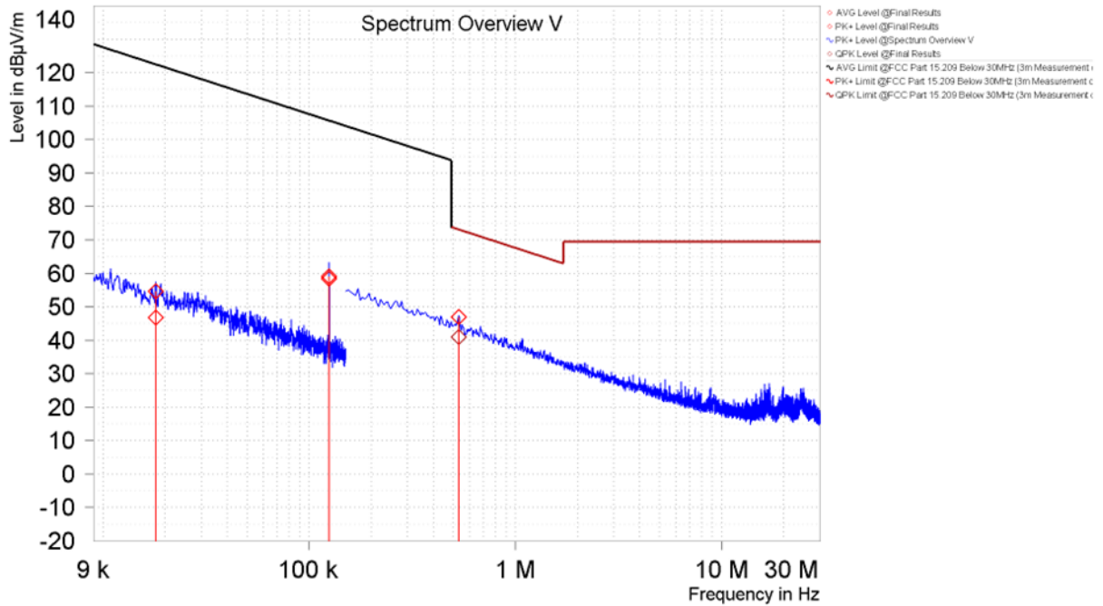
Figure 18. Spurious Emissions Below 30MHz, Coplanar Loop, (CK MINI, Without Credential)
