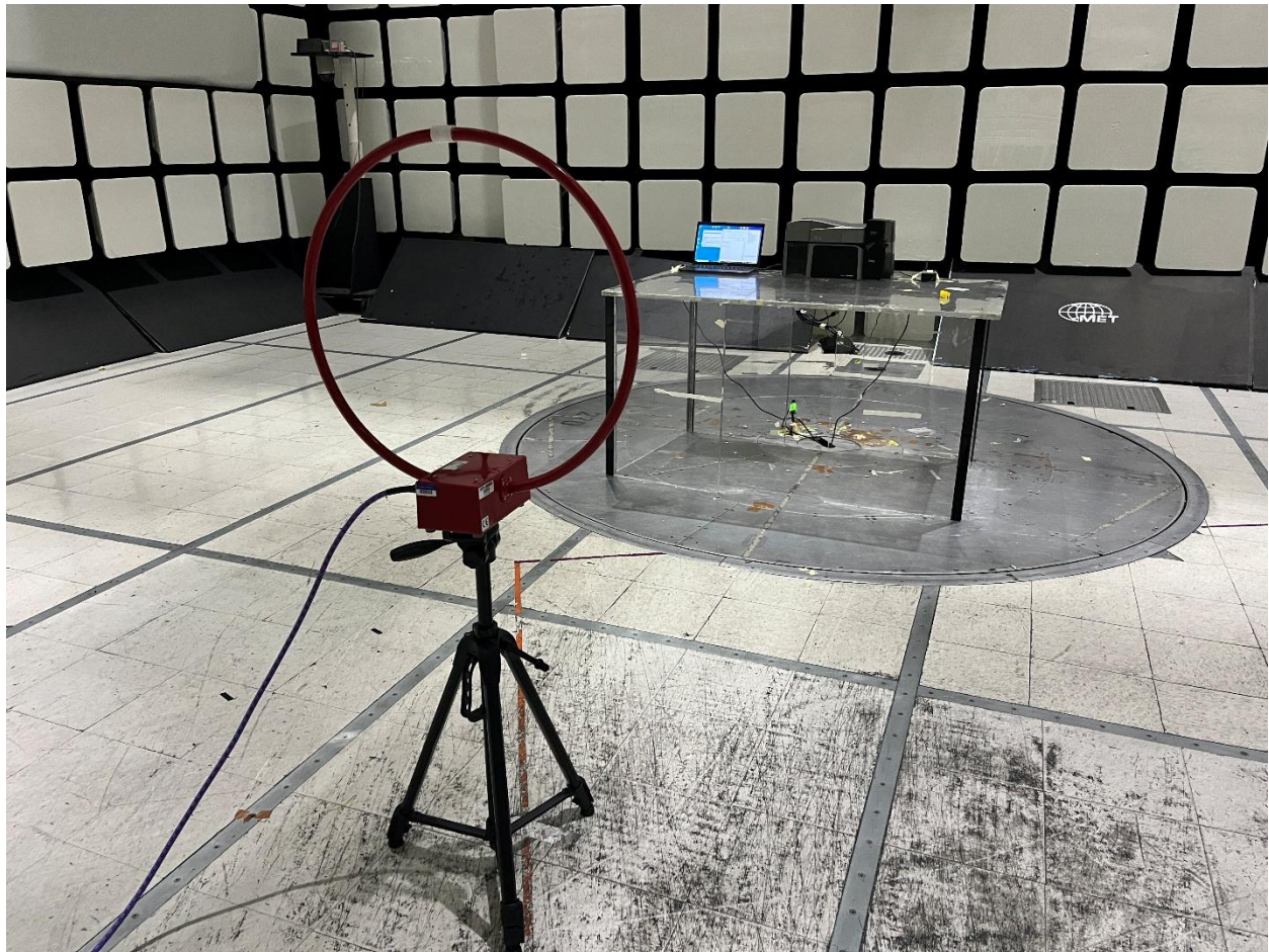
Radiated Emissions Below 30MHz (Front Side)
