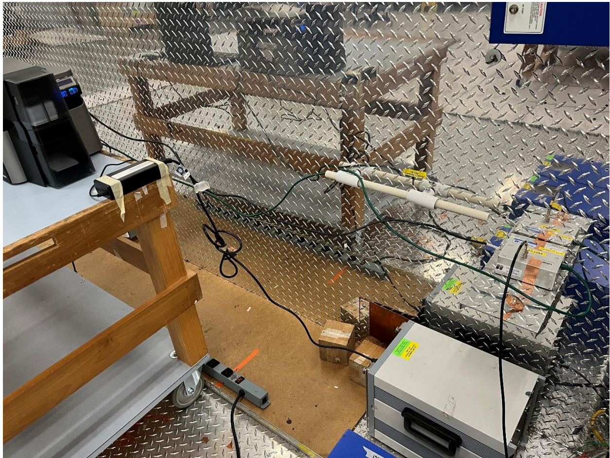
Conducted Emissions (LISN)
