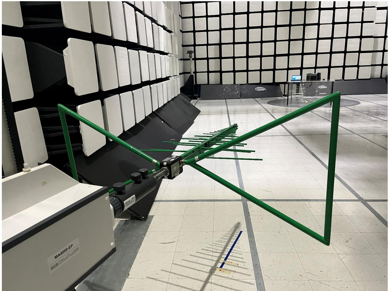
Radiated Emissions 30MHz – 1GHz (Front Side)
