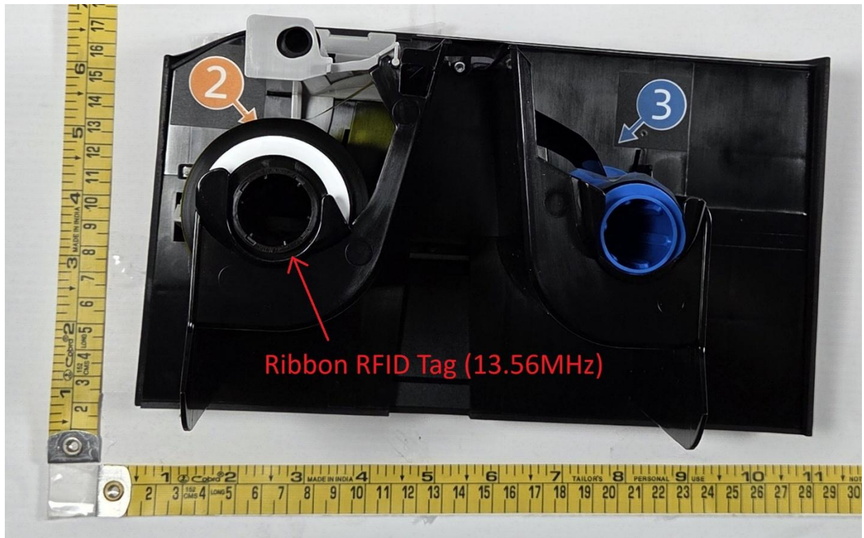
Ribbon Cartridge_RFID Tag
