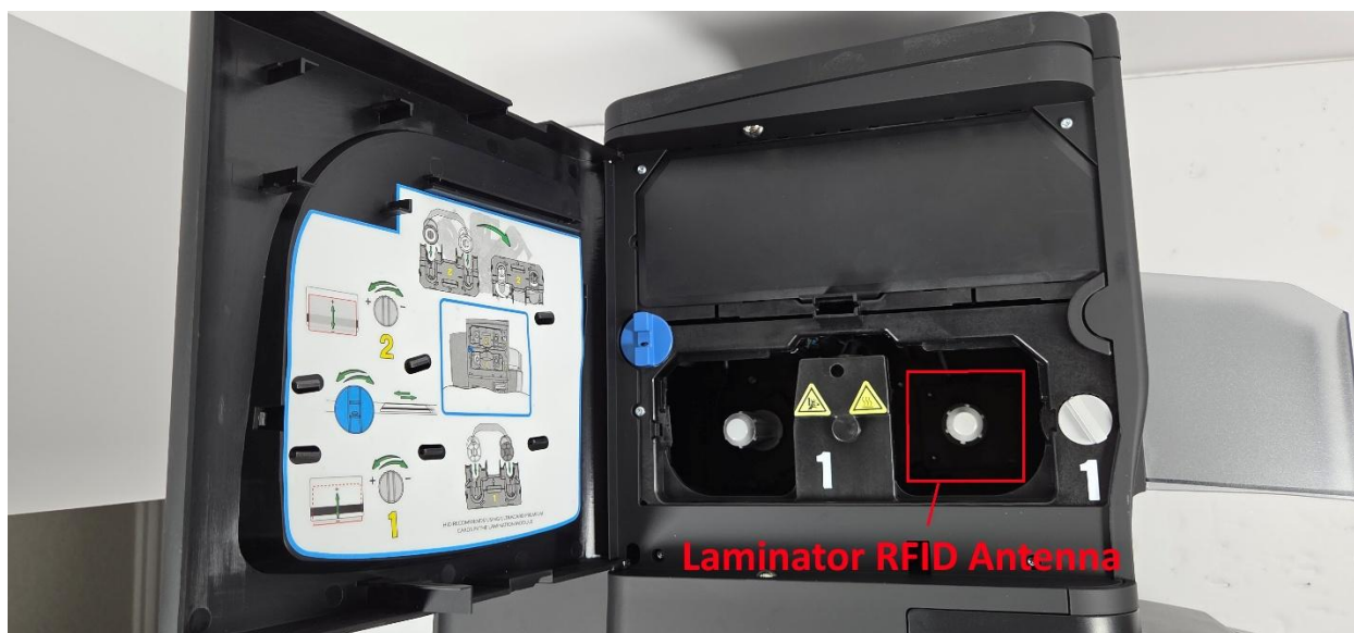
Laminator RFID Antenna Location
