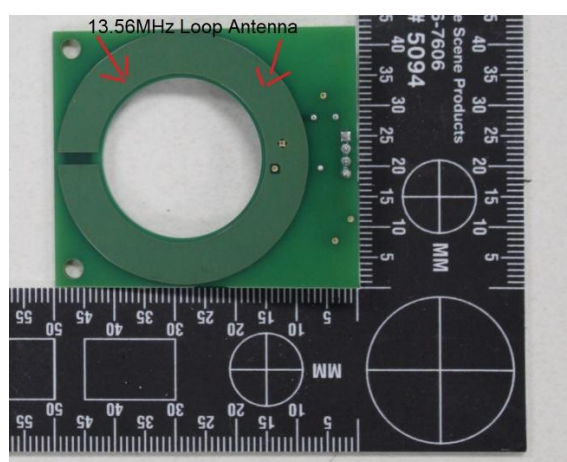
Laminator RFID Antenna _Bottom Side
