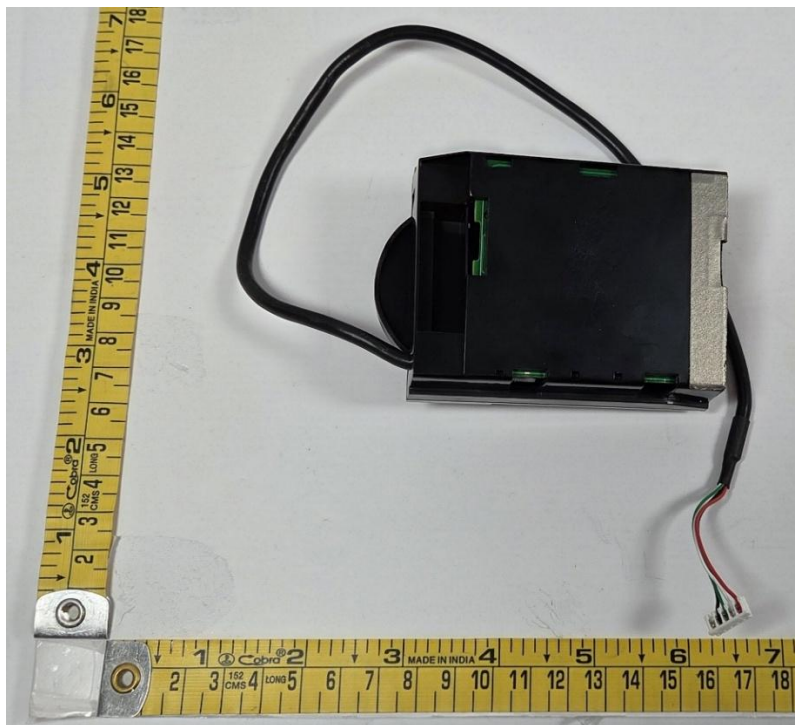
OMNIKEY (5122, 5127SI, 5127CK MINI) Housing_Bottom Side
