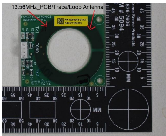
Laminator RFID Antenna _Top Side
