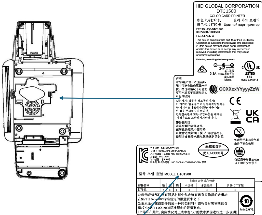
Bottom side of DTC1500
