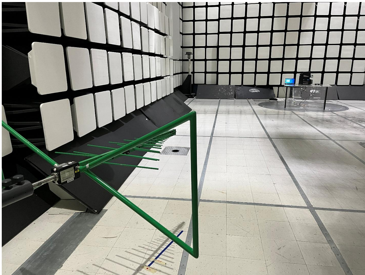
Radiated Emissions Antenna Side – 30MHz – 1GHz
