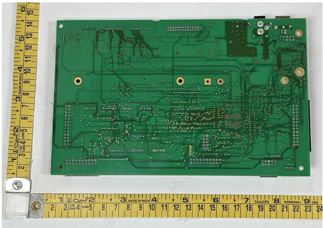
Printer_Main Control Board_Bottom Side
