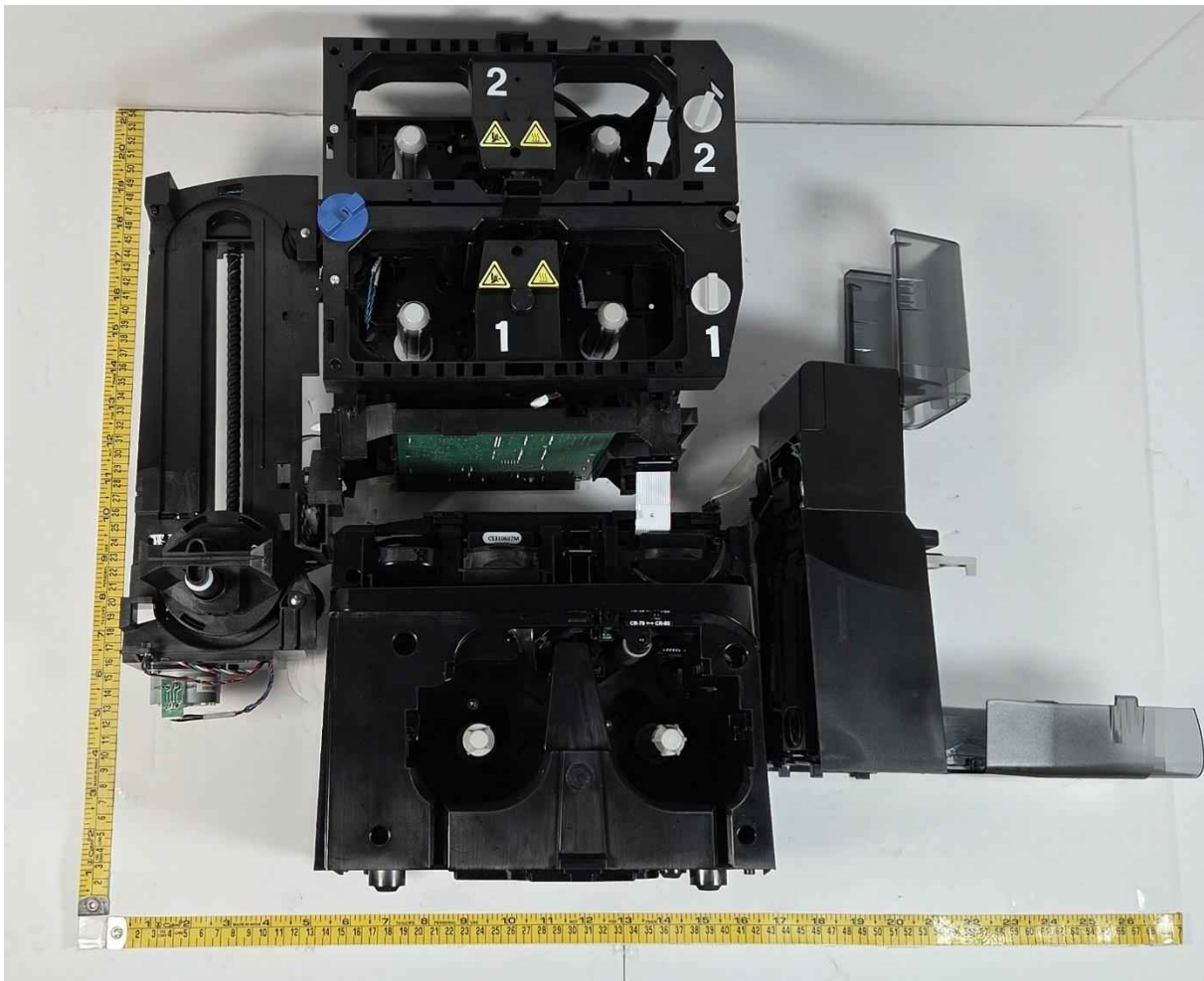
Full Sytem_Covers Removed_Front/Top Side
