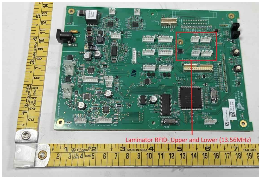
Laminator RFID Chip Location
