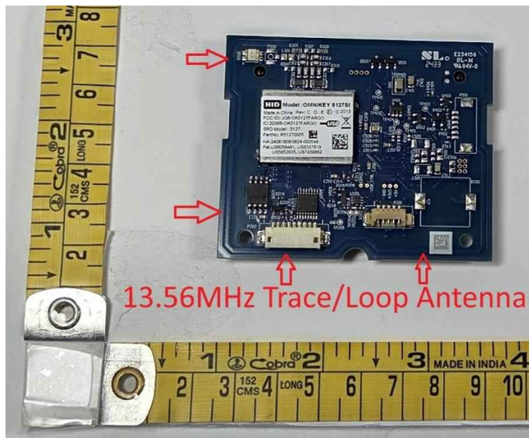
OMNIKEY 5127SI_HF Antenna Location_Top Side
