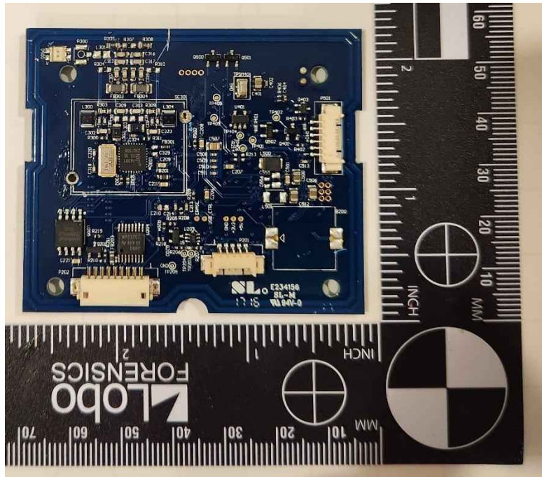
OMNIKEY 5127SI_RF Shield Removed_Top Side
