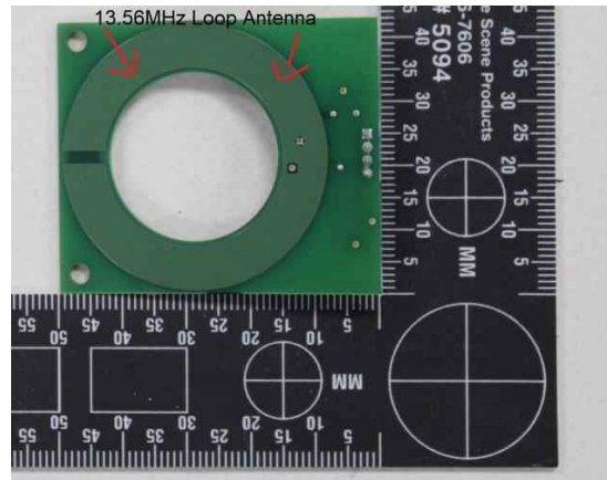
Ribbon RFID Antenna_Bottom Side
