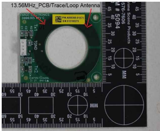
Laminator Lower RFID Antenna_Top Side
