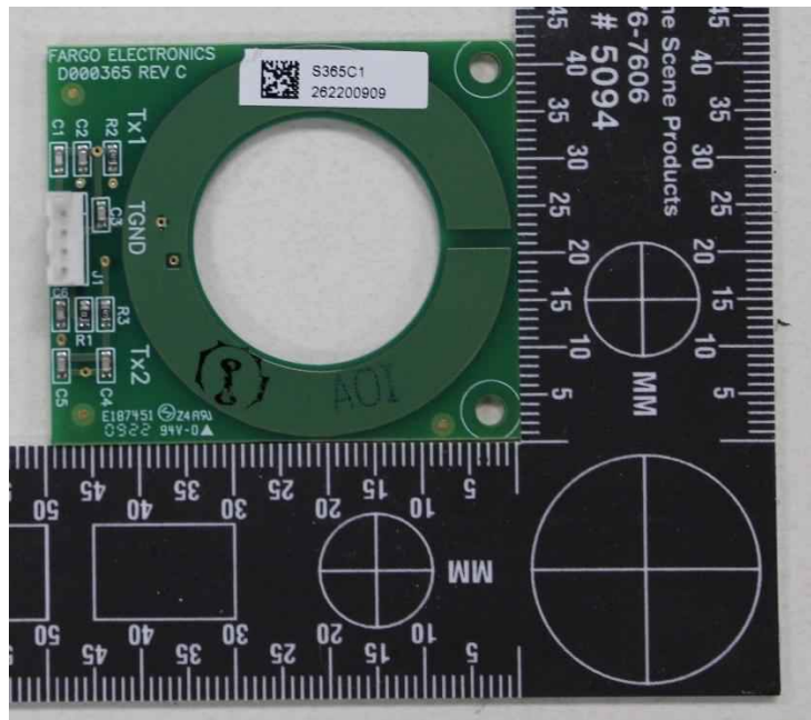
Ribbon PCB Antenna_Top Side
