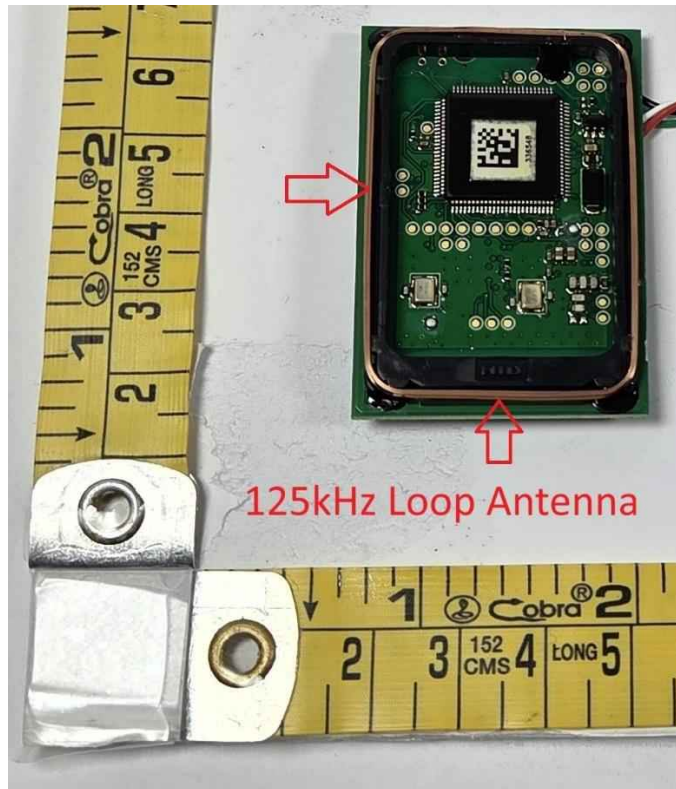
OMNIKEY 5127CK MINI_LF Antenna Location_Bottom Side
