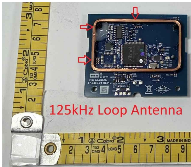
OMNIKEY 5127SI_LF Antenna Location_Bottom Side
