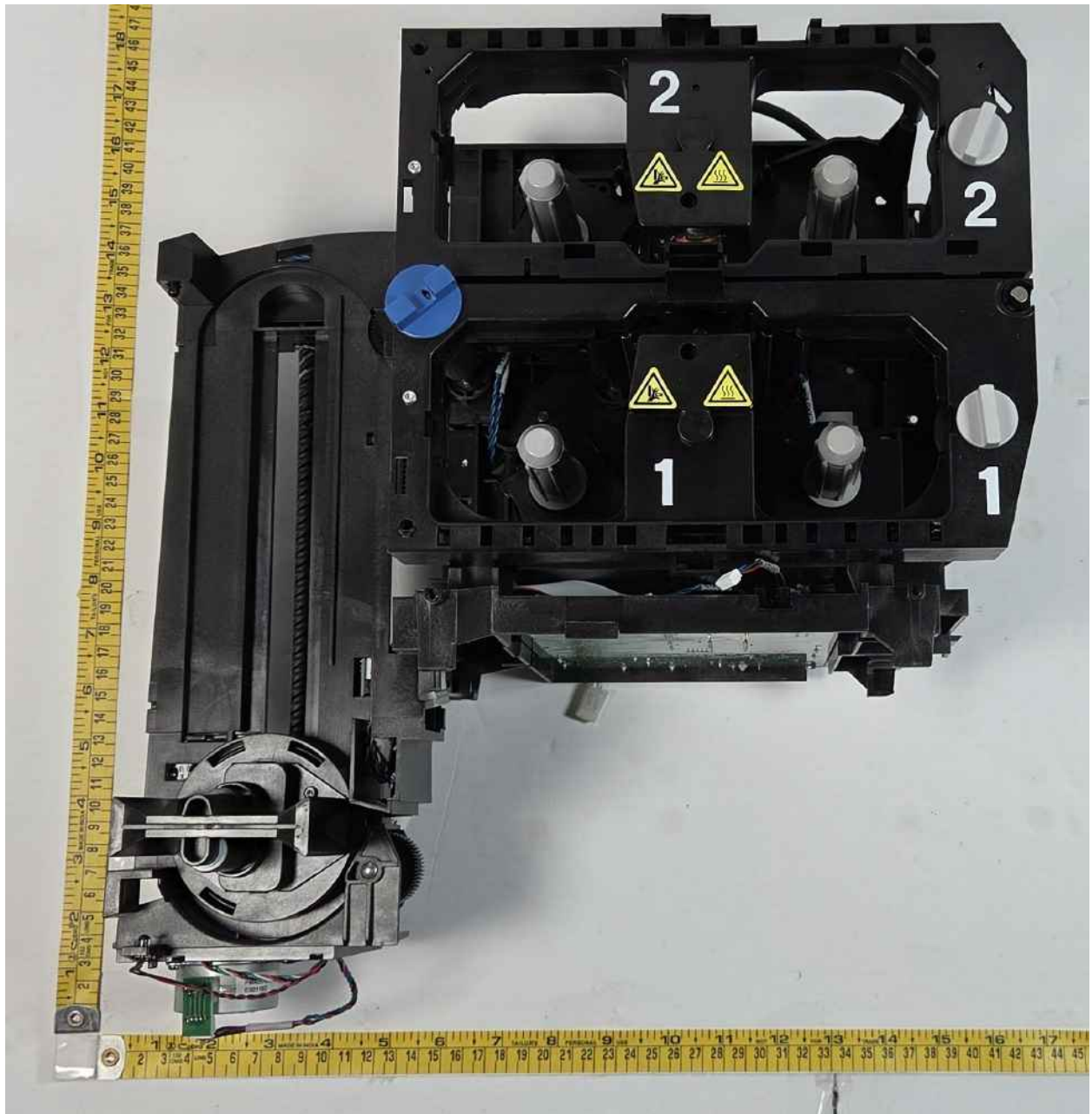
Laminator/Flipper_Covers Removed_Front Side
