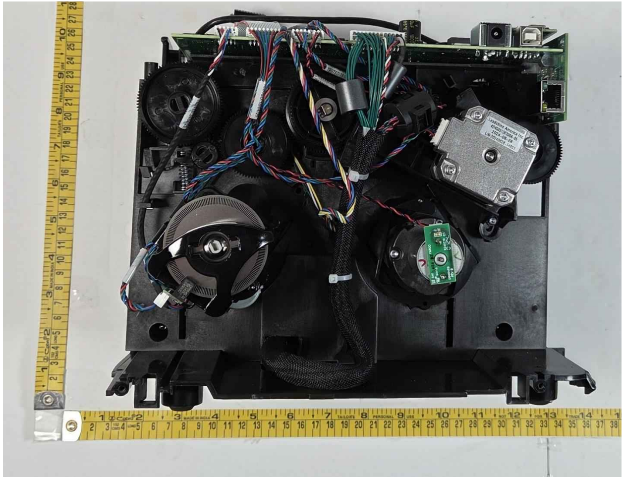
Printer_Covers Removed _Back Side
