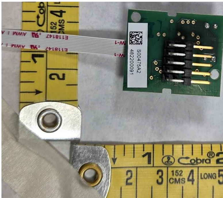
Contact Encoder Board_Bottom Side
