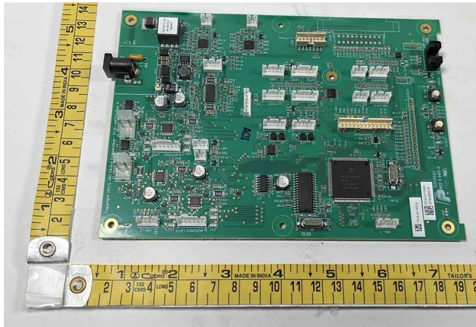
Laminator Control Board_Top Side
