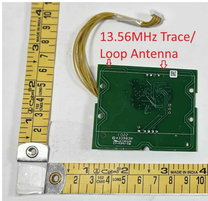
OMNIKEY 5122_HF Antenna Location_Bottom Side
