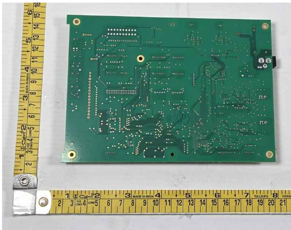
Laminator Control Board_Bottom Side
