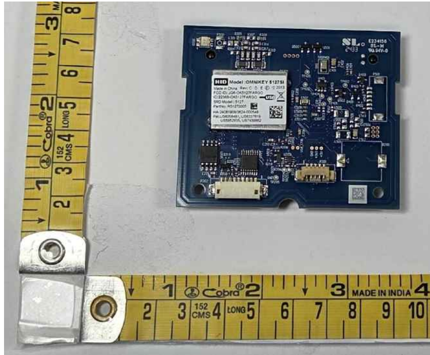
OMNIKEY 5127SI Encoder_Top Side
