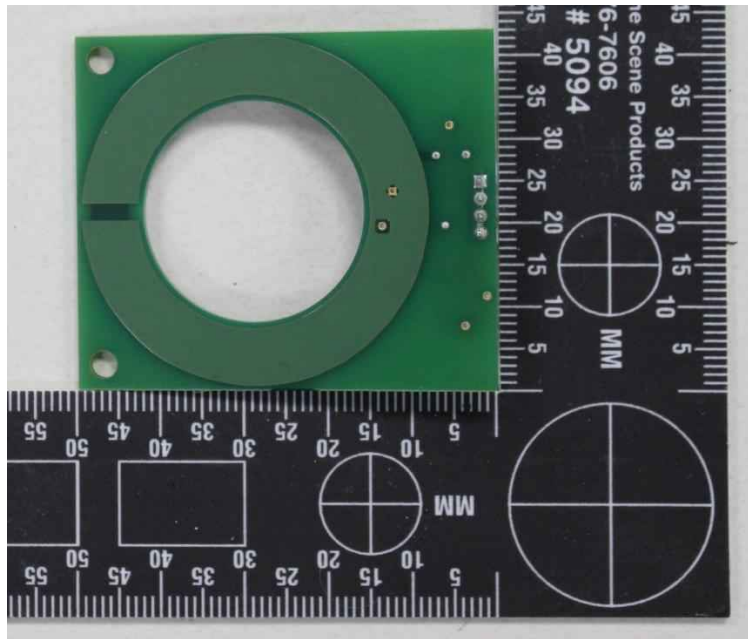
Ribbon PCB Antenna_Bottom Side
