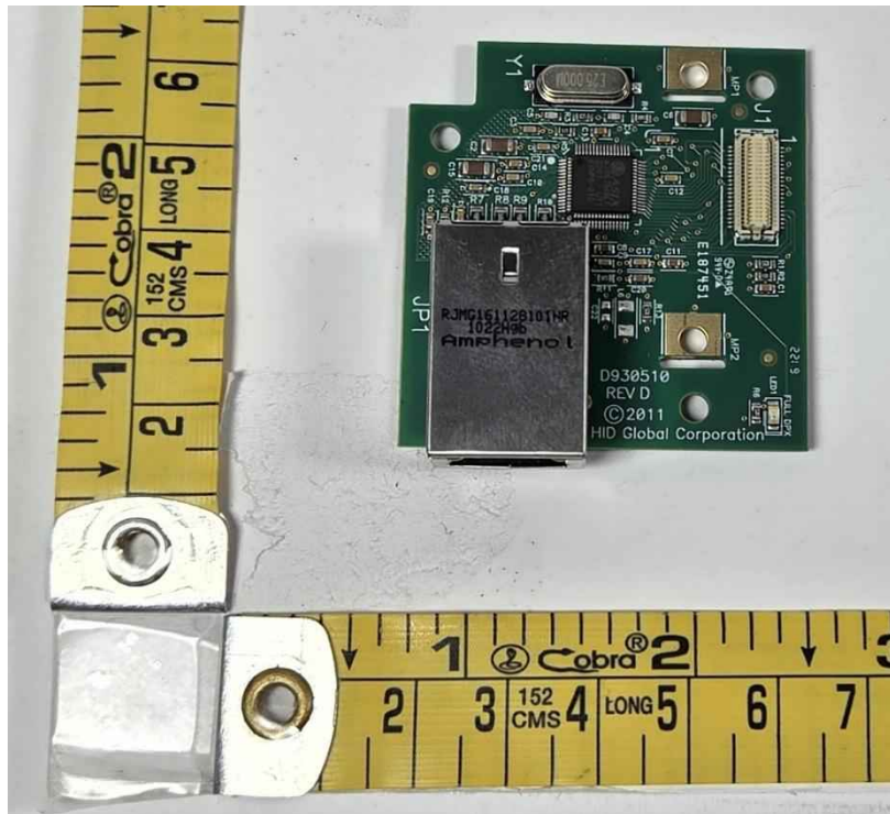
Ethernet Board_Top Side
