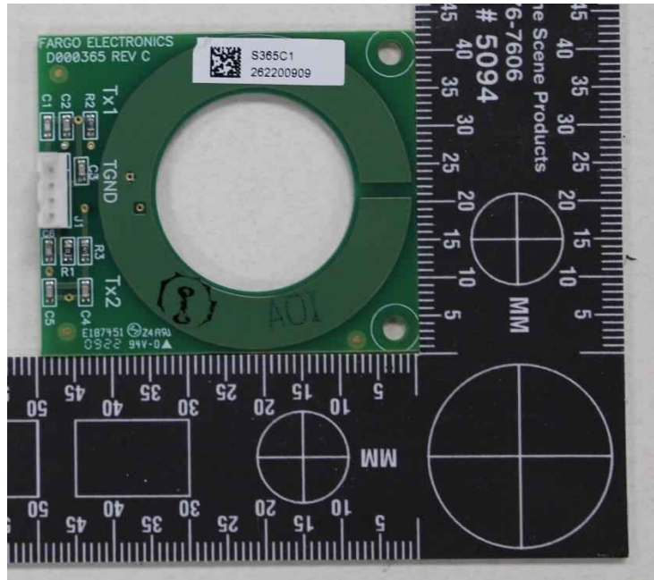
Laminator Upper and Lower RFID_PCB Antenna_Top Side
