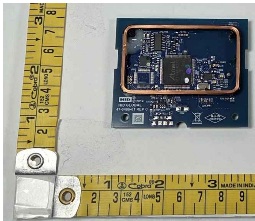
OMNIKEY 5127SI Encoder_Bottom Side
