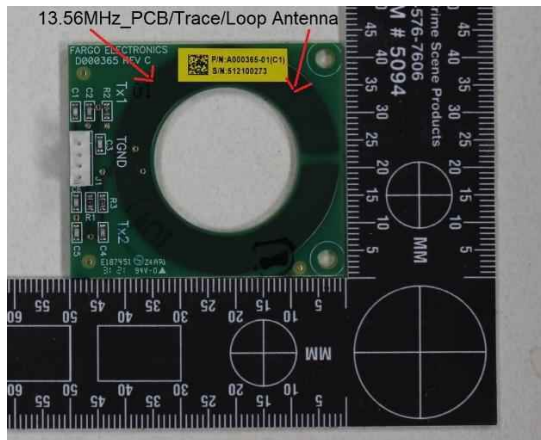
Ribbon RFID Antenna_Top Side
