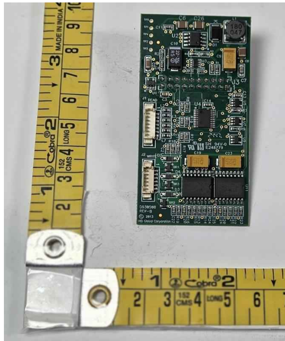
Mag Encoder Board_Top Side
