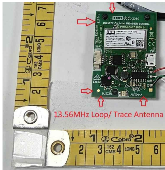
OMNIKEY 5127CK MINI_HF Antenna Location_Top Side
